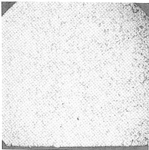
(a) Bare metal, picral etch. 25X.
