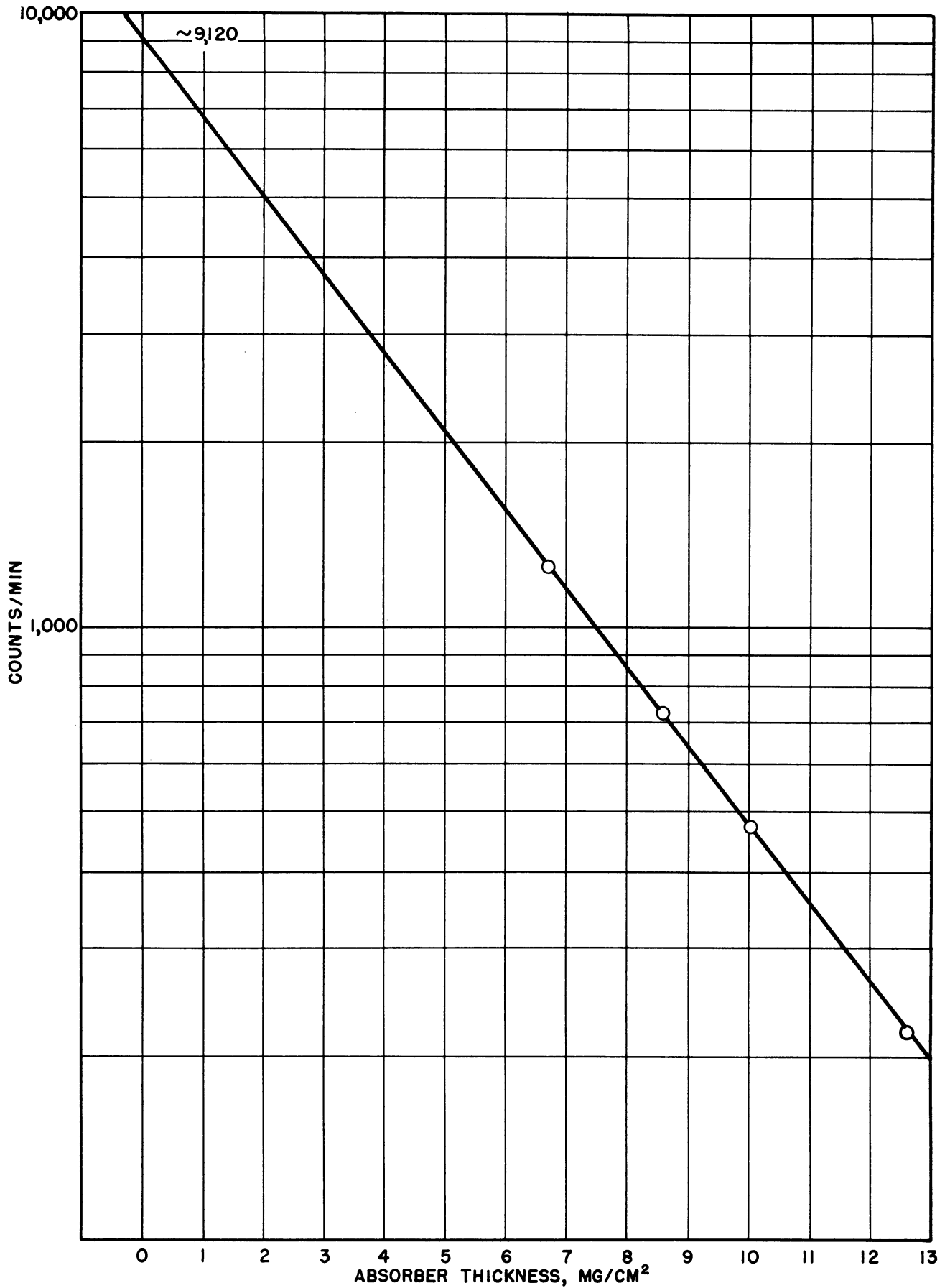
Figure 51.- Absorption curve for carbon-14.
