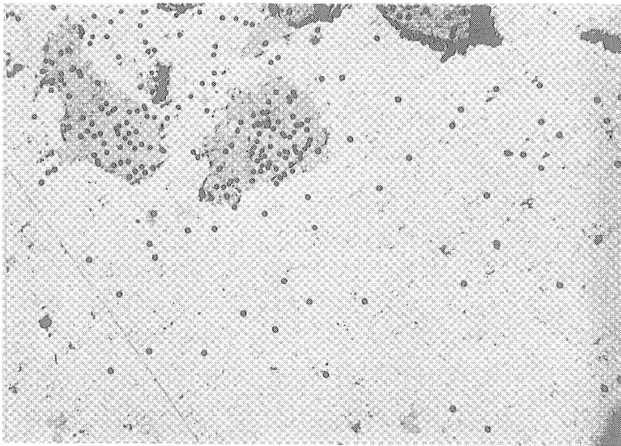
Figure 49.- Autoradiograph of nickel-silver mixture. Collodion type AX. 2.5-hour exposure. 250X.
