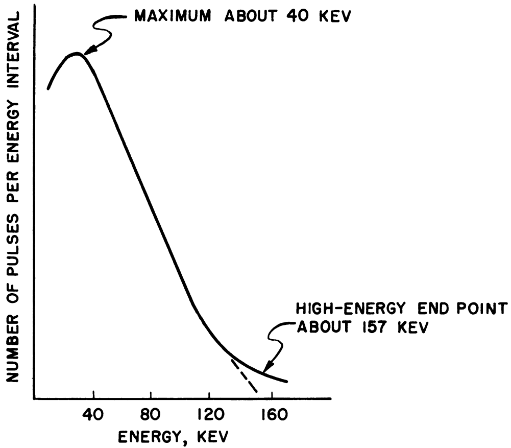
Figure 2.- Carbon-14 beta spectrum. (From ref. 101.)
