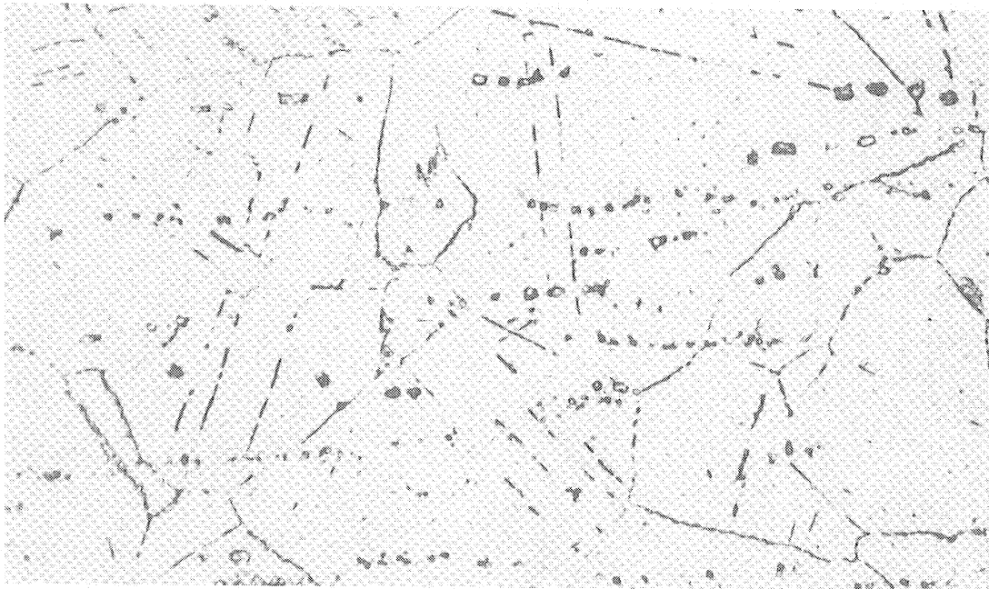
(b) Solution-treated at 2,200° F for 1 hour, water-quenched, heated at 1,400° F for 1,000 hours, and air-cooled. 1,000X.
