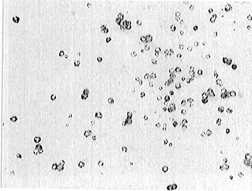
(c) Focus on silver grains. 1,000X.
