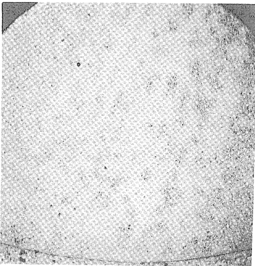
Figure 38.- Photomicrograph and autoradiograph of carbon-14 in steel. Sample coated with evaporated silver layer under autoradiograph. Collodion type AW. 1.3-hour exposure.
