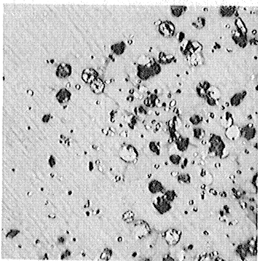
Figure 24.- Autoradiographs of carbon-14 in iron to show effects of different developers. Collodion type AW. 2.3-hour exposure.
