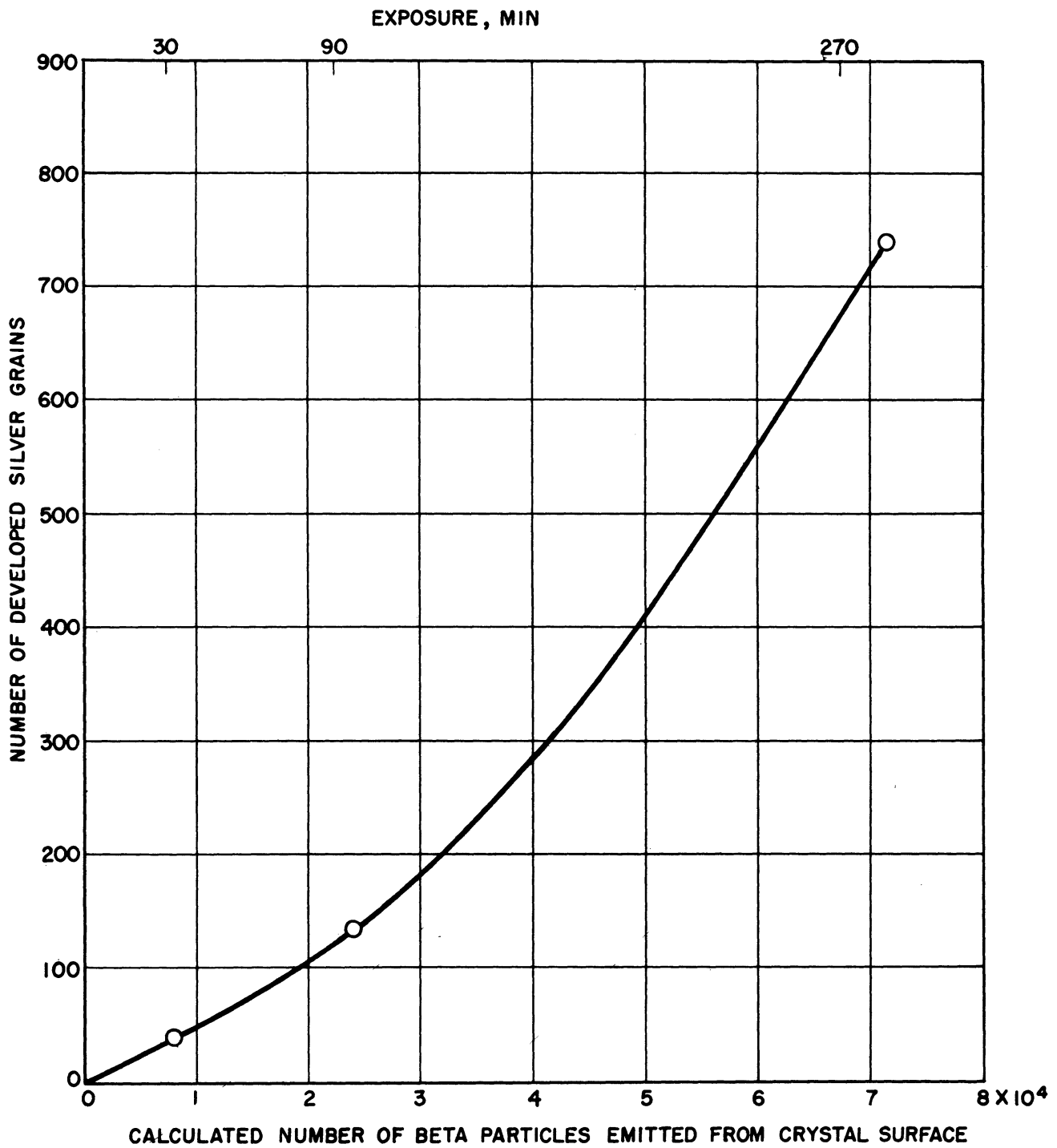
Figure 23.- Wet-autoradiography sensitivity curve.
