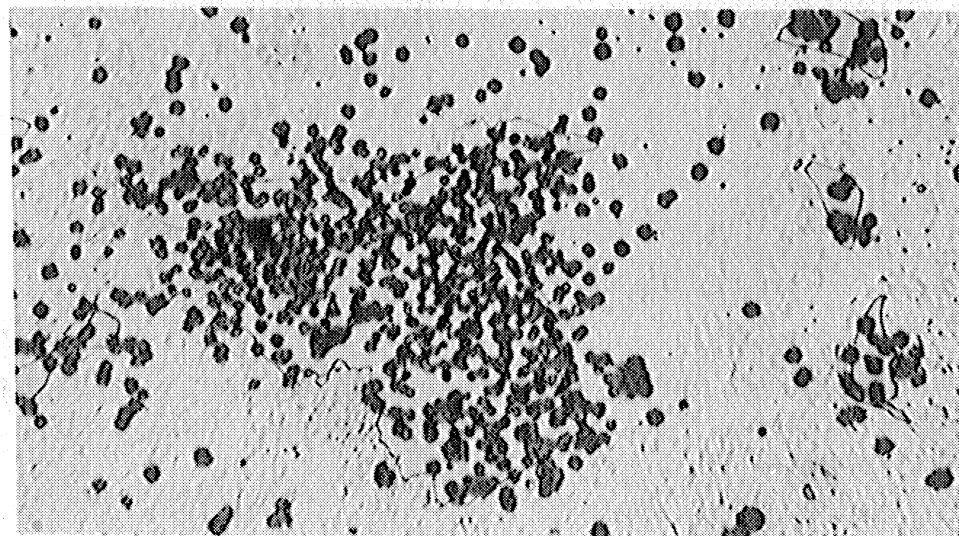
Figure 22.- Autoradiographs of the same cementite crystal at different exposure times. Collodion type AW.
