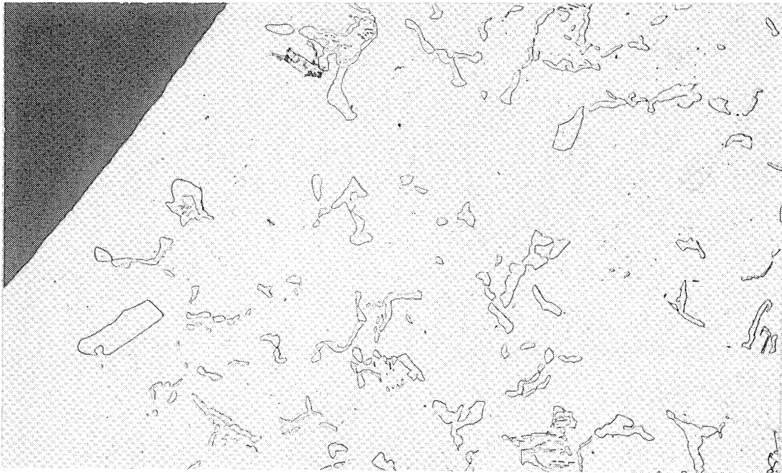
(a) Bare metal, picral etch. 250X.
