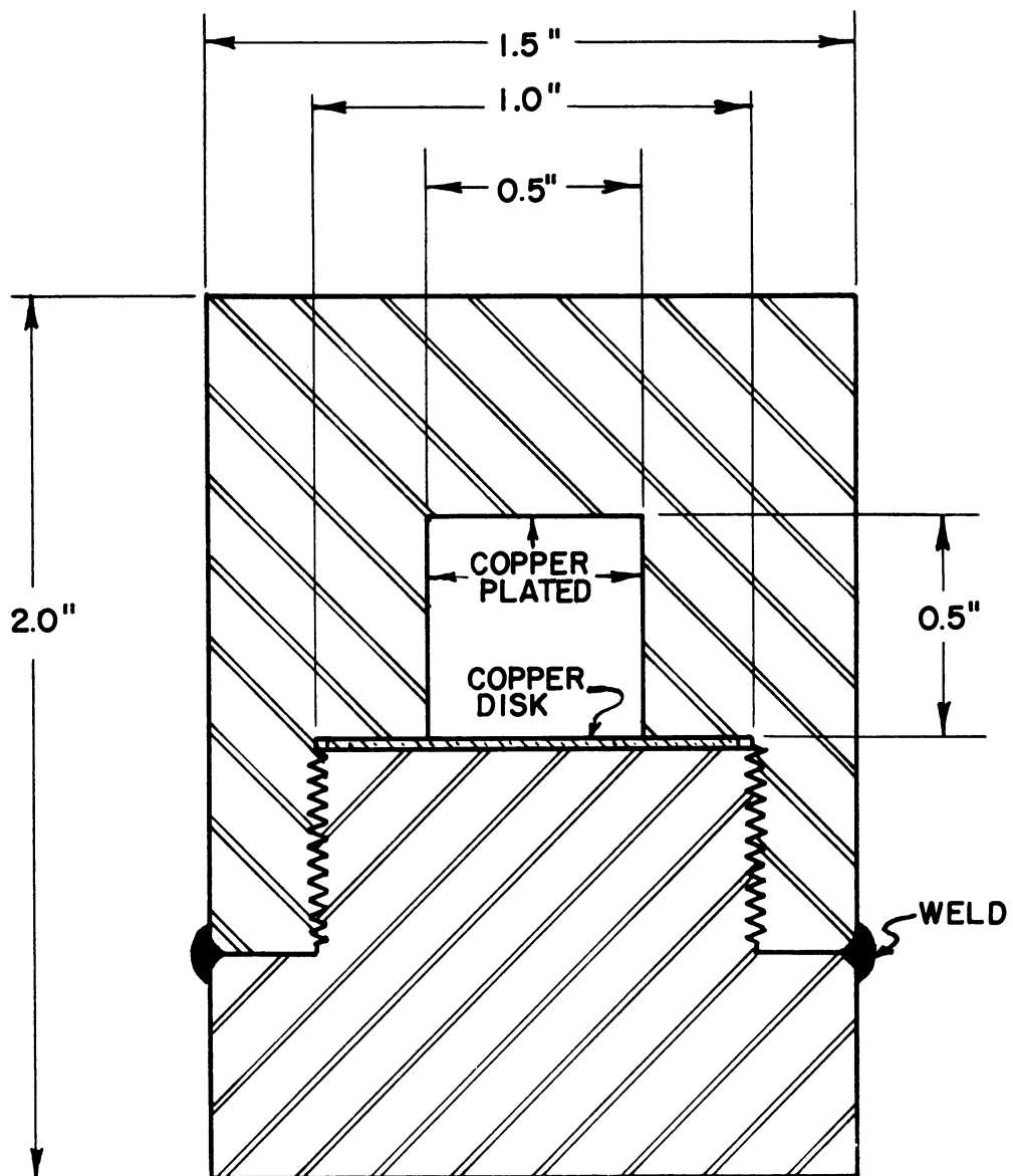
Figure 4.- Cylindrical steel carburizing capsule.
