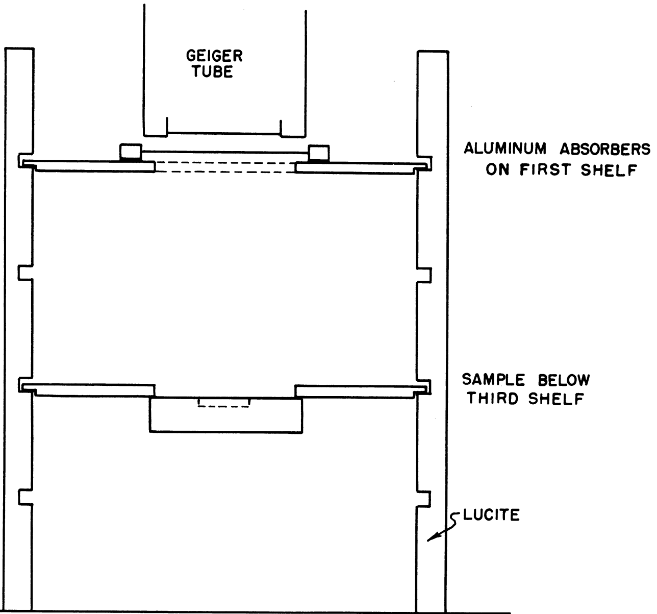
Figure 50.- Radioactivity counting rack.
