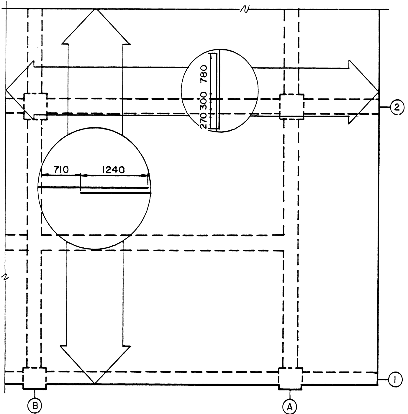
Fig. 4.19. Lap Splice Locations, Bottom Slab Bars, Floor Level Z2.
