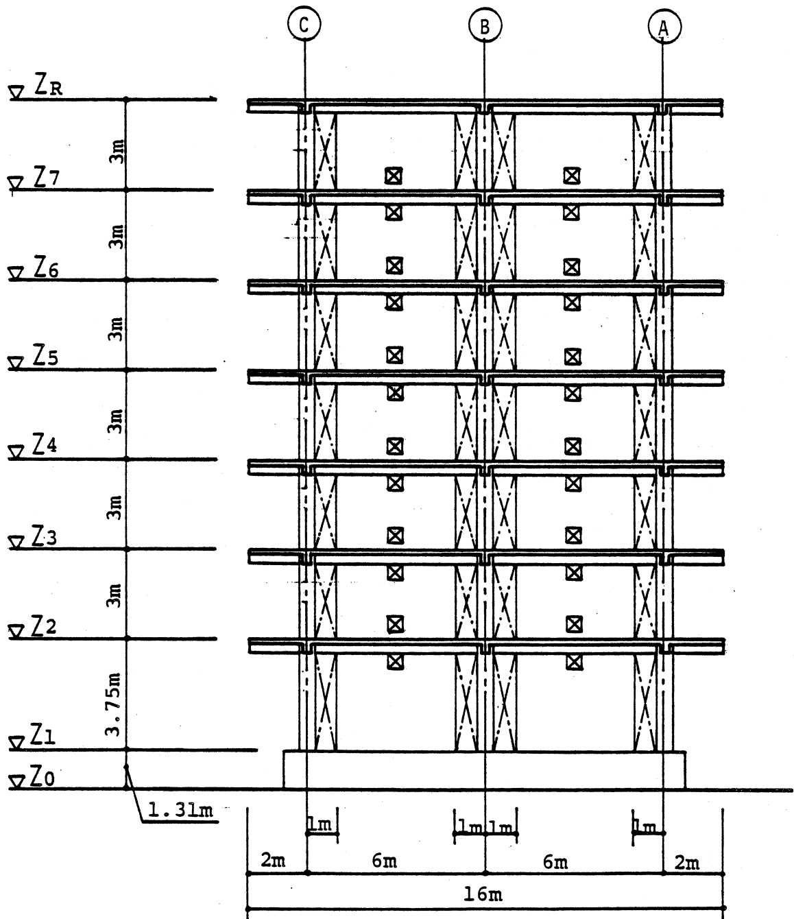
Fig.1.3. Elevation, Frame 4
