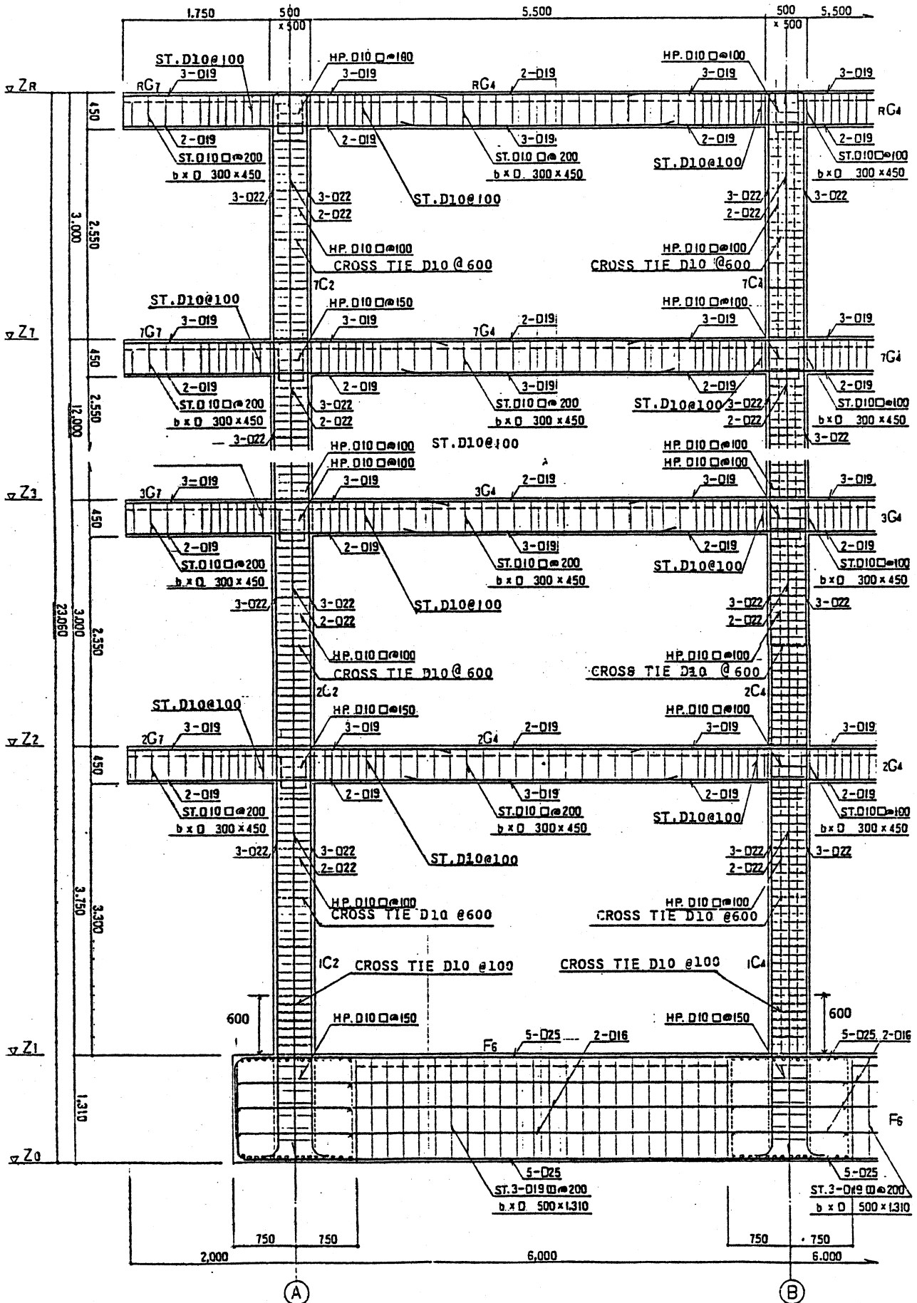
Fig. 4.4. Details of Reinforcing, Frames 2 and 3.
