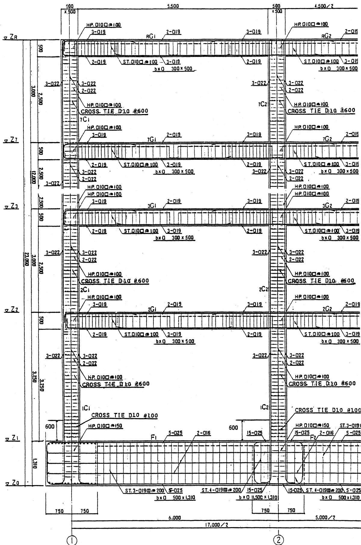
Fig. 4.1. Details of Reinforcing, Frames A and C.
