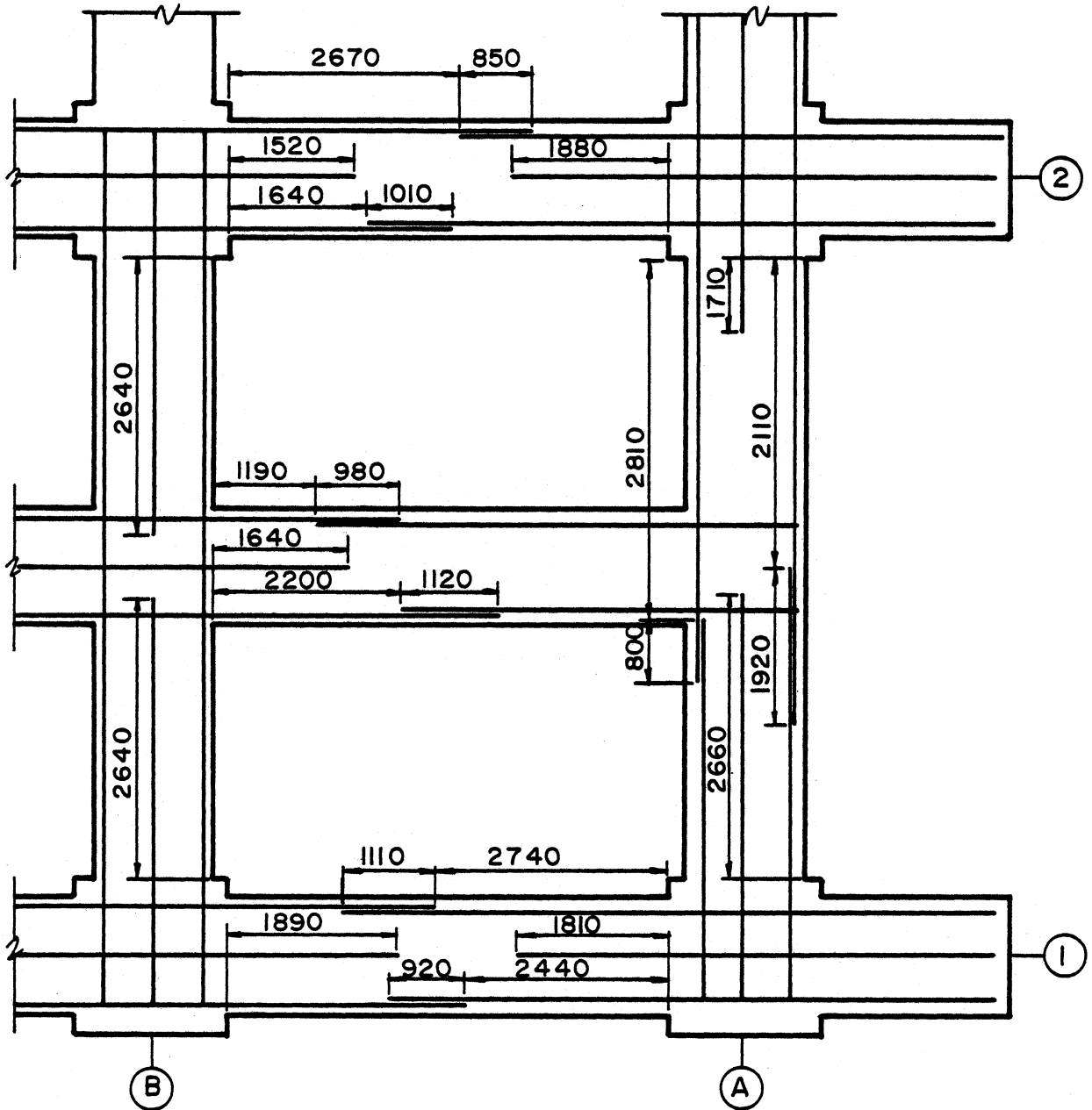
Fig. 4.16. Lap Splice Locations, Top Beam Bars, Floor Level Z4.
