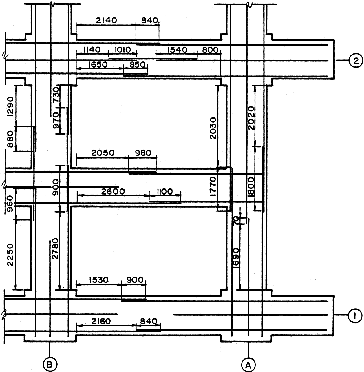
Fig. 4.14. Lap Splice Locations, Top Beam Bars, Floor Level Z2.
