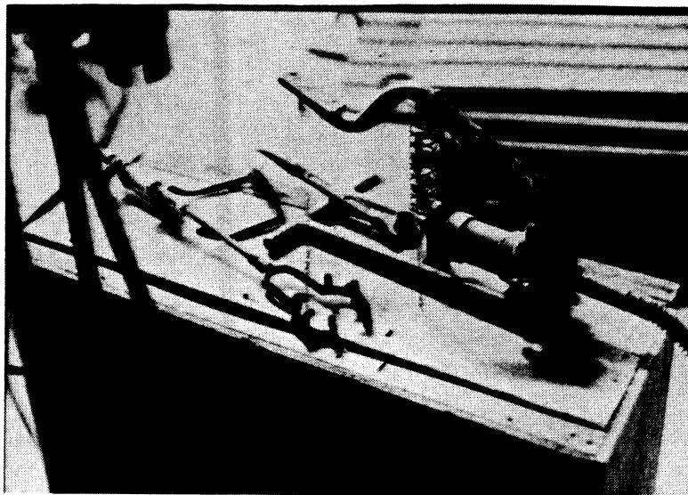
Fig. 2.2. Equipment for Gas Pressure Welding.
