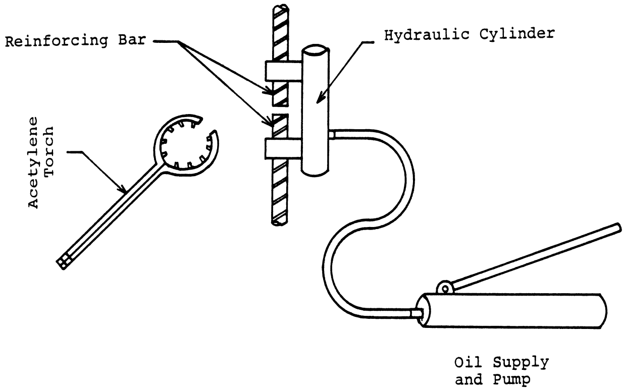
Fig. 2.1. Gas Pressure Welding Process.
