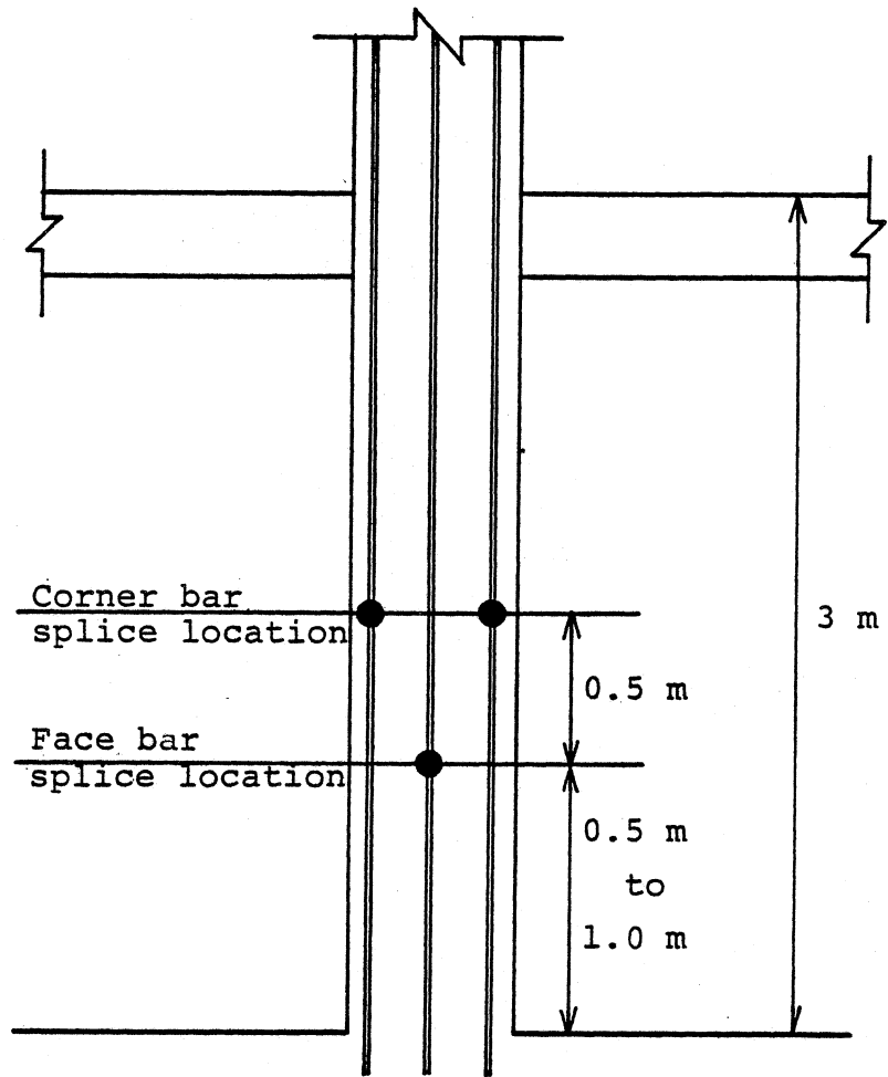
Fig. 4.13. Location of Column Rebar Splices.
