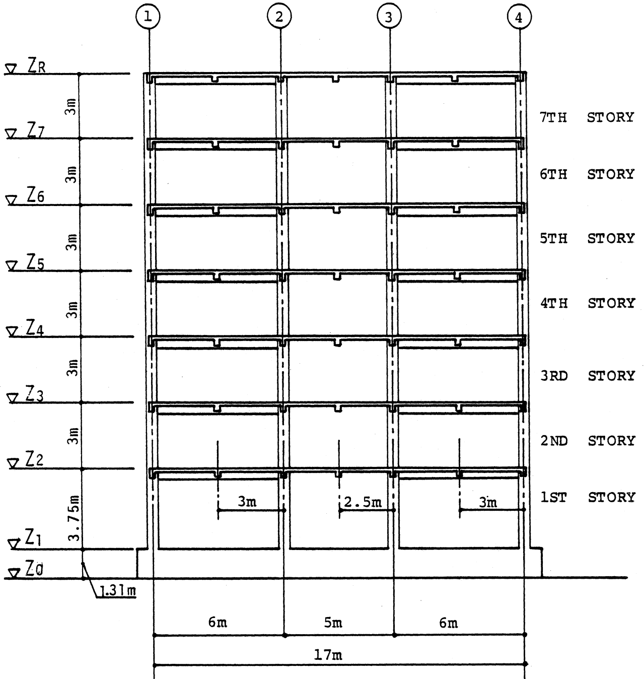
Fig.1.2. Elevation, Frame B
