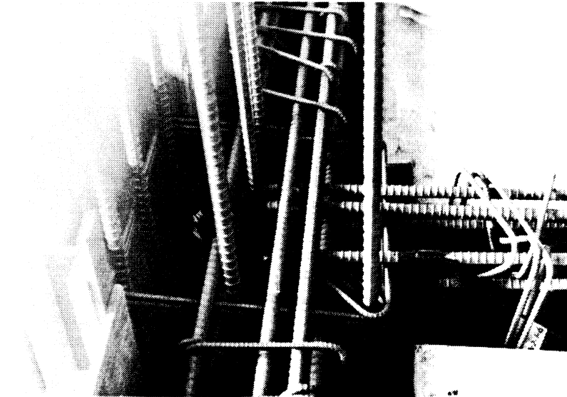
Fig. 4.22. Bars Anchored Near Column Center-line.
