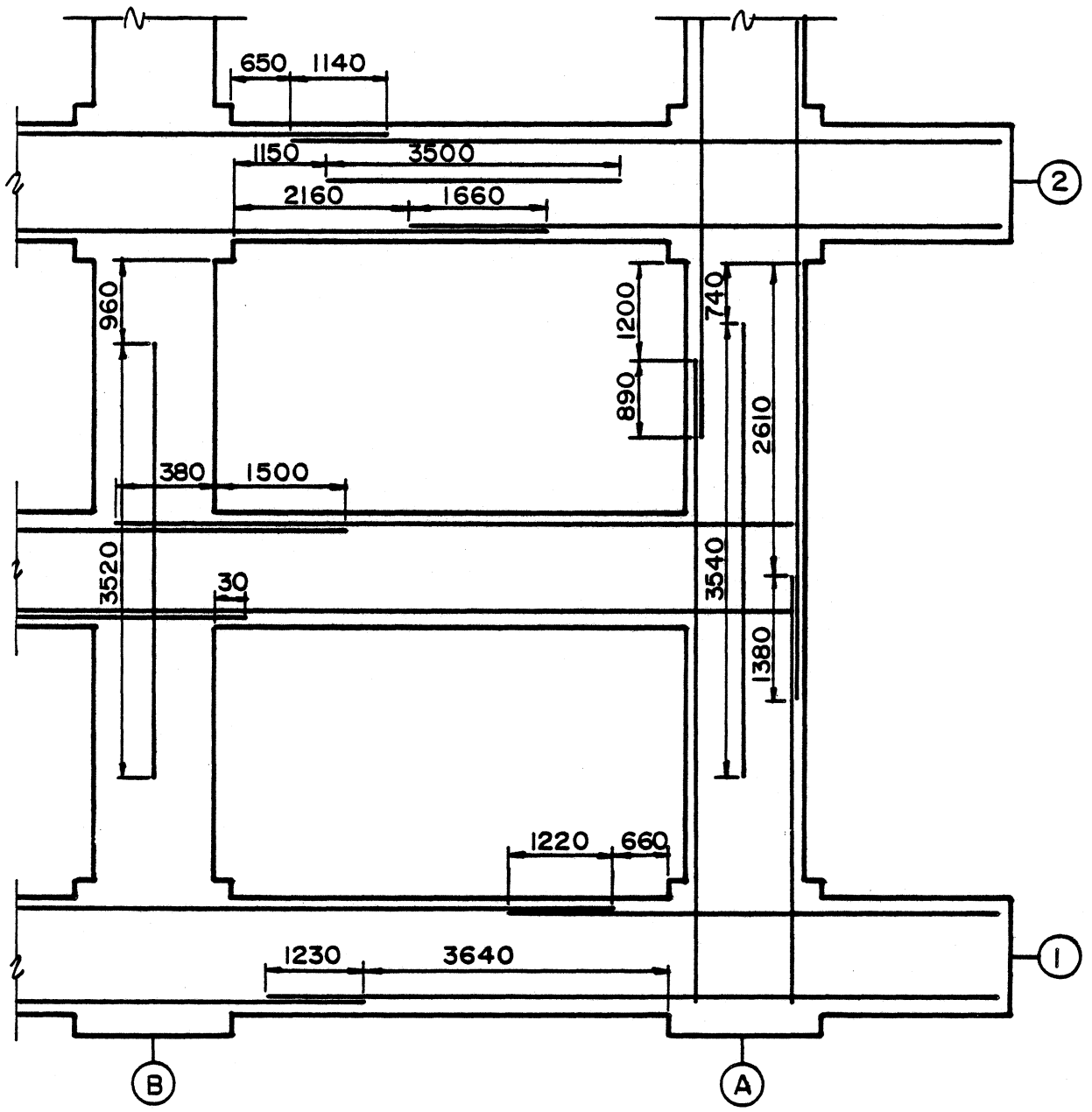
Fig. 4.17. Lap Splice Locations, Bottom Beam Bars, Floor Level Z4.
