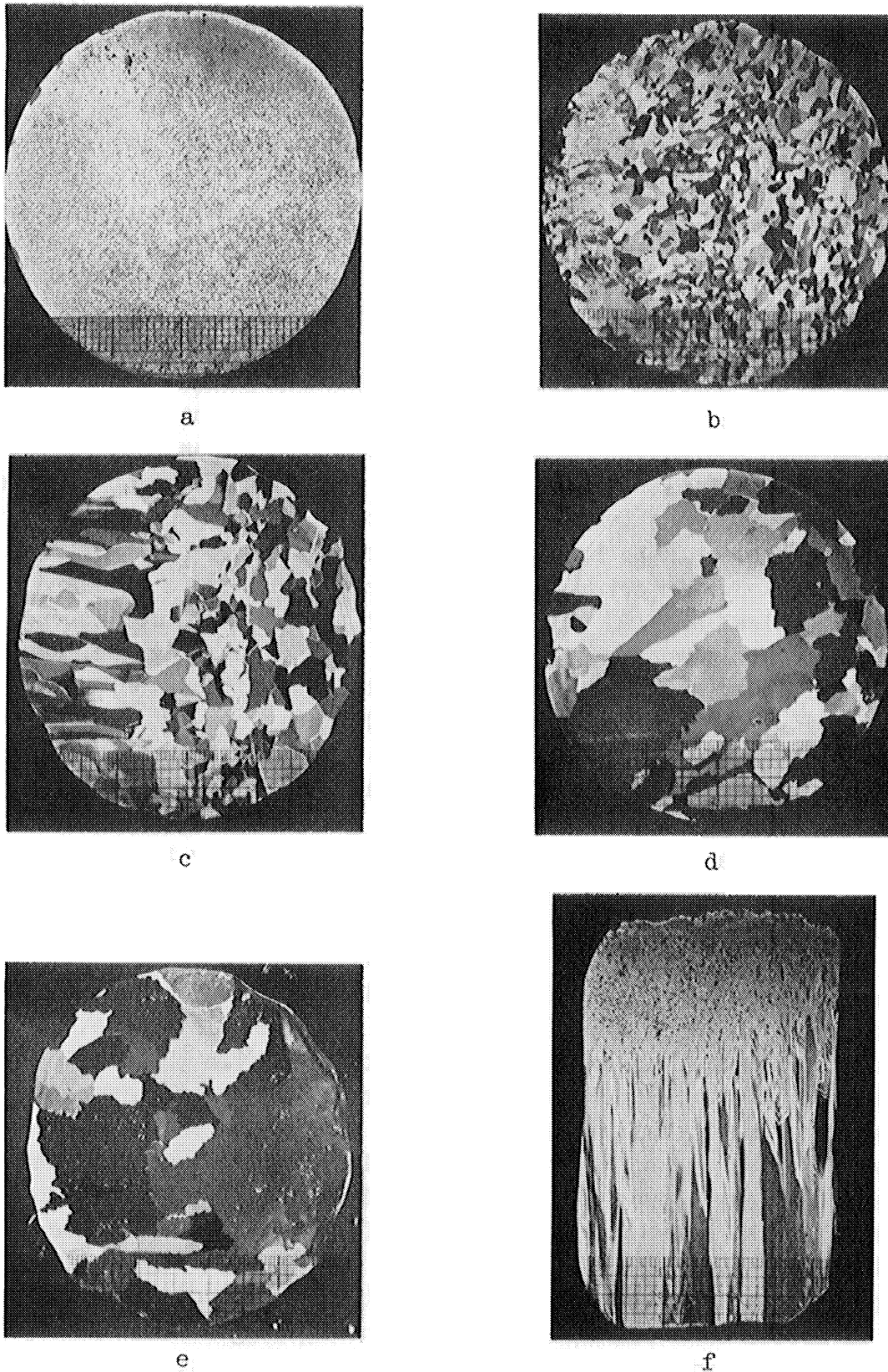
Figure 17. Photographs of thin sections of ice between crossed polaroids. Sections were 1/4 inch thick. a to e are successive sections at 4-inch intervals starting 3 inches from the top of a 17-inch core from Duncan Bay, Cheboygan, Michigan. f is a vertical section of sheet ice. The squares on the scale are 1/10 inch.
