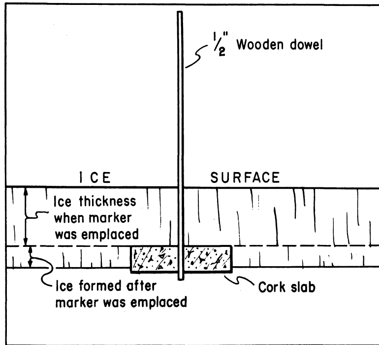
Figure 39. Drawing of cork slab marker.
