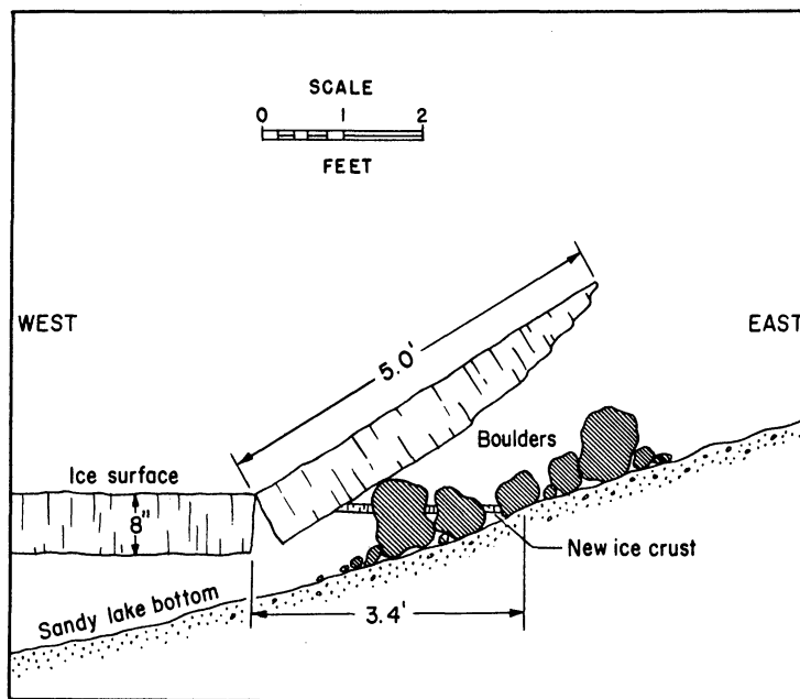
Figure 43. Drawing showing relation between ice push and the upturned ice edge.
