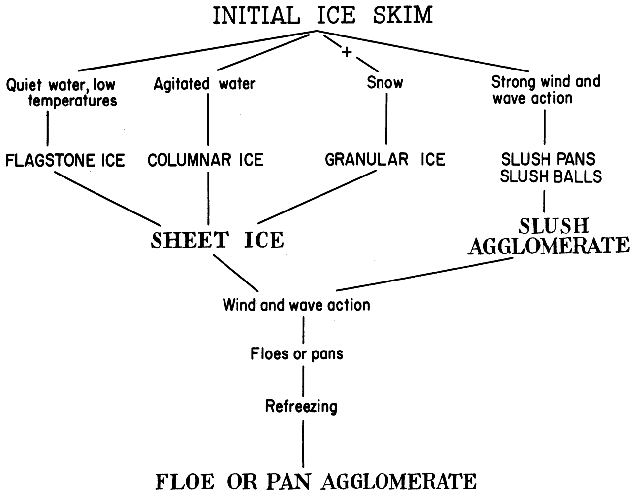
Figure 25. Classification of ice covers.
