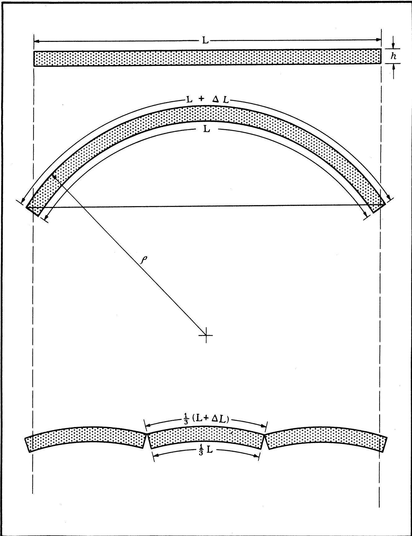
Figure 51. Schematic drawing of the ice push process.
