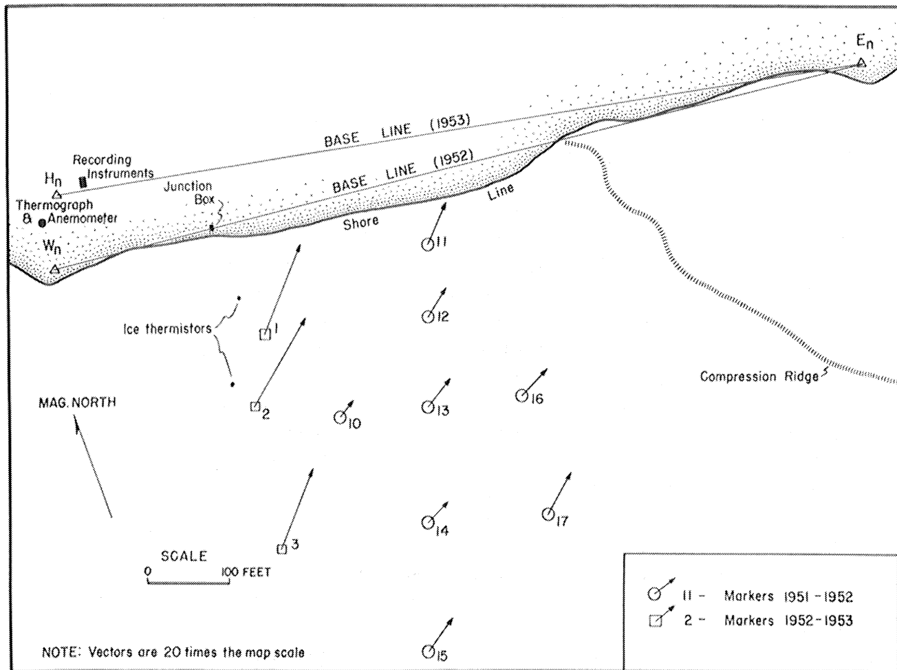
Figure 37. Map of the ice push study area.
