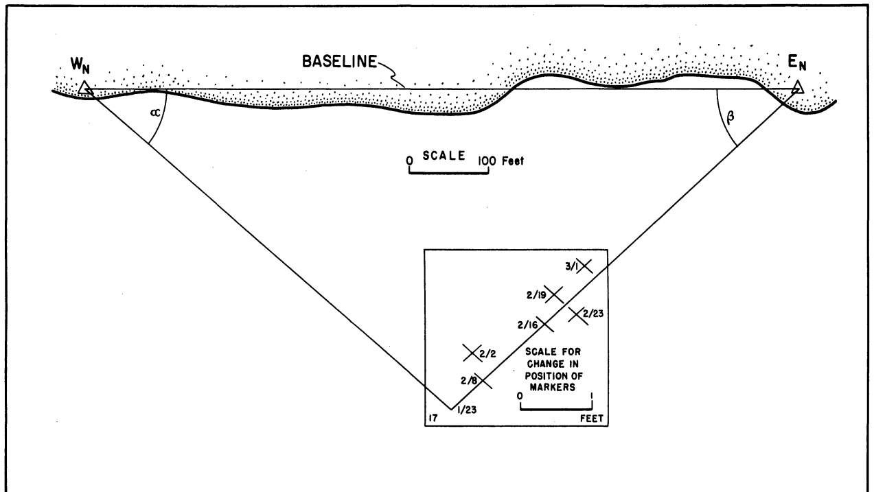
Figure 40. Drawing to show the movement of a marker as determined by angle measurements from the shore.
