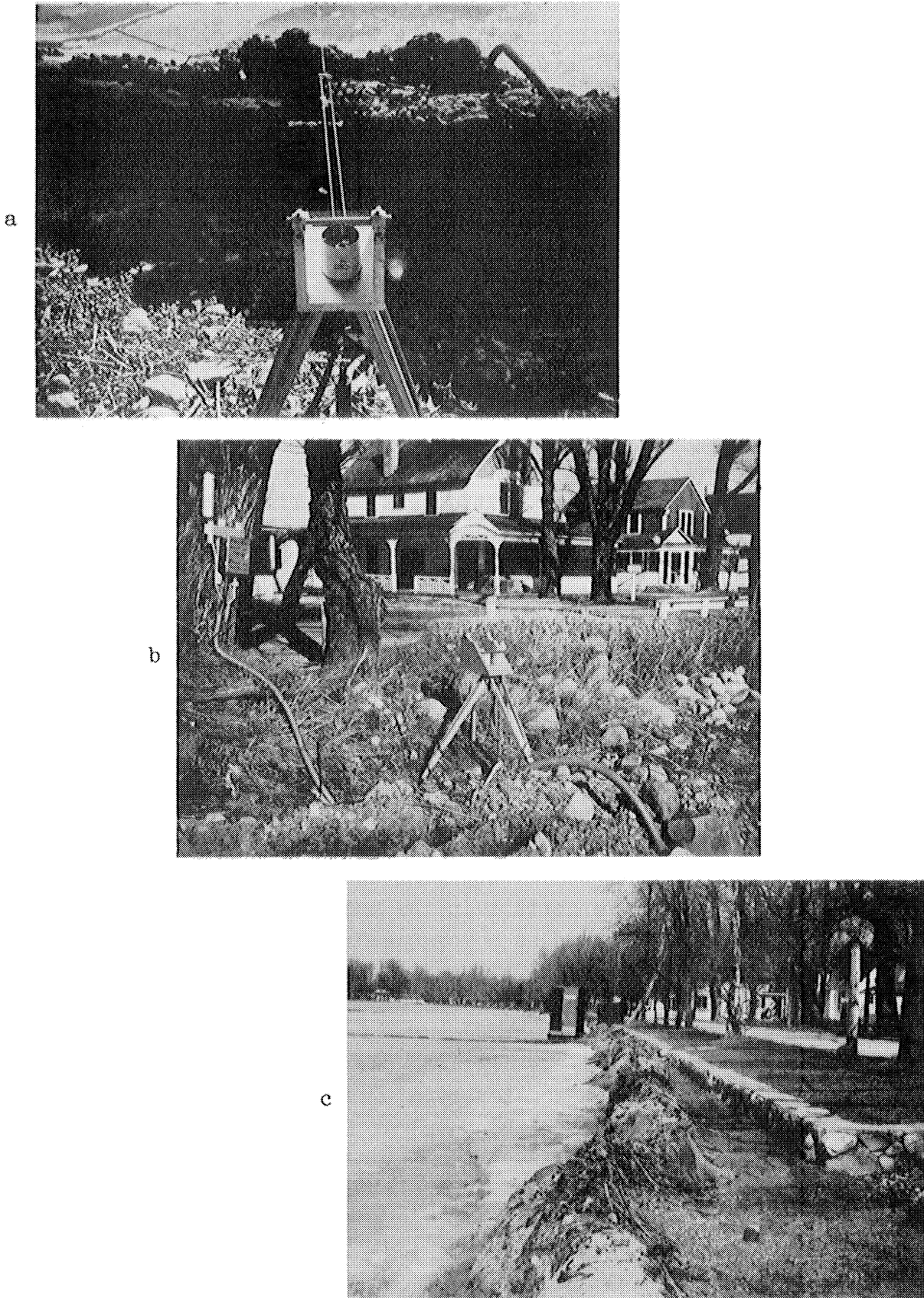
Figure 46. New ice ramparts formed during the winter of 1952-53. Note the effect of the low lake level at this time.
