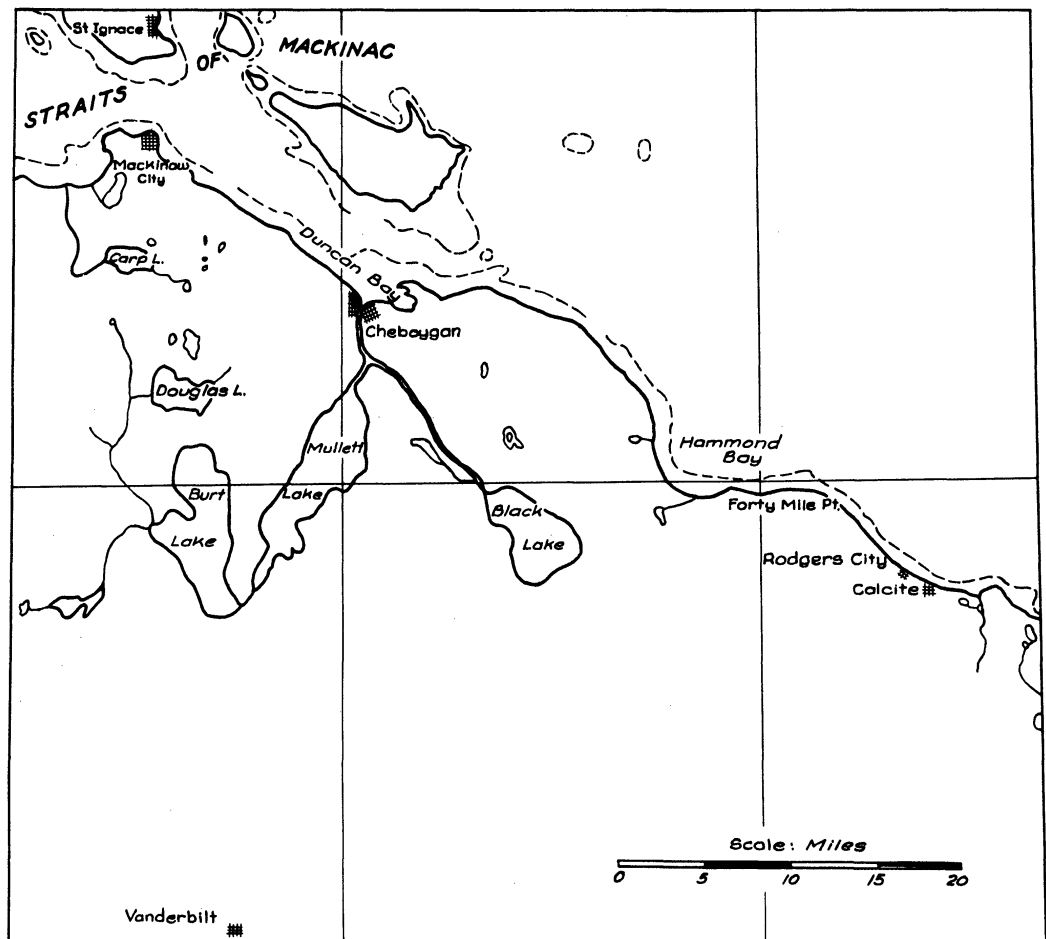
Figure 5. Index map of the Rogers City—Cheboygan area.
