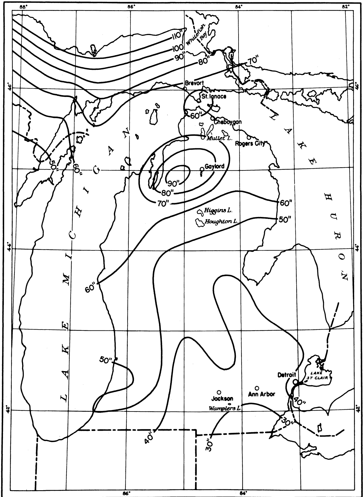
Figure 3. Average annual snowfall in Michigan.
