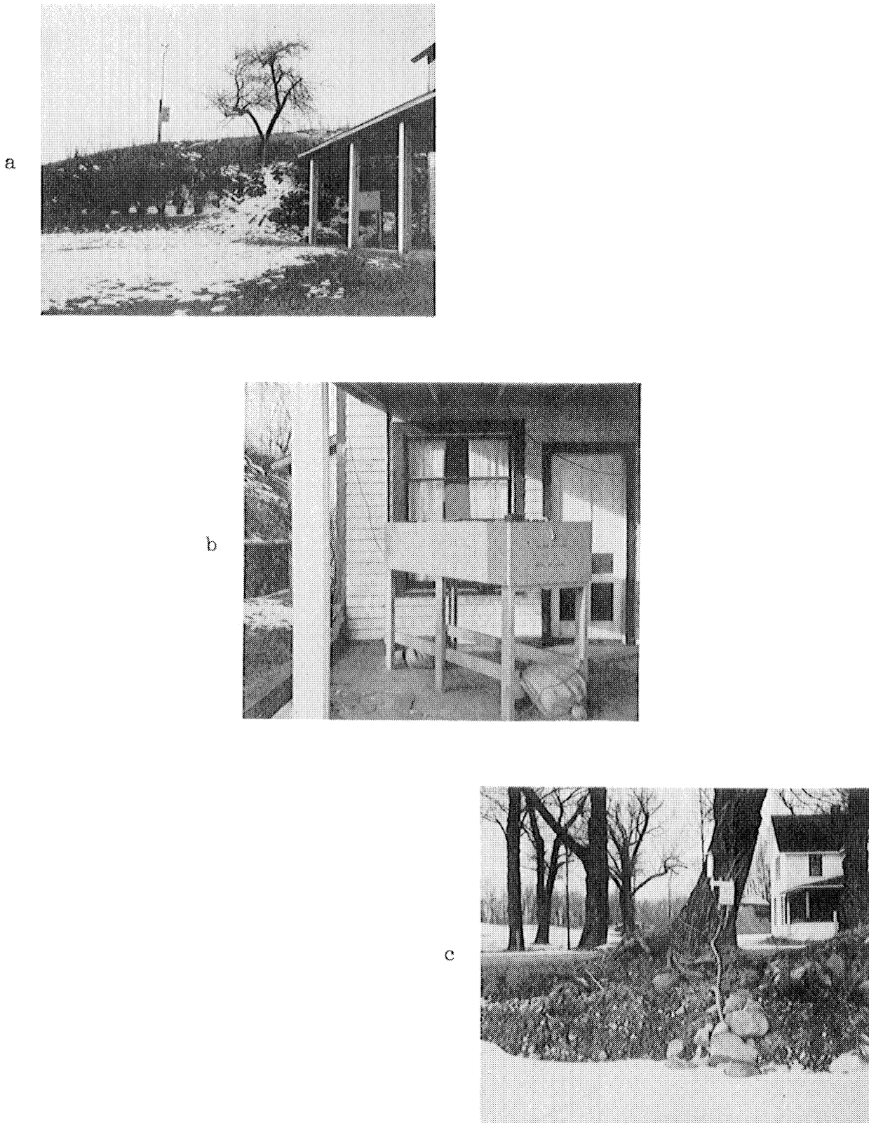
Figure 47. Photographs of the temperature recording installation on the north shore of Wamplers Lake, Winter of 1952-53. a. anemometer and recorder locations. b. Recorder house. c. Junction box, air thermostat housing and shore end of cables.
