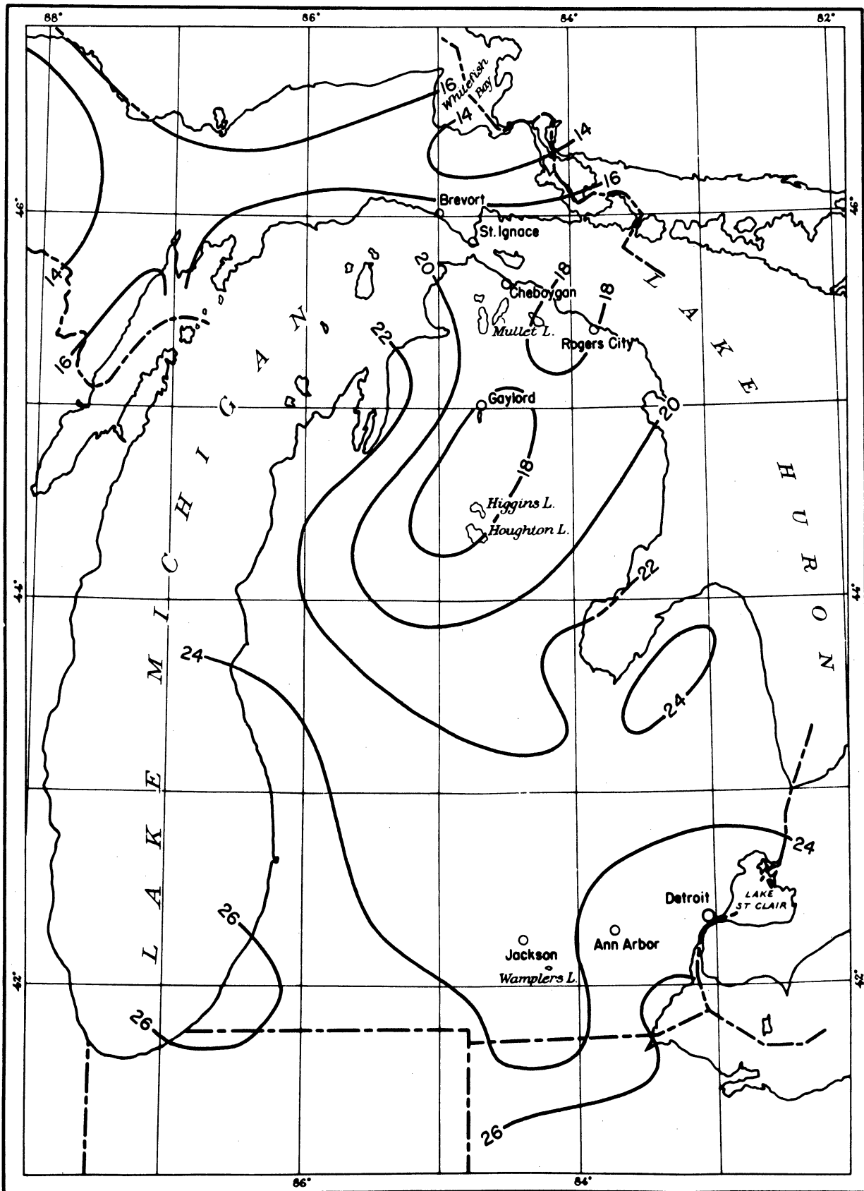
Figure 2. Average January temperatures in Michigan.
