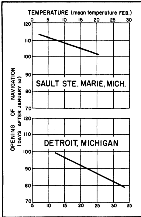
Figure 4. Date of opening of navigation as a function of the February temperature.
