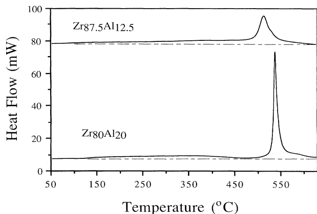
FIG. 3. DSC traces, taken at 20°C/min, for 24-h milled Zr_{87.5}Al_{12.5} and Zr_{80}Al_{20} powders. The narrow exothermic peak corresponds to transformation to equilibrium. The exothermic signal starts at temperatures as low as about 120°C.
