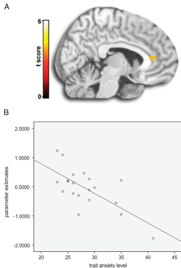
Figure 1. (A) Whole-brain anterior cingulate activation (peak voxel at -6, 36, 9 ) from negative regression of trait anxiety level for [(Attend Face angry - Attend Face neutral ) - (Attend Scene angry - Attend Scene neutral )]. (B) Illustrative scatter plot of trait anxiety level and anterior cingulate activation ( \beta weights) extracted from a 5-mm radius volume of interest centered at the peak ( -6, 36, 9 ).
