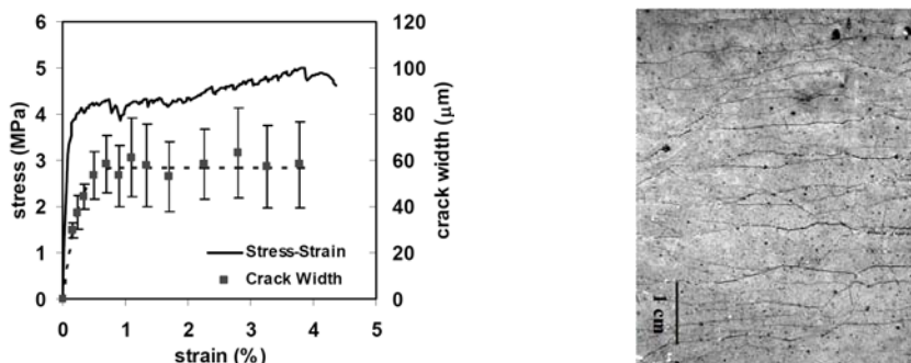
Figure 1: Typical direct tension stress-strain behavior of ECC and microcrack pattern
