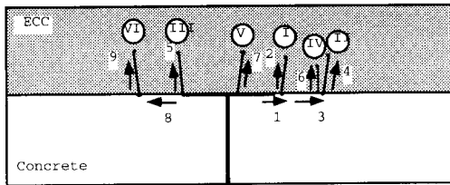
(a) Sequence of kinked crack development
