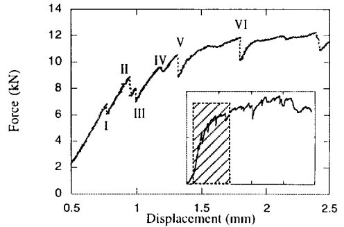
(b) Load-deflection with kinked sequence
