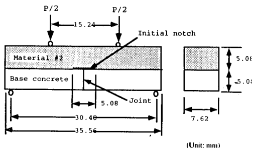
Figure 3: Loading configuration and dimensions of designed specimen
