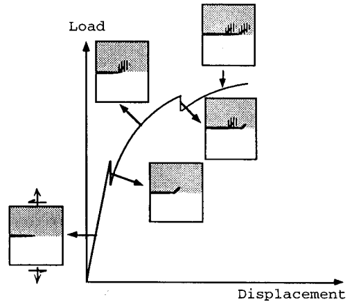
Figure 2: Trapping mechanism in a bimaterial interface system
