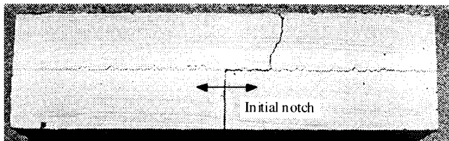
(b) Concrete/Concrete system (reassembled after test)
