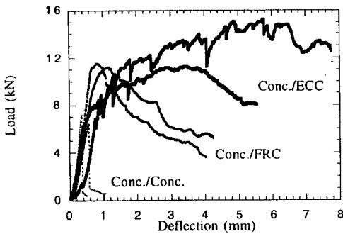
Figure 6: Load-deflection behavior in different bimaterial system
