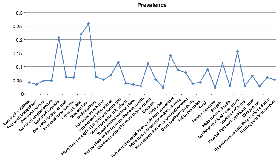
Fig. 1. Lifetime prevalence of 34 externalizing behaviors (N = 43, 093).
