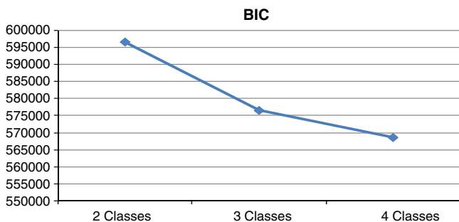
Fig. 2. BIC values across latent classes.
