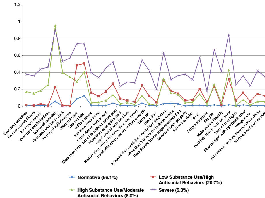
Fig. 6. Lifetime prevalences of 34 externalizing behaviors across 4 latent classes.
