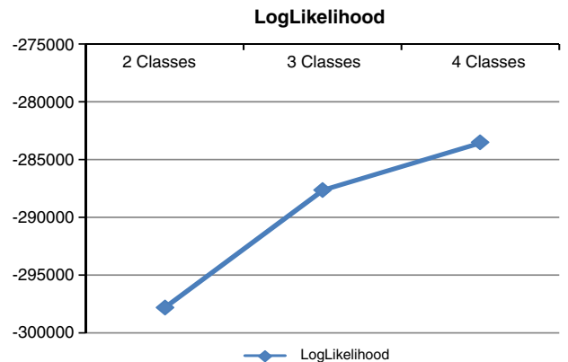
Fig. 4. Trends in log-likelihood values across latent classes.
