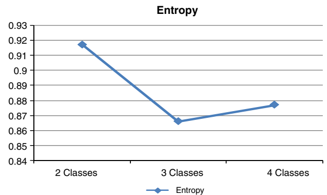
Fig. 3. Entropy values across latent classes.
