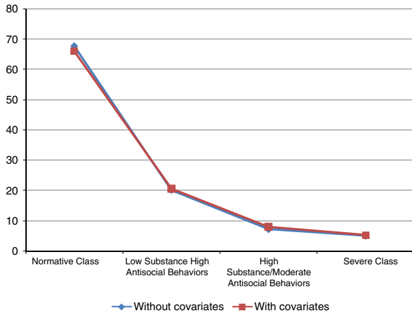
Fig. 5. Probability of four latent classes with and without covariates.
