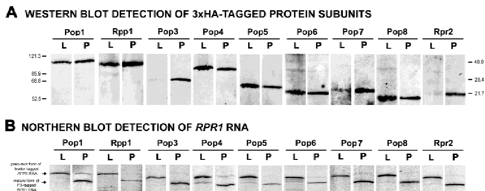
FIGURE 3. The protein subunit composition of pre-RNase P and mature RNase P. Crude extracts from yeast strains containing 3×HA-tagged protein subunits and either the leader- or P3-tagged RPR1 were incubated with Sephadex, after which the beads were washed and eluted with dextran. The eluates were analyzed for the presence of protein subunits and RPR1 RNA by western (A) and northern blot analysis (B), respectively. Pre- RPR1 and mostly mature RPR1 are specifically isolated, respectively, from the strains containing the leader-tagged (L) or P3-tagged RPR1 (P) constructs as shown in B. (The small-sized bands found in the eluates of some leader-tagged RPR1 strains are not the correct sizes for mature RPR1 and are likely to be partial degradation products of pre- RPR1 that occur during isolation.) From the western analysis (A), the protein subunit composition of pre-RNase P is similar to that of mature RNase P, except that Pop3p and Rpr2p are nearly absent. The protein samples were analyzed on either 7.5% (Pop1p) or 12% SDS-PAGE (the other protein subunits). The molecular weight markers for both gels are shown at the left and right in A. Some protein subunits, that is, Rpp1p and Pop7p, migrate as proteins with molecular weight larger than predicted by sequence.
