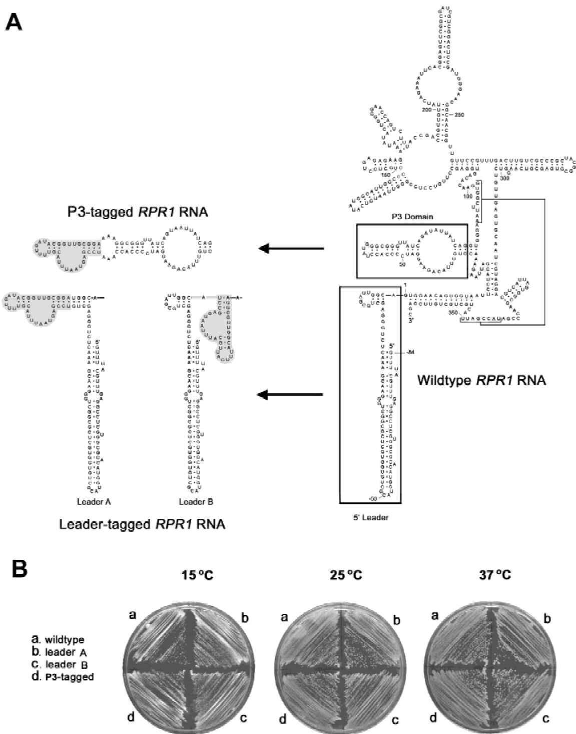
FIGURE 1. Affinity tagging of RPR1 RNA with Sephadex-binding RNA ligand. A: The secondary structure of RPR1 RNA according to Frank et al. (2000) is shown with the sequence of mature RPR1 RNA starting at the nucleotide position +1. The predicted structures of the 5' leader (from -1 to -84) and the P3 domain are shown in rectangles. The minimal binding motif of Sephadex-binding RNAs (in shaded areas) are inserted into the 5' leader and the end of P3 domain to generate the leader-tagged (A and B) and P3-tagged RPR1 RNA, respectively. B: Growth phenotypes of the yeast strains containing either wild-type, leader-tagged (A or B), or P3-tagged RPR1 at various temperatures (15, 25, and 37 °C). The strains containing tagged RPR1 have growth phenotypes indistinguishable from that of the wild-type strain.
