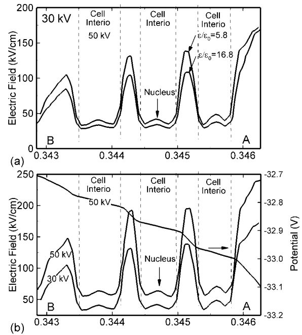
Figure 13. Electric fields for different operating parameters and cell properties. (a) Electric fields for membrane dielectric constants of 5.8 and 16.8 and (b) electric fields for –30 and –50 kV on the applicator. The increase in dielectric constant by a factor of 3 results in a decrease in electric field across the membranes by 40%. The increase in applied voltage by a factor of 1.66 results in a commensurate increase in electric field.
