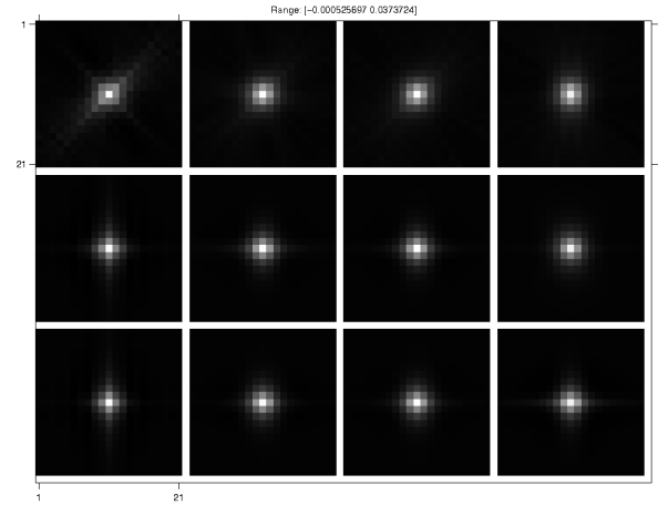
Fig. 2. xy, xz, and yz (top to bottom) slices of PSFs created using our proposed regularization at (25,25,0), (15,15,0), (15,15,15), and (25,0,0) (left to right).
