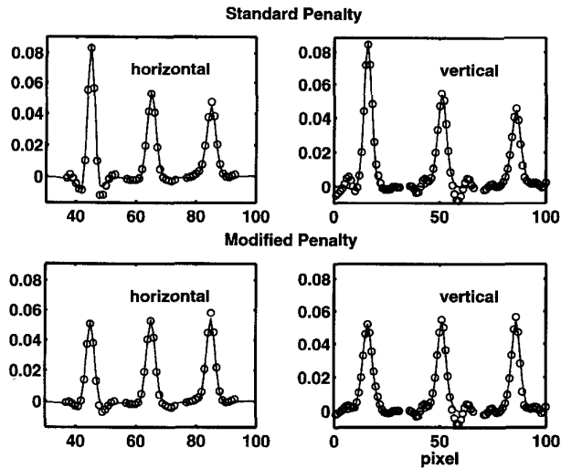
Fig. 4. Horizontal and vertical profiles (concatenated left to right) through three local impulse response functions for a penalized-likelihood estimate of the image shown in Fig. 3. The standard quadratic penalty yields highly nonuniform resolution (upper profiles), whereas the proposed modified penalty leads to nearly uniform spatial resolution (lower profiles). Note that for the standard penalty the resolution is poorest in the high-count (rightmost) disk.
