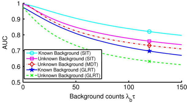
Fig. 6. AUC versus \lambda_b \tau for spatially uniform background of known and unknown intensity background where \mu r = 10 and \alpha \tau = 10 .
