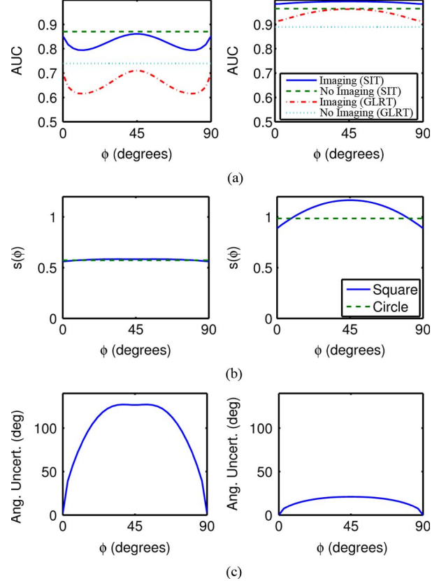
Fig. 5. AUC, relative sensitivity, and angular uncertainty for square position-sensitive and circular counting detectors of equal area ( r = 2l/\sqrt{\pi} ) versus \phi with \mu l = 0.5 (left) and \mu l = 5 (right), and \alpha \tau = \lambda_b \tau = 10 . (a) AUC versus \phi ; (b) s(\phi) versus \phi ; and (c) angular uncertainty versus \phi .
