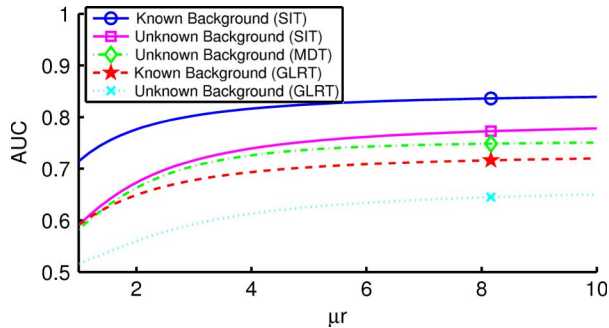
Fig. 7. AUC for spatially uniform background of known and unknown intensity versus attenuation-radius product for \alpha \tau = 10 , \lambda_b \tau = 100 .
