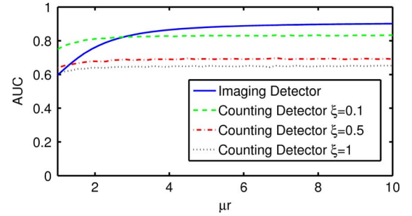
Fig. 8. AUC versus \mu r for position-sensitive and counting detectors, where the counting detector uses a "guessed" background rate in the "known background" GLRT. \alpha \tau = \lambda_b \tau = 10 .
