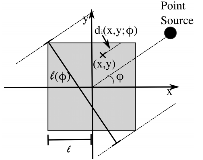
Fig. 2. Diagram of square detector with side length 2l .
