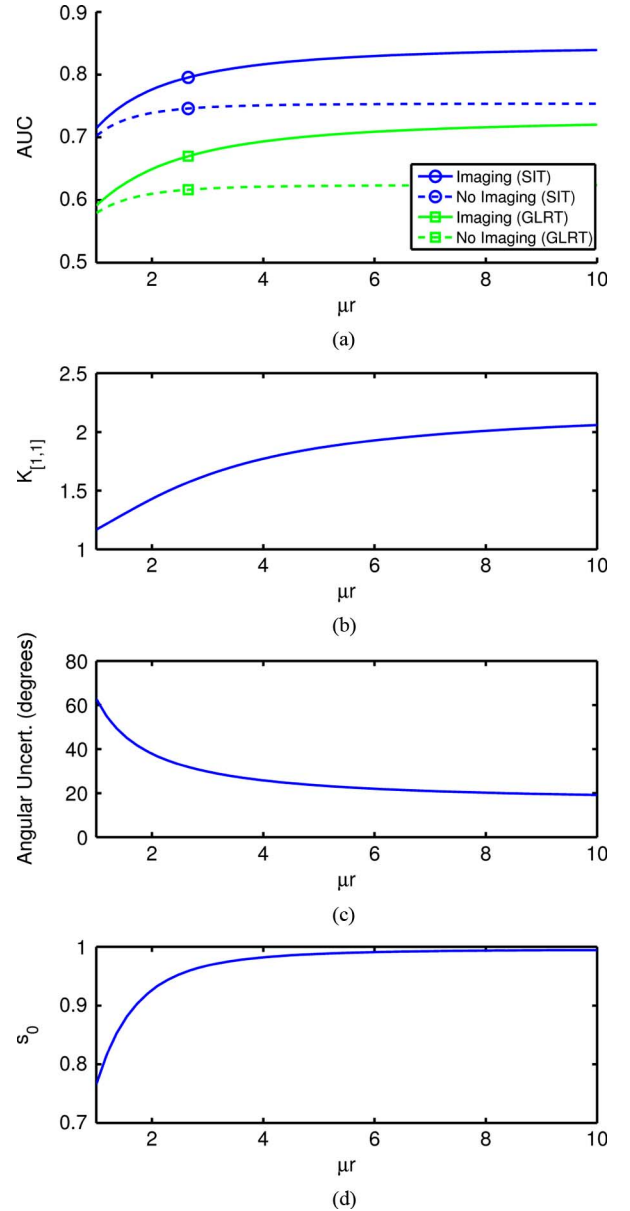
Fig. 3. Various quantities for a circular uniform-sensitivity detector with \alpha\tau = 10 , \lambda_b\tau = 100 , and geometric sensitivity p(G|\phi) = 1 . (a) AUC versus \mu r ; (b) K_{[1,1]} versus \mu r ; (c) angular uncertainty versus \mu r ; and (d) s_0 versus \mu r .
