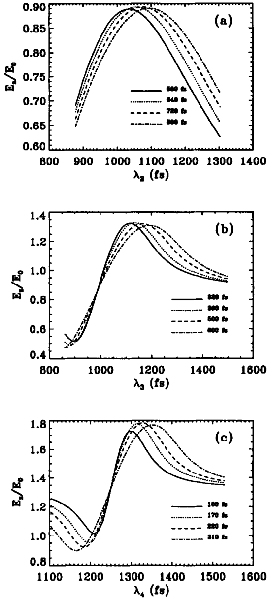
FIG. 9. The maximum electric field \hat{E}_{\max,n} produced by varying both the pulse widths \tau and interpulse spacings \lambda_{N,n} , for the second n = 2 (a), third n = 3 (b), and fourth n = 4 (c) pulses. Note the change in scaling of \hat{E}_{\max} for the three plots.
