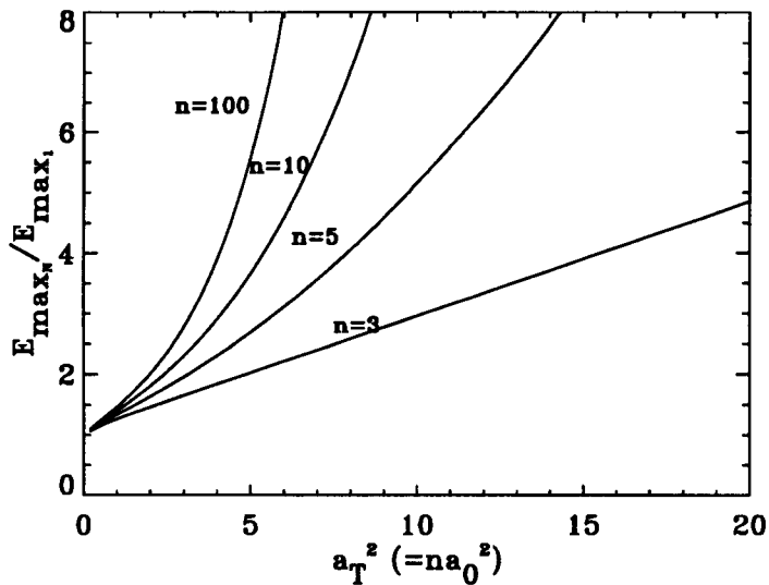
FIG. 2. The ratio of the maximum field achieved with a train of pulses ( \hat{E}_{\max_n} ) over that achieved with a single pulse ( \hat{E}_{\max_1} ) of the same energy versus the quantity a_T^2 = n a_0^2 for n = 3, 5, 10 and 100 .
