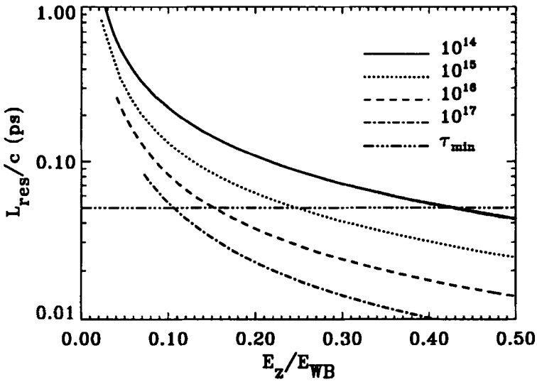
FIG. 7. Plot of L_{res}/c vs \epsilon for various densities. Finite rise-time effects are important for L_{res}/c < \tau_{min} .
