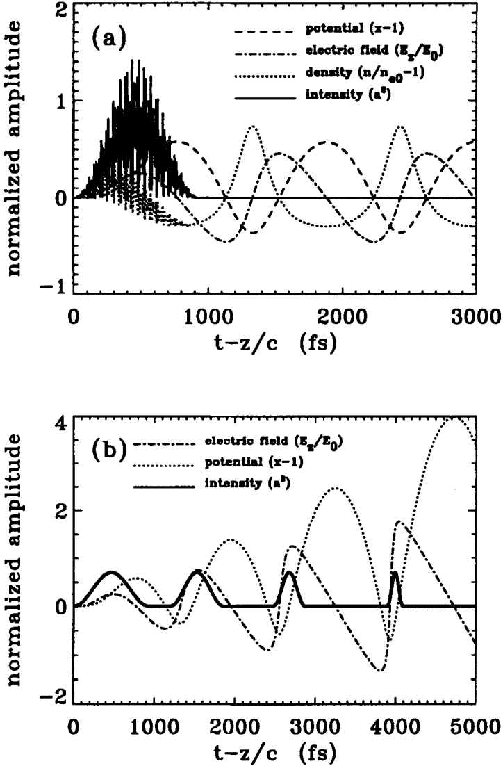
FIG. 4. Numerical solutions for LWFA and RLPA with sine-shaped pulses: (a) single sine pulse at n_e = 10^{16} \text{ cm}^{-3} with a_0 \simeq 1.2 , and (b) an optimized sine pulse train at n_e = 10^{16} \text{ cm}^{-3} with a_0 = 1.2 .
