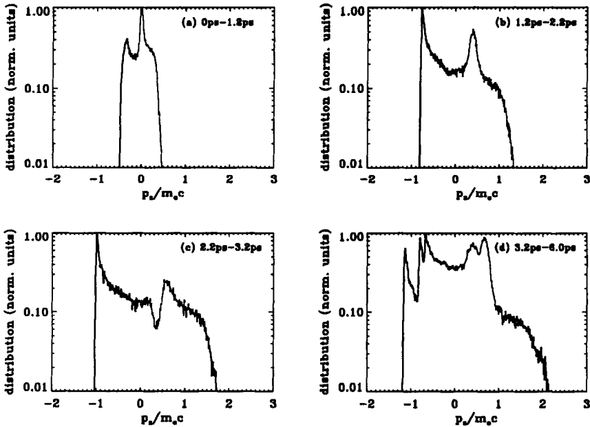
FIG. 14. Normalized electron momentum distribution [ f(p_z/m_e c) vs p_z/m_e c ] from the PIC simulation of the RLPA at various times: (a) t - z/c = 0 - 1.2 ps, (b) t - z/c = 1.2 - 2.2 ps, (c) t - z/c = 2.2 - 3.2 ps, and (d) t - z/c = 3.2 - 6.0 ps.
