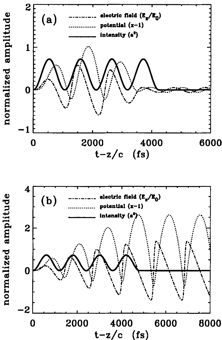
FIG. 8. Numerical solutions for the PBWA: (a) without optimization, showing the effects of detuning, and (b) with optimization.
