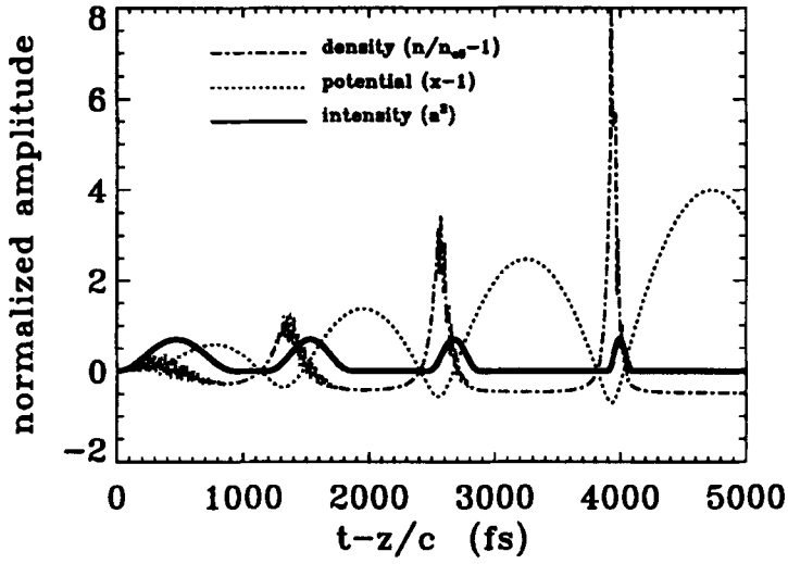
FIG. 6. Numerical solutions for the RLPA with sine-shaped pulses at n_e = 10^{16} \text{cm}^{-3} and a_0 = 1.2 , showing plasma-wave density instead of electric field.
