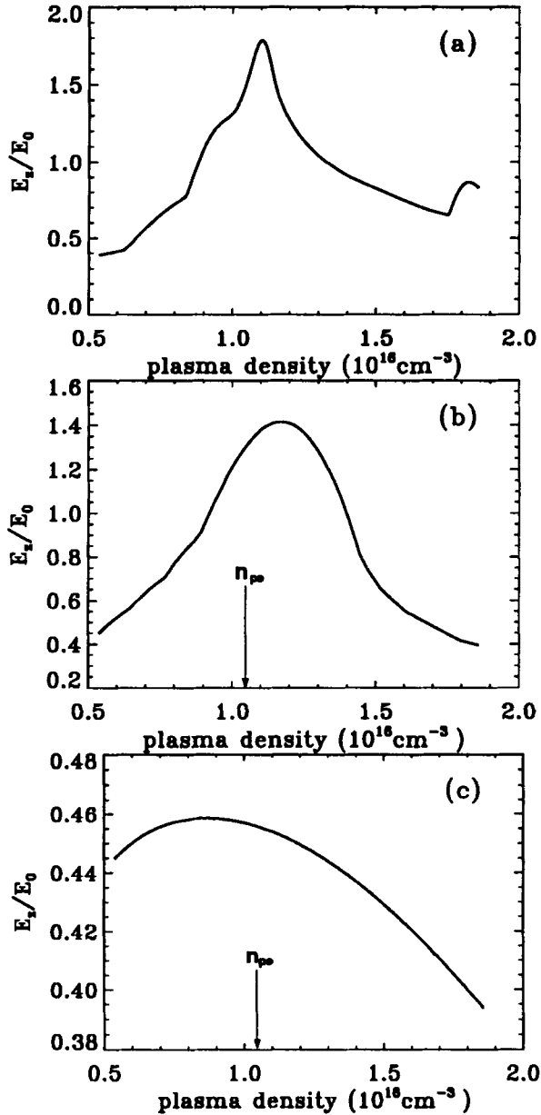
FIG. 10. Final wake-field amplitude as a function of the value of the initial plasma density for: (a) RLPA, (b) PBWA and (c) LWFA. The arrows indicate the densities corresponding to the resonant densities in the linear approximation, \Delta\omega = \omega_p(n_e) for fixed \Delta\omega in the PBWA, and \tau = 2\pi/\omega_p(n_e) for fixed \tau in the LWFA.
