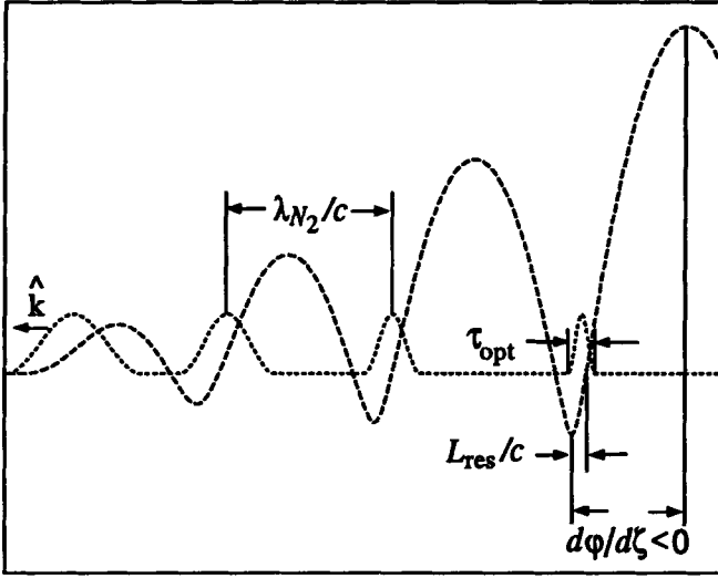
FIG. 5. Legend explaining the definitions of various optimization parameters.
