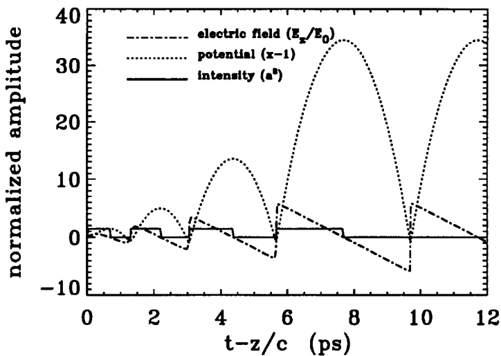
FIG. 3. Numerical solutions for an optimized square pulse train at n_e = 10^{16} \text{ cm}^{-3} and with a_0 = 1.2 .
