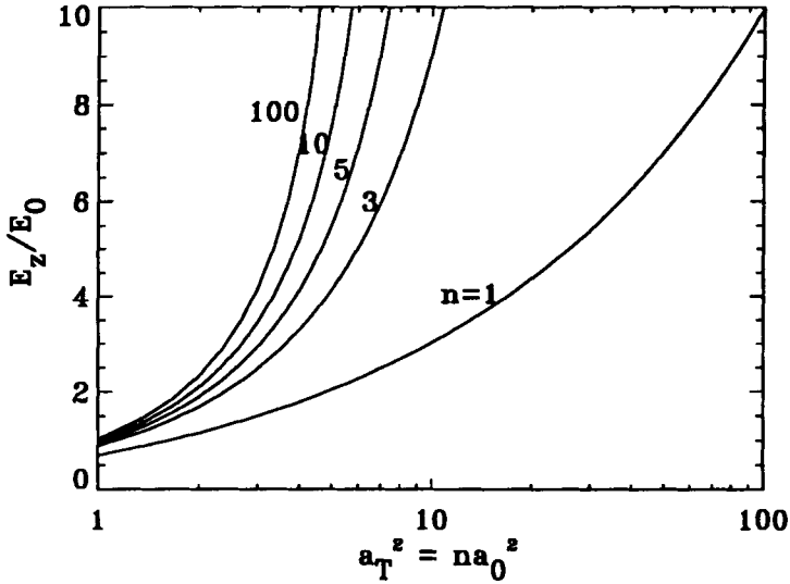
FIG. 1. The maximum electric field ( \hat{E}_{\max,n} ) vs the quantity a_T^2 = n a_0^2 for n = 1, 3, 5, 10 and 100 .
