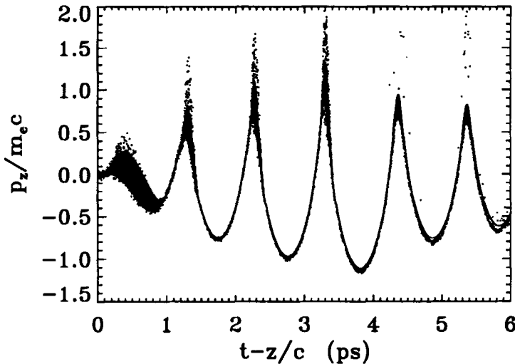
FIG. 13. Phase space diagram of longitudinal momentum vs time ( p_z/m_e c vs t - z/c ) from the PIC simulation of the RLPA. The solid line represents the prediction of the cold fluid theory.
