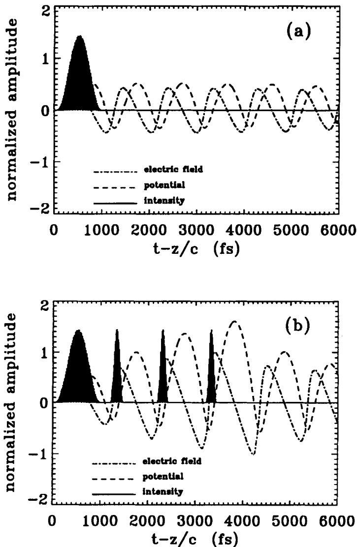
FIG. 12. PIC simulation solution with n_e = 10^{16} \text{ cm}^{-3} and a^2 = 1.44 for (a) a single sine pulse, and (b) four sine pulses. Plasma wave damping is observed at late times only in the latter case.
