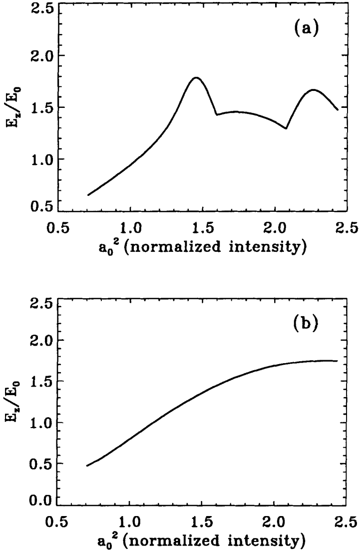
FIG. 11. Final wake-field amplitude as a function only of the laser intensity (constant \lambda_n and L_n ) for (a) RLPA, and (b) PBWA.
