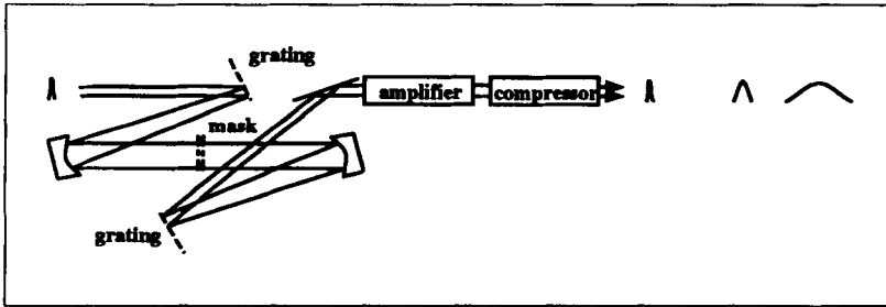
FIG. 15. A variably spaced pulse train with arbitrary pulse widths is produced by use of Fourier filtering in the laser stretcher stage.
