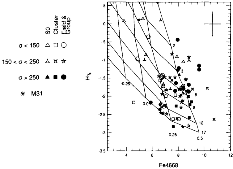
FIGURE 4. Early type galaxies of different size and environment in an age diagnostic diagram; H\gamma_F (Worthey & Ottaviani 1997) versus Fe4668 (Worthey et al. 1994). Models (Worthey 1994) are plotted as a grid labeled with [Fe/H] along the bottom and age in Gyr along the right edge. Approximate observational error is indicated. Three galaxies at very young age and with \sigma < 150 km s -1 are off the scale of this diagram.
