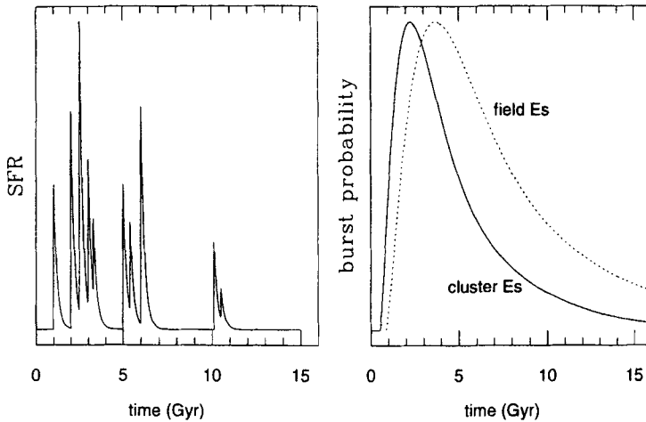
FIGURE 1. A schematic picture of the most probable way that star formation proceeded in E galaxies over the life of the universe. Each galaxy is formed by a series of accretions and mergers. The strengths and times of the star formation bursts are random and have occurred in precursor branches of a merging tree. Bursts are governed by an overall probability distribution in which star formation is more likely to have occurred in the past. The probability curve varies as a function of field/cluster environment and galaxy size.
