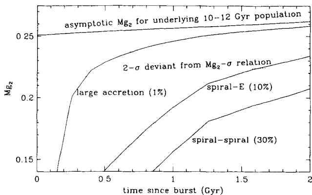
FIGURE 2. The Mg_2 evolution of different fractions by mass (1%, 10%, and 30%) of burst mass / total mass are shown to illustrate how fast an elliptical galaxy will look “normal” after an episode of star formation. Time is counted starting from a burst of star formation that occurred in a passively evolving, 10-Gyr-old “elliptical,” whose unperturbed Mg_2 strength is also shown. One- \sigma and 2- \sigma increments from the Mg_2 - \sigma relation ( \sigma_{\text{measurement}} = \pm 0.018 mag [Bender et al. 1993]) are shown to indicate when a galaxy would “blend in” with the others. The error in Mg_2 is about 0.01 mag. The models shown in this diagram are a variant of the Worthey (1994) models in which Padova evolution is used instead of VandenBerg.
