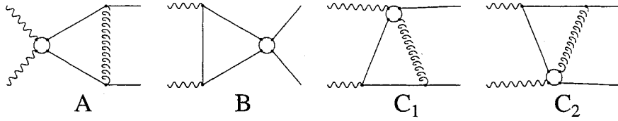
FIGURE 1. The triangle topologies of the one loop box diagram.
