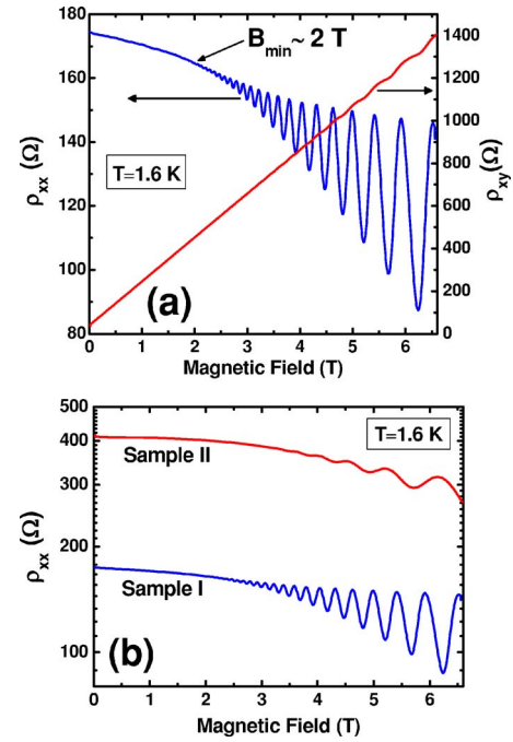
FIG. 1. (Color online) (a) Longitudinal resistivity ( \rho_{xx} ) and Hall resistivity ( \rho_{xy} ) curves of \text{Al}_{0.25}\text{Ga}_{0.75}\text{N}/\text{AlN}/\text{GaN} sample obtained from SdH and Hall measurements at T=1.6 K. (b) SdH measurement results for samples I and II.
