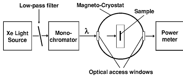
FIG. 4. Schematic diagram of the measurement setup used for PPC experiments.
