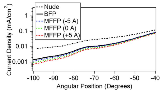
FIG. 9. (Color online) Comparison of off-centerline current density profiles for the nude probe, BFP, and MFFP. Operating conditions are 500 V, 9.80 A and a facility pressure of 1.1 \times 10^{-3} Pa Xe.
