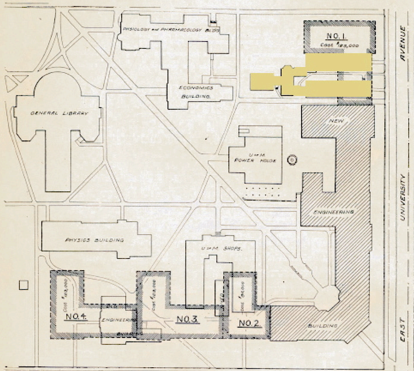
PROPOSED EXTENSION OF THE ENGINEERING BUILDING.
