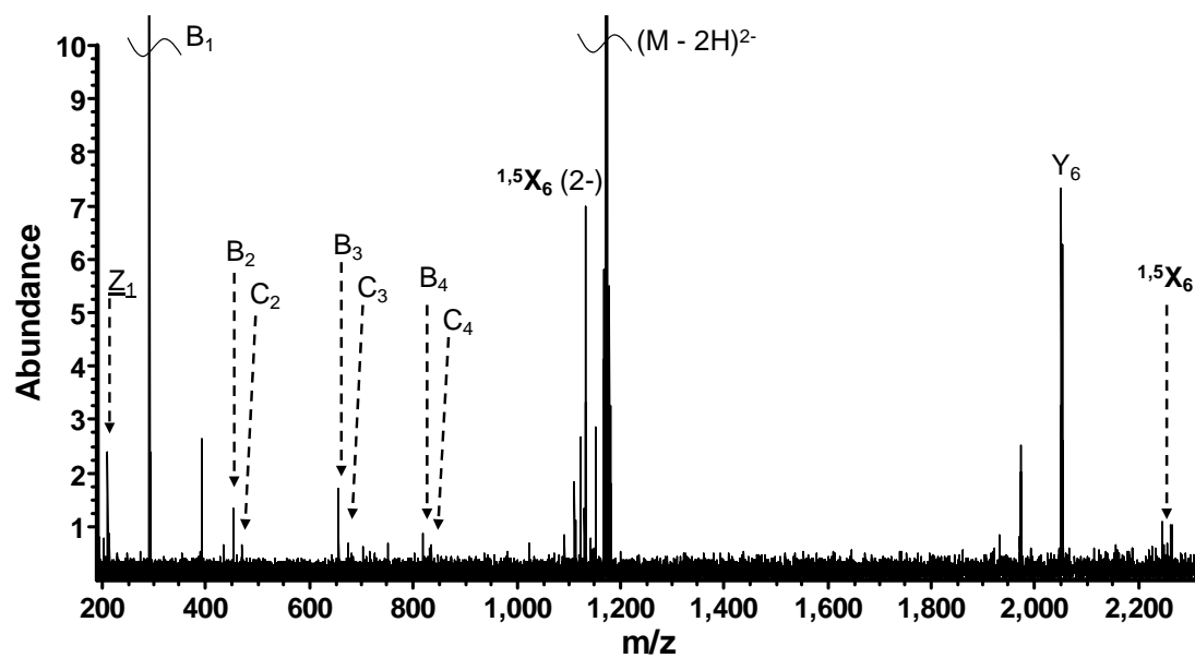
(a) IRMPD of 2-AB labeled N -glycan
