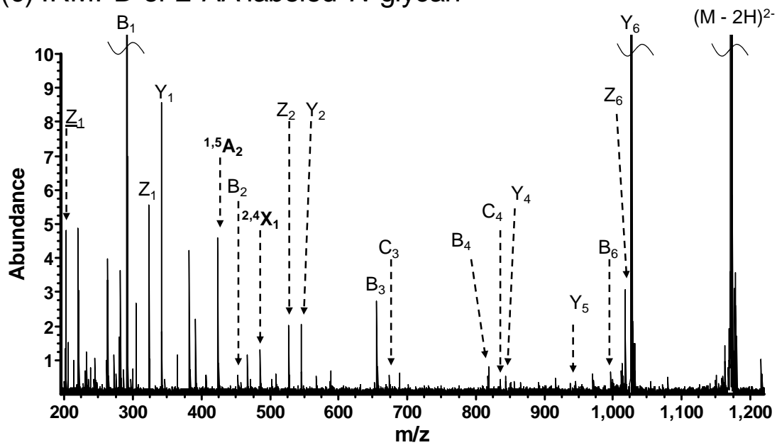
(c) IRMPD of 2-AA labeled N -glycan
