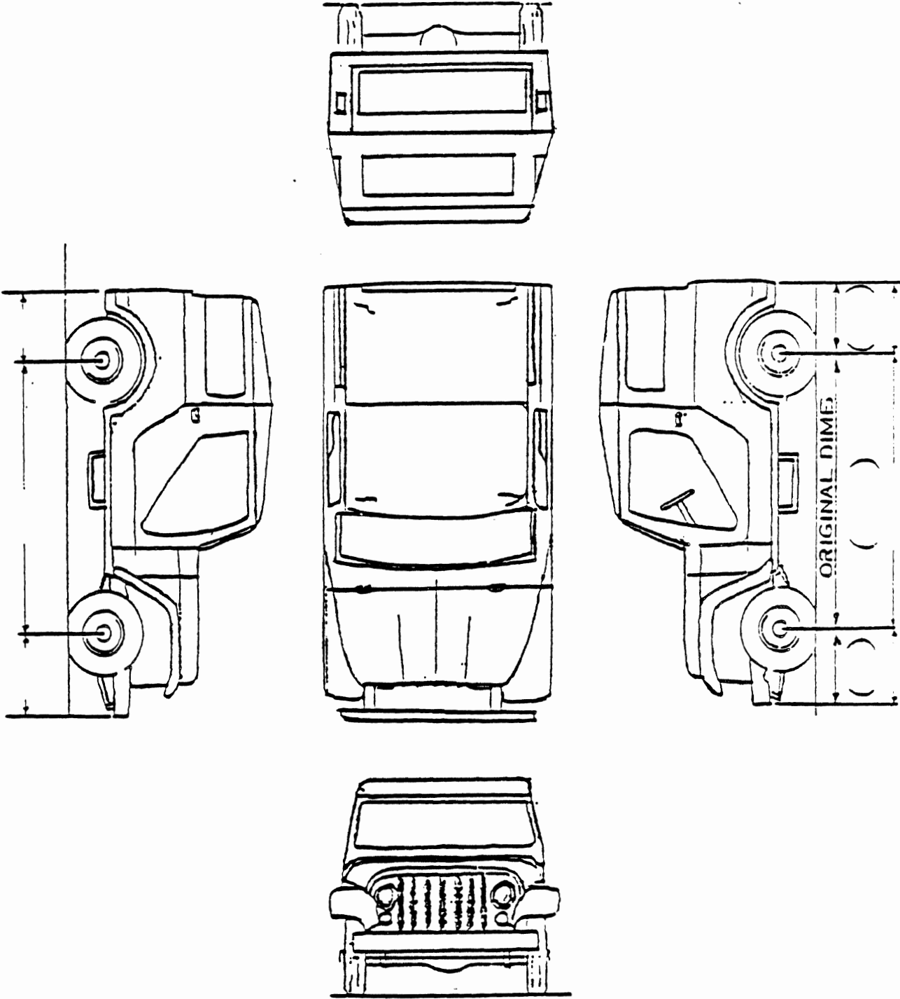
Optional Damage Pictorial Diagram: Two-Door (Short-Wheelbase) Utility Vehicle ("Jeep"-Type Design)
