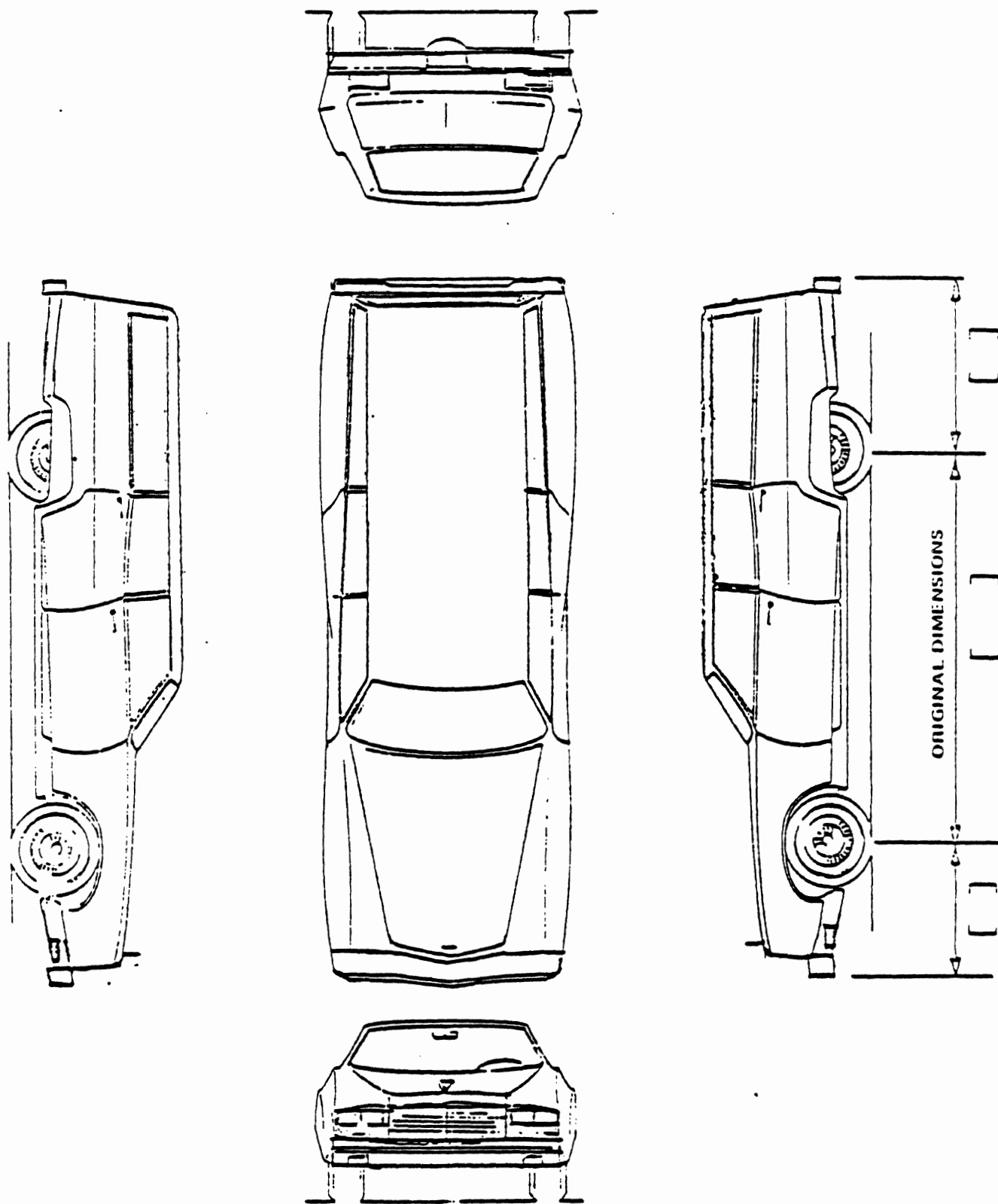
Optional Damage Pictorial Diagram: Four-Door Station Wagon
