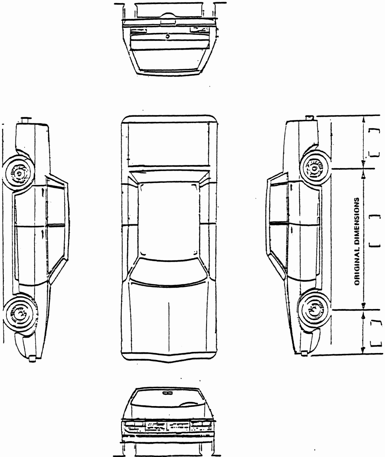
Optional Damage Pictorial Diagram: Four-Door Sedan with Rear or "Opera" Windows
