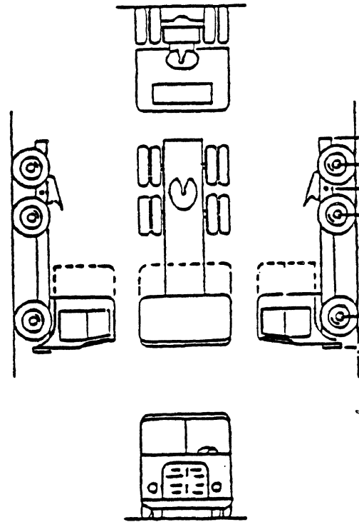
Optional Damage Pictorial Diagram: Conventional Tractor Alone ("Bobtail")
