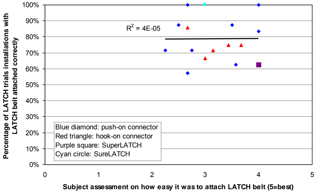
Figure 39. Percentage of LATCH installs with LATCH belt attached correctly vs. subjects’ ratings of ease of attaching the LATCH belt.
