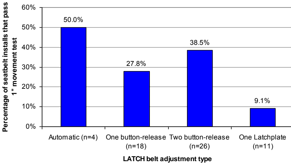
Figure 19. Percentage of seatbelt installations passing 1" test for tightness by LATCH adjuster type.
