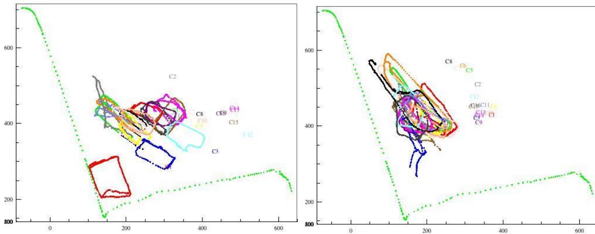
Figure 11. Locations of CRS belt paths when installed RF (left) and FF (right) on the FMVSS 213 buck.
