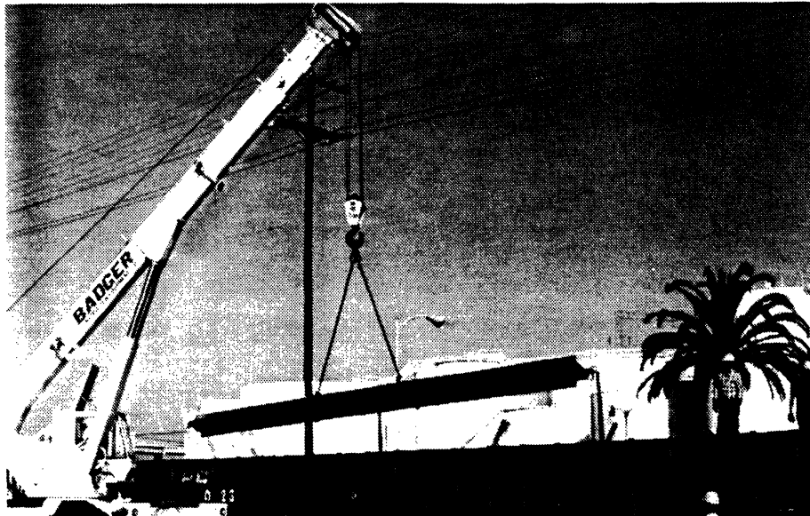
Figure VI-7 MOBILE CRANE UNLOADING SHAPES WITH A CHAIN SLING
