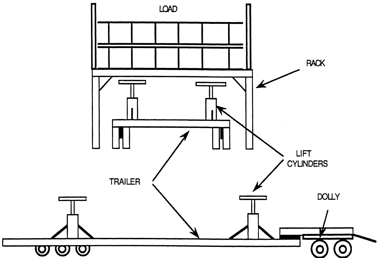
Figure VI-8 LIFT TRAILER
