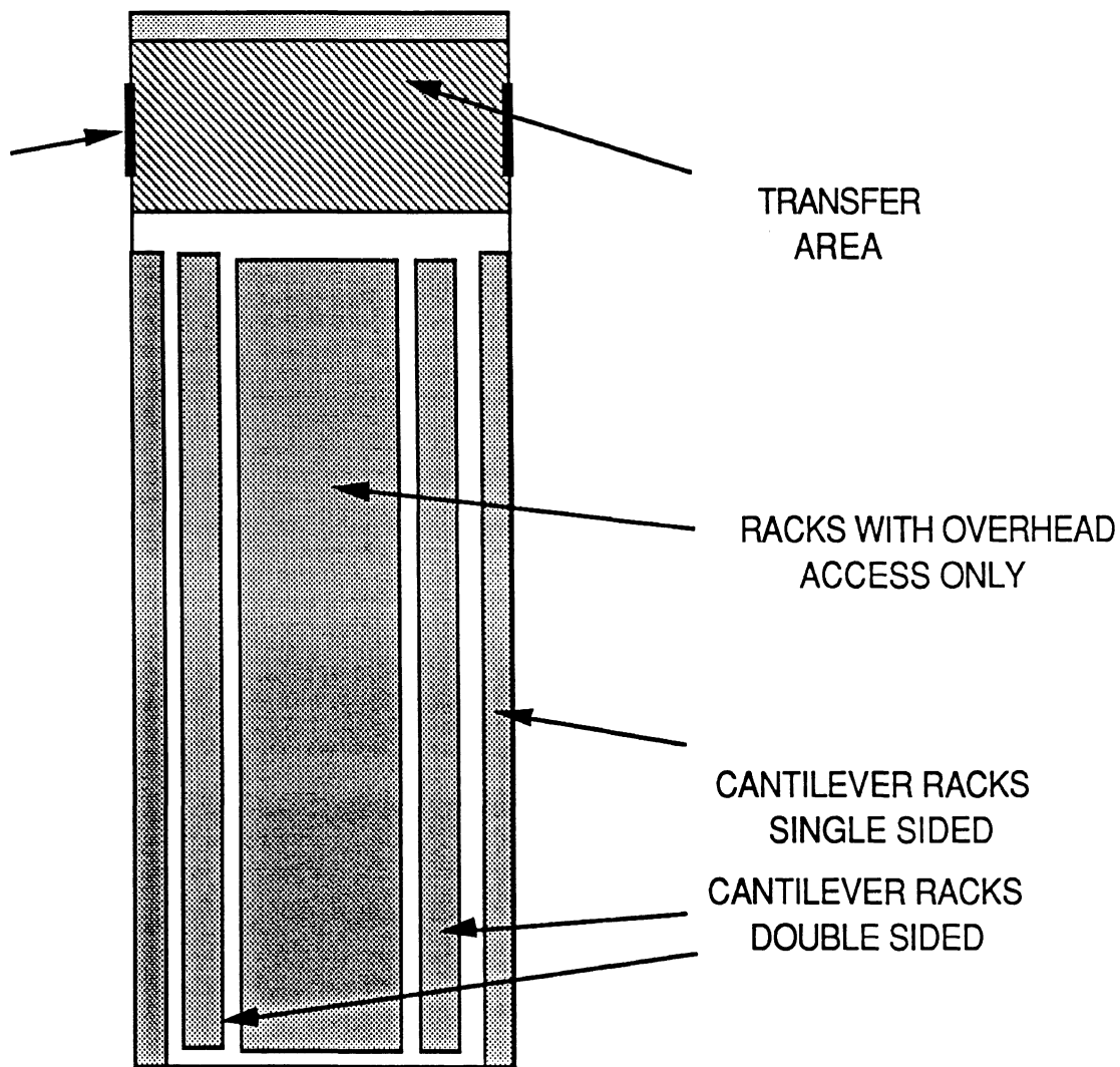
Figure VI-14 STORAGE BUILDING
