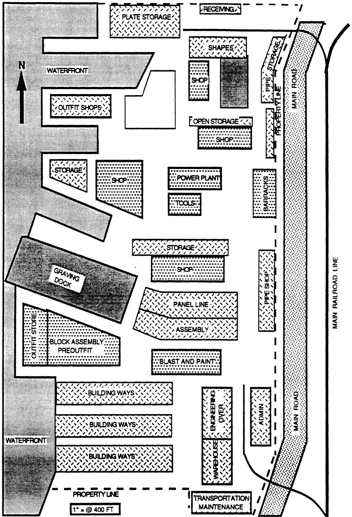
Figure VII-1 SAMPLE SHIPYARD LAYOUT
