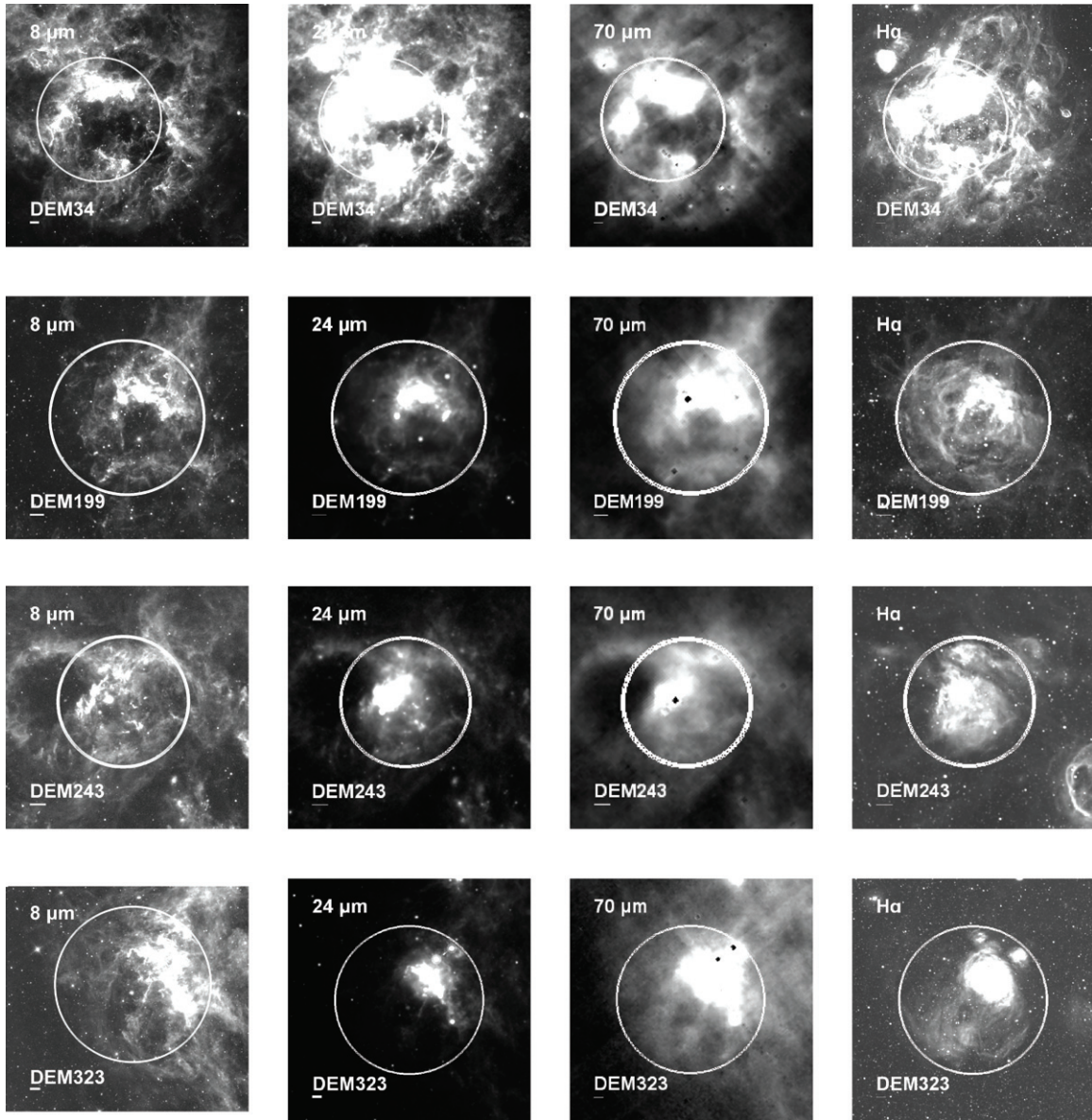
Figure 2. Same as Figure 1, but showing the classical H II regions in the sample.
