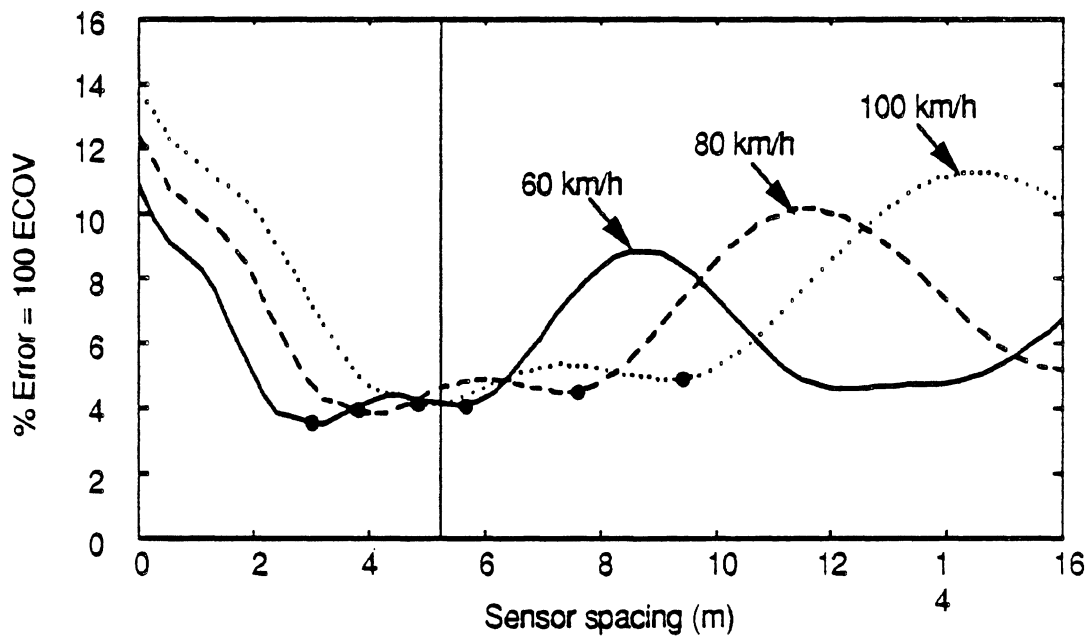
Fig. 5.9 Theoretical graph of \rho vs \Delta , for n = 3 and speeds of 60, 80 and 100 km/h. The design spacing was calculated using an average speed of 80 km/h and an average frequency of 1.9 Hz. The 'solid' circles on each curve correspond to \delta = 1/3 and \delta = 2/3 .
