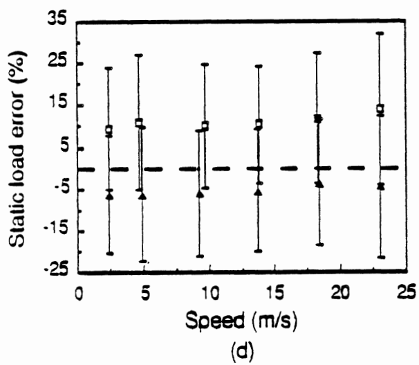
Fig. 3.3 Static load error vs speed, Vehicle S2 (a) Axle 1 (b) Axle 2 (c) Axle 3 (d) Axle 4 (e) Axle 5 Error bars indicate \pm 1 standard deviation
