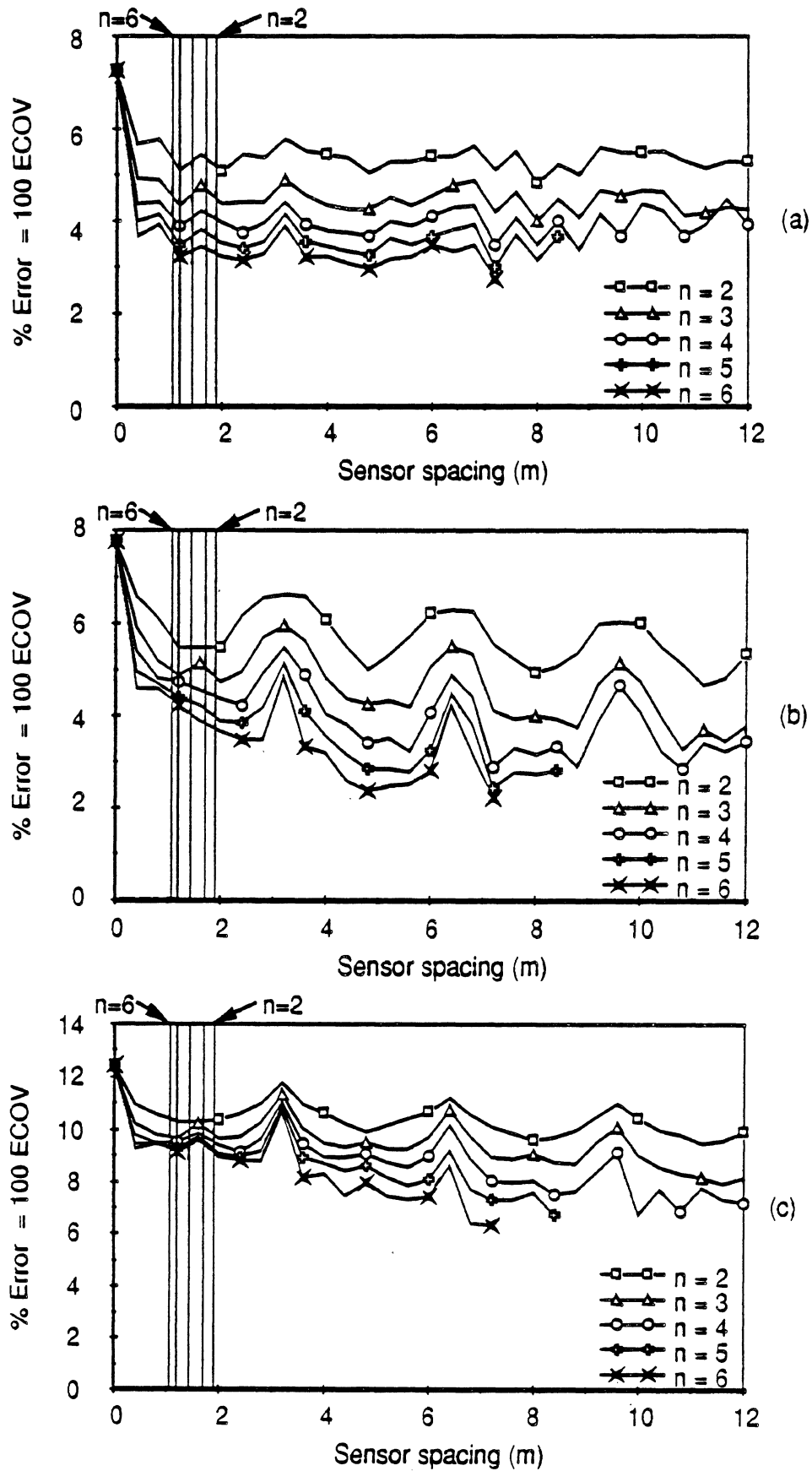
Fig. 5.20 WIM array error vs sensor spacing Vehicle S2, Speed = 9.5 m/s (34 km/h) (a) Axle 1 (b) Axle 3 (c) Axle 5
