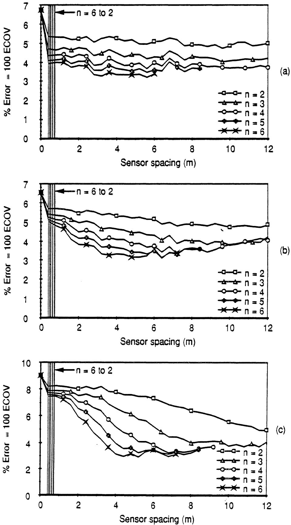
Fig. 5.36 WIM array error vs sensor spacing Vehicle S5, Speed = 3.6 m/s (13 km/h) (a) Axle 1 (b) Axle 3 (c) Axle 5
