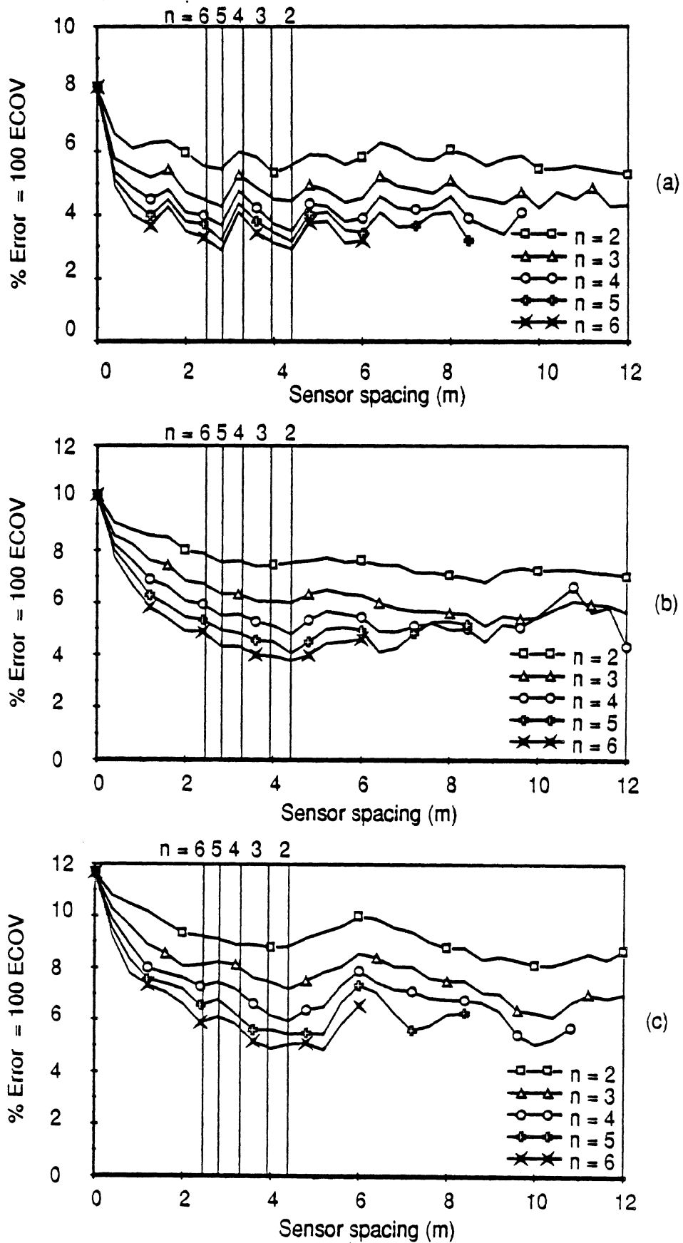
Fig. 5.47 WIM array error vs sensor spacing Vehicle S6, Speed = 22 m/s (79 km/h) (a) Axle 1 (b) Axle 3 (c) Axle 5
