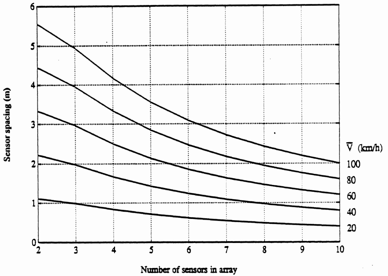
Fig. 4.8 Design chart for multiple sensor WIM systems using eq. 4.22 with \bar{f} = 2.5 Hz.
