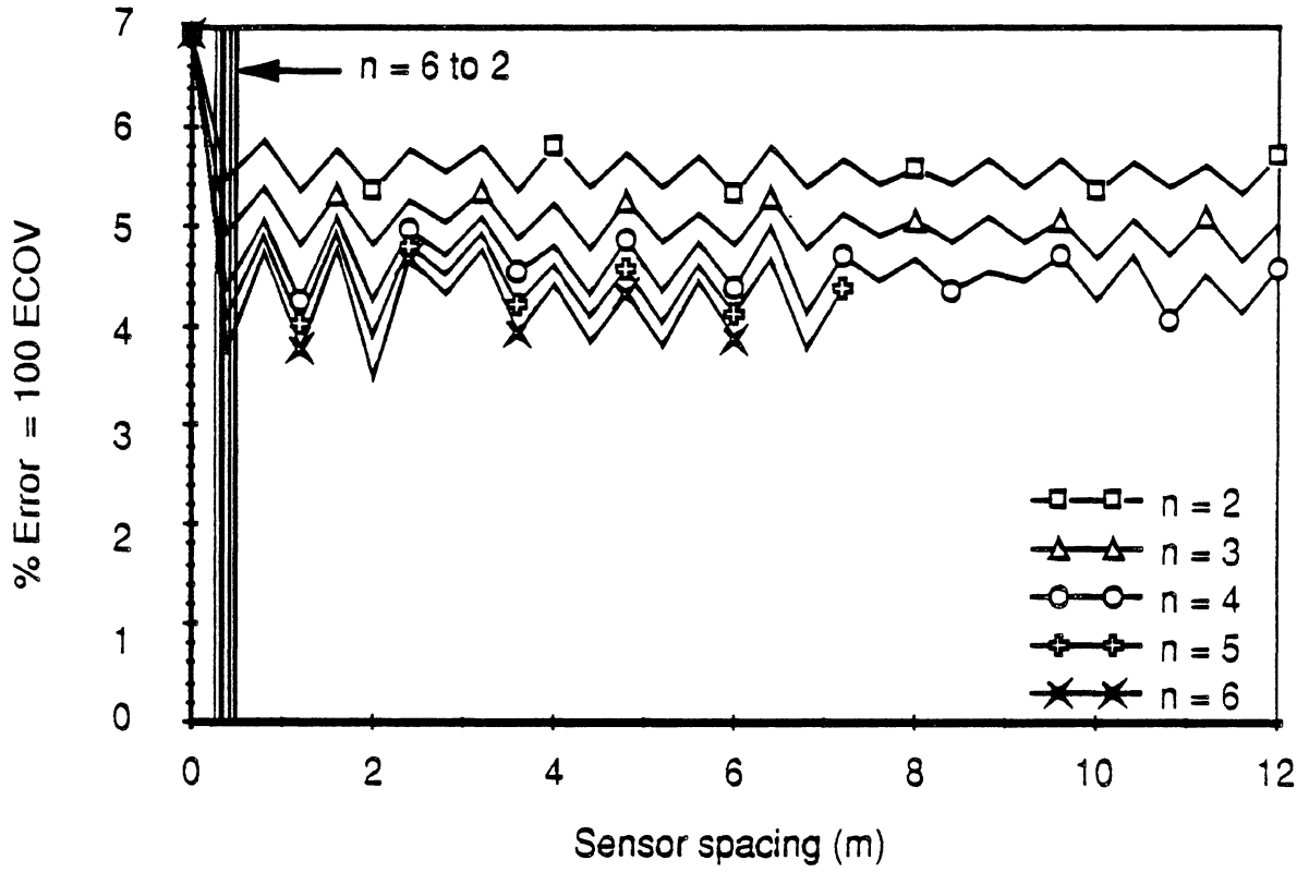
Fig. 5.5 Experimental WIM array Error Coefficient of Variation \rho vs sensor spacing \Delta , vehicle S1, speed 9 km/h, steer axle. Vertical lines denote design spacings according to eq. 4.22.
