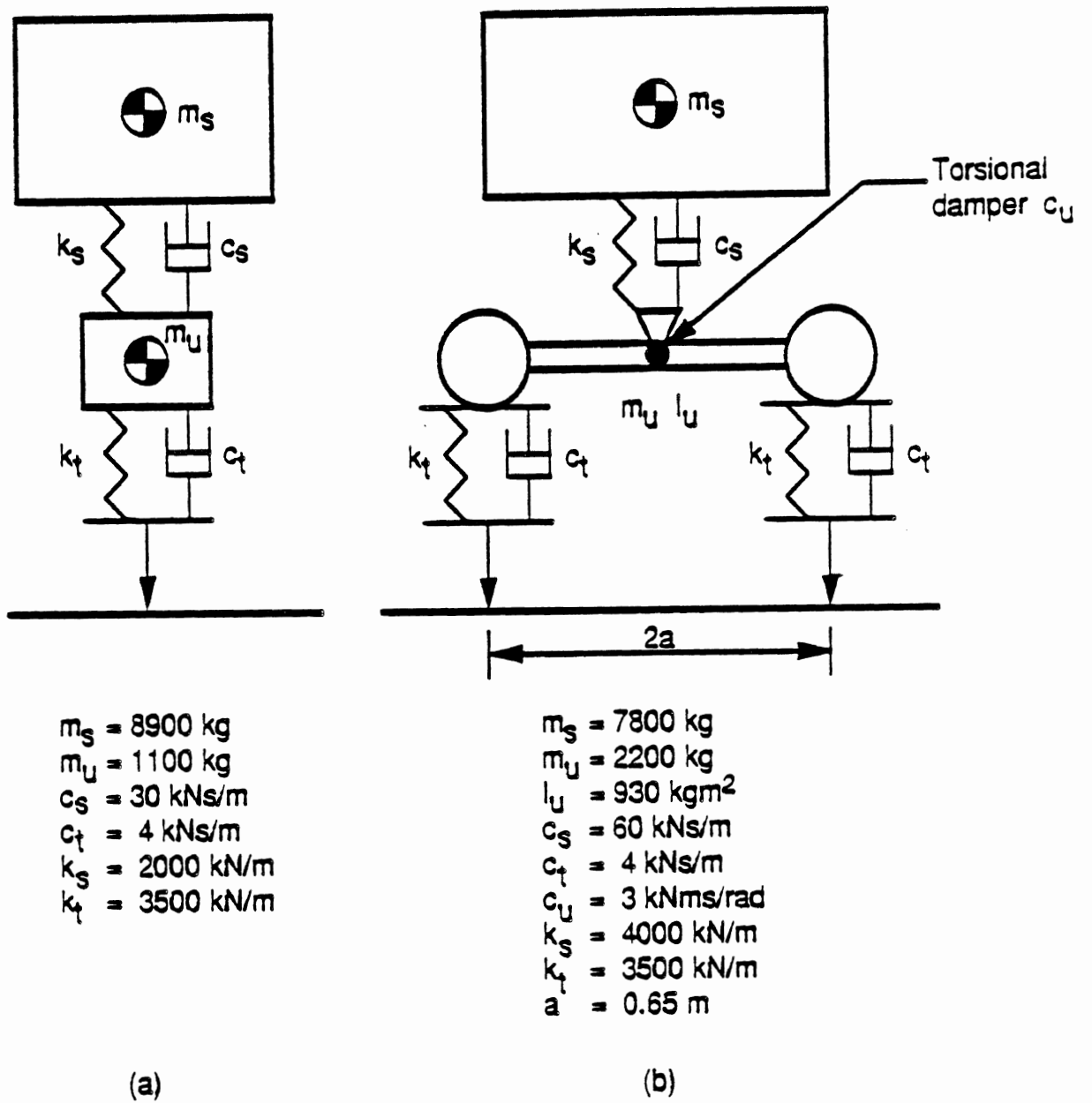
Fig. 4.5 Schematic diagrams of the two vehicle models (a) Model 1: 2 degrees of freedom, '1/4-car' (b) Model 2: 3 degrees of freedom, 'walking-beam.'
