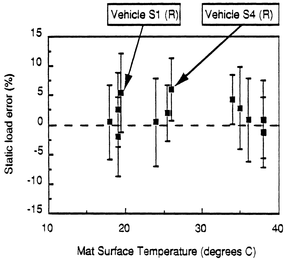
Fig 3.1 Static load errors, steering axles, Vehicles S1-S6. The error bars indicate one standard deviation either side of the mean
