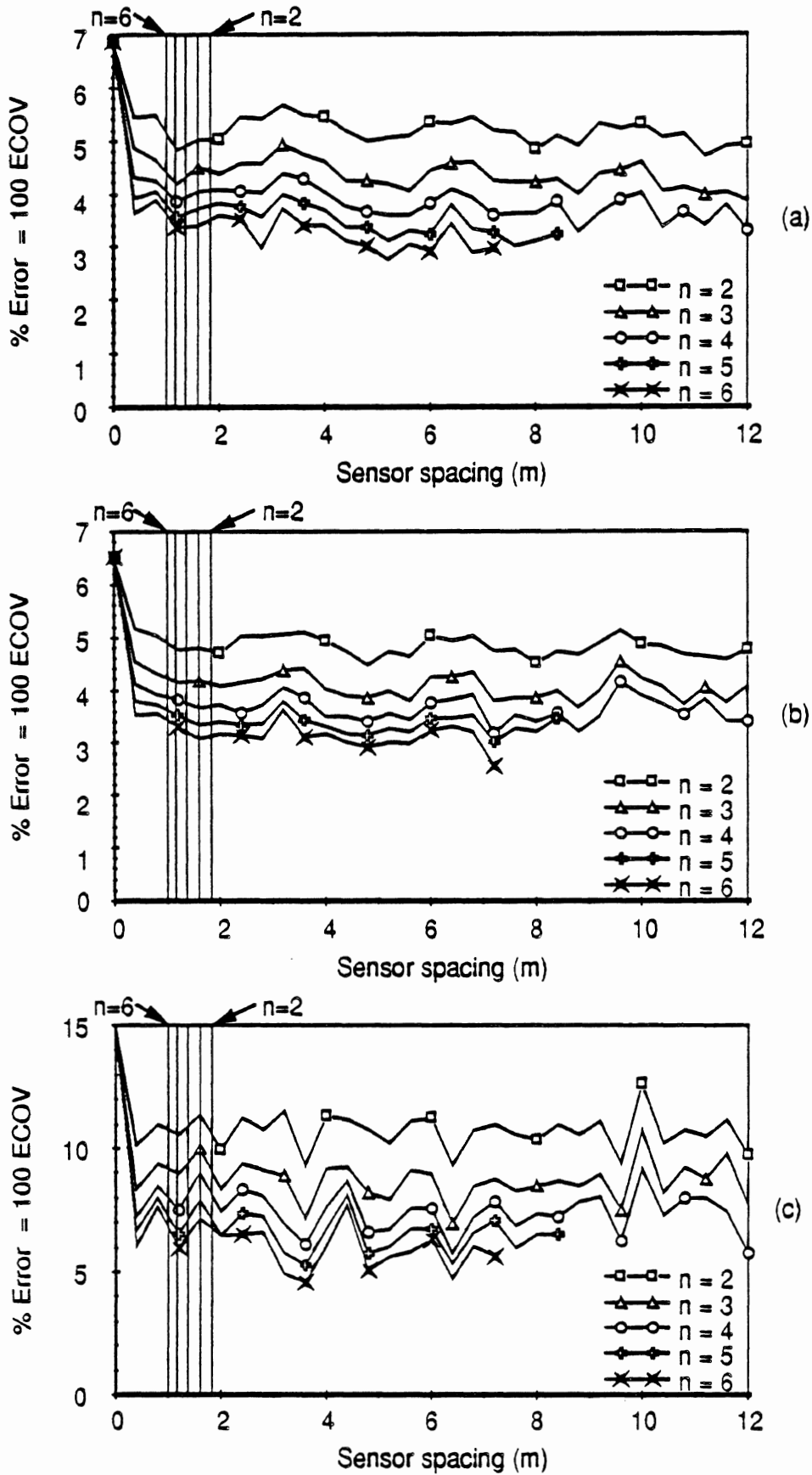
Fig. 5.26 WIM array error vs sensor spacing Vehicle S3, Speed = 9.1 m/s (33 km/h) (a) Axle 1 (b) Axle 3 (c) Axle 5
