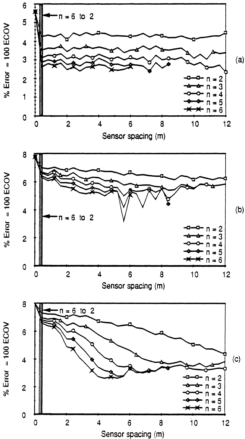
Fig. 5.42 WIM array error vs sensor spacing Vehicle S6, Speed = 2.4 m/s (8.6 km/h) (a) Axle 1 (b) Axle 3 (c) Axle 5
