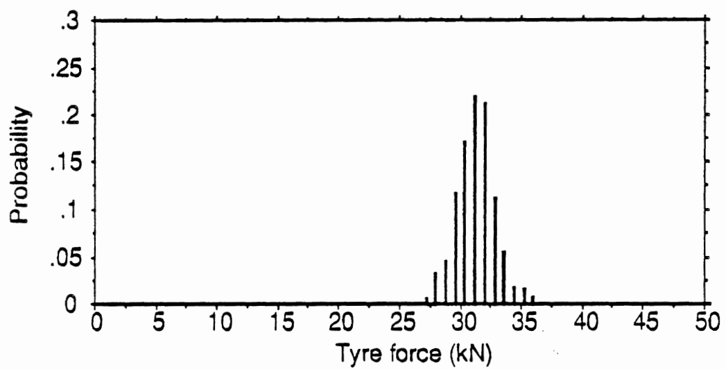
Fig. 5.2 Histograms of WIM average force, Vehicle S4, Axle 5, Speed = 23.7 m/s (85 km/h). (d) single sensor (e) 3 sensors, \Delta = 4.0 m (f) 6 sensors, \Delta = 2.4 m.
