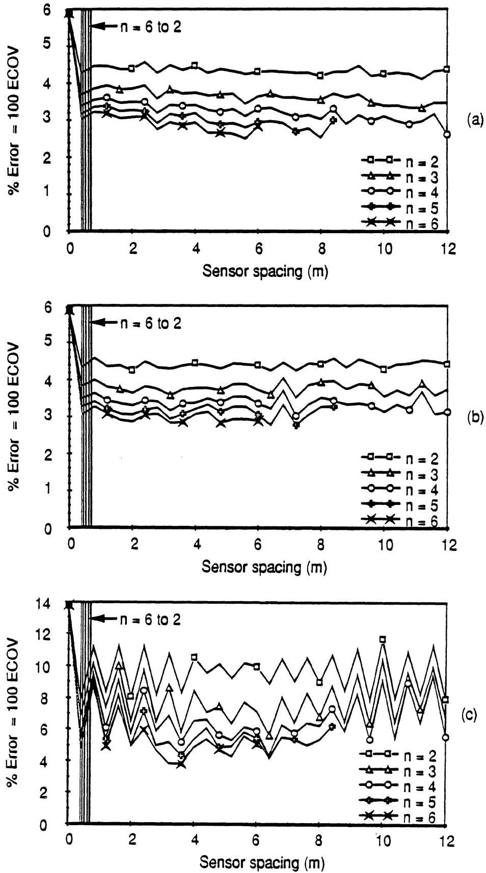
Fig. 5.25 WIM array error vs sensor spacing Vehicle S3, Speed = 3.5 m/s (13 km/h) (a) Axle 1 (b) Axle 3 (c) Axle 5
