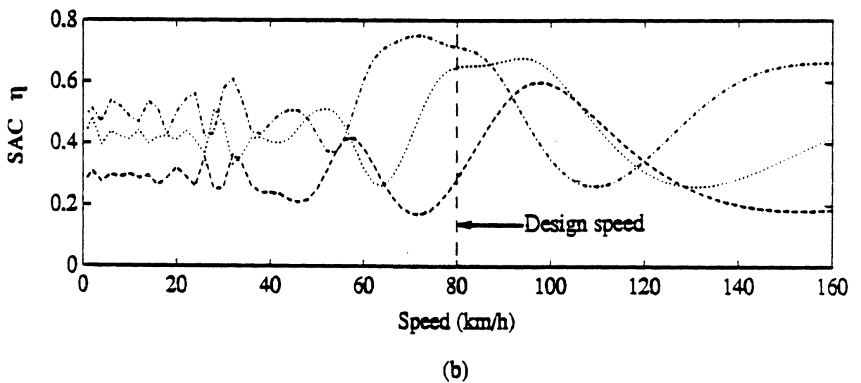
Fig 4.12 Influence of speed on the performance of 2-, 3- and 4-sensor WIM systems, designed for \bar{f} = 2.5 Hz and \bar{V} = 80 km/h, and trafficked by vehicle model 2. (a) Error Coefficient of Variation \rho , (b) Static Accuracy Coefficient \eta . ——— n=1 (DLC), - - - - - n=2 , ..... n=3 , - · - · - n=4 .
