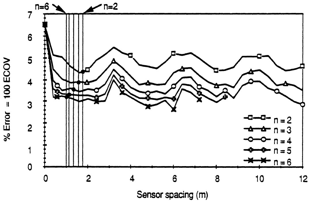
Fig. 5.3 Experimental WIM array Error Coefficient of Variation \rho vs sensor spacing \Delta , Vehicle S1, speed 32 km/h, steer axle. Vertical lines denote design spacings according to eq 4.22.
