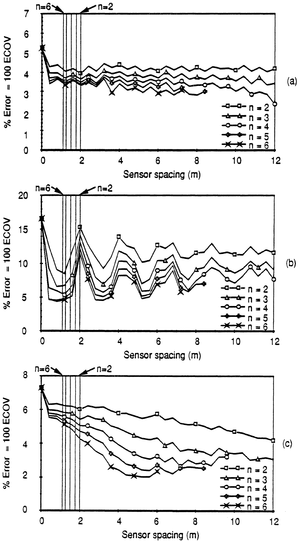
Fig. 5.32 WIM array error vs sensor spacing Vehicle S4, Speed = 9.9 m/s (36 km/h) (a) Axle 1 (b) Axle 3 (c) Axle 5
