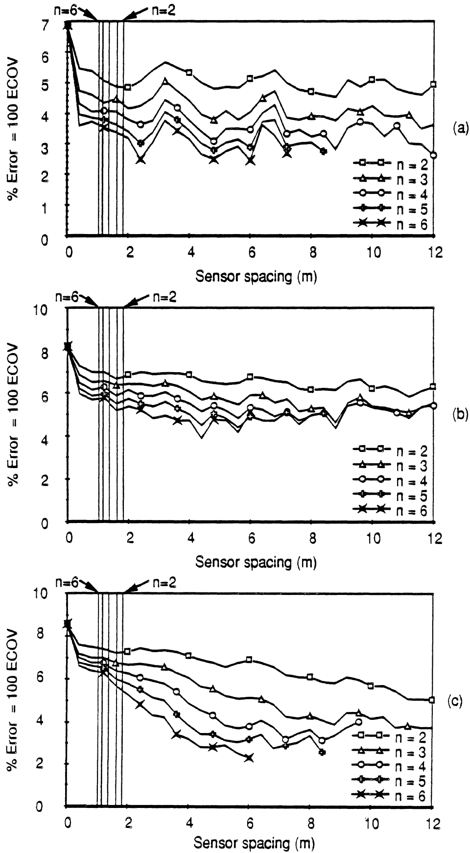
Fig. 5.44 WIM array error vs sensor spacing Vehicle S6, Speed = 9.1 m/s (33 km/h) (a) Axle 1 (b) Axle 3 (c) Axle 5
