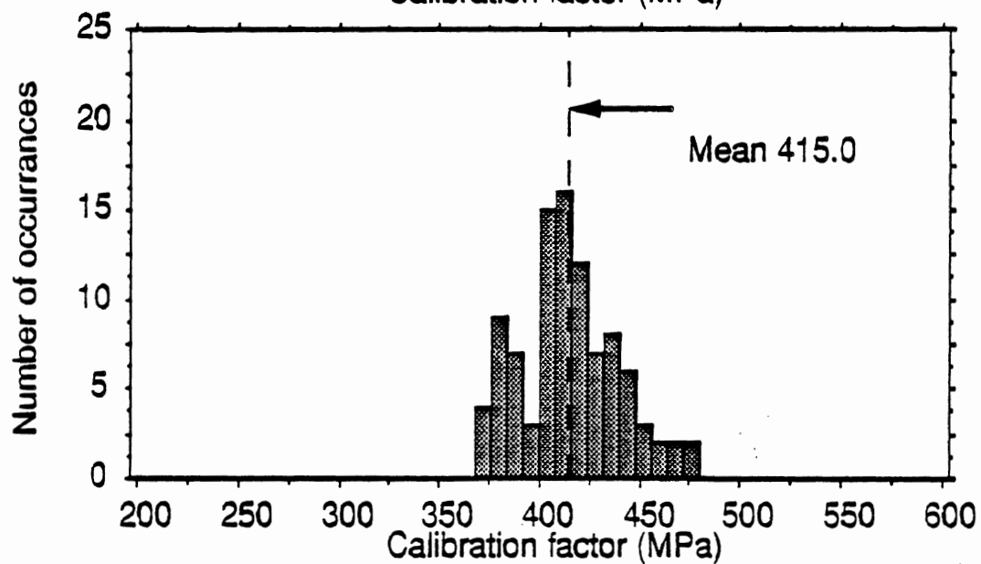
Fig. 2.3 Histograms of sensor calibration factors (a) Bare sensor calibrator (b) 'In-situ' calibrator (c) Field calibration with steer axles of 6 vehicles
