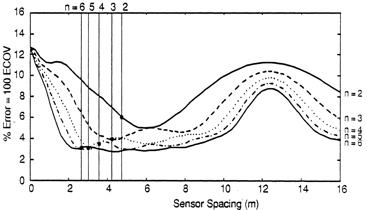
Fig. 5.8 Theoretical WIM array Error Coefficient of Variation p vs sensor spacing \Delta , 1/4-car model, speed = 85 km/h. Vertical lines denote design spacings according to eq 4.22.
