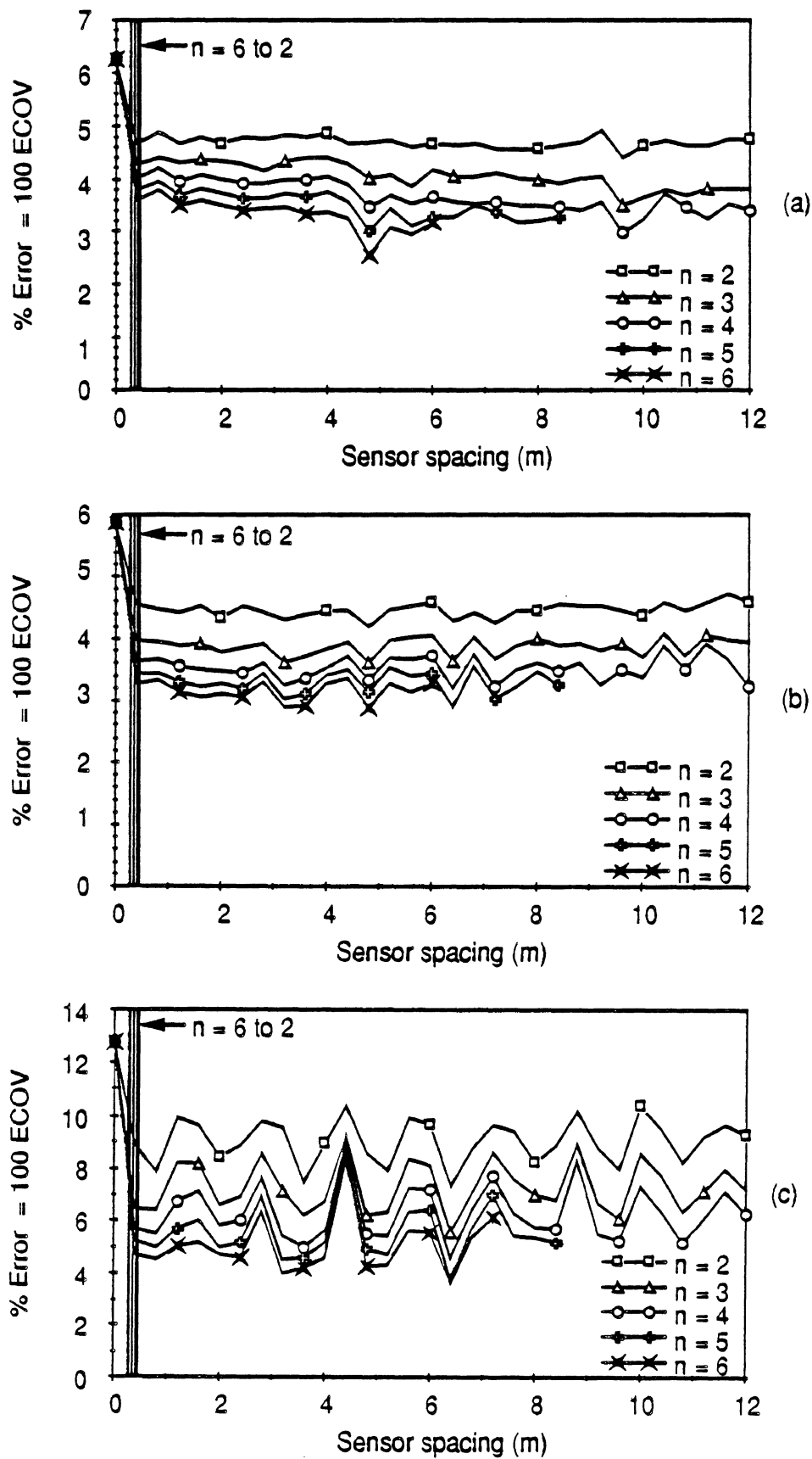
Fig. 5.24 WIM array error vs sensor spacing Vehicle S3, Speed = 2.4 m/s (8.5 km/h) (a) Axle 1 (b) Axle 3 (c) Axle 5
