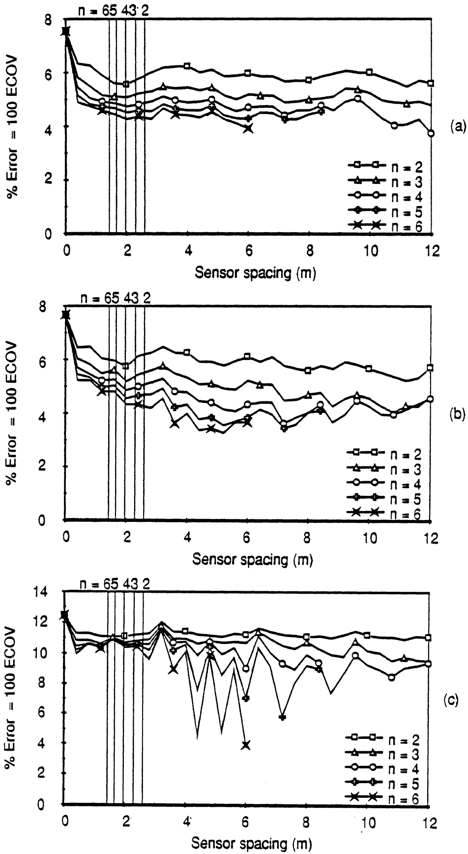
Fig. 5.15 WIM array error vs sensor spacing Vehicle S1, Speed = 13.0 m/s (47 km/h) (a) Axle 1 (b) Axle 3 (c) Axle 5
