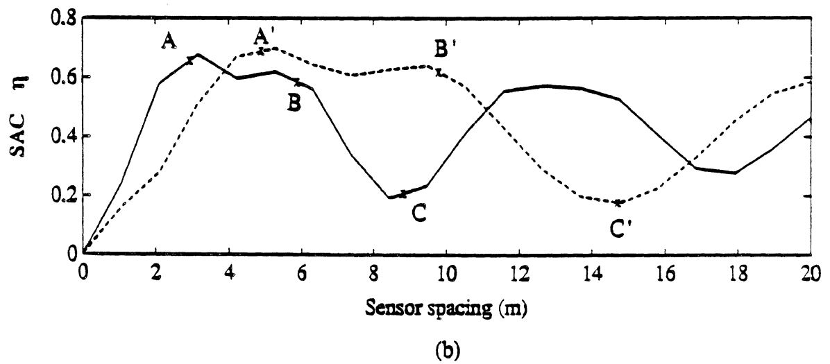
Fig. 4.7 WIM system performance versus sensor spacing \Delta for vehicle model 1. Points A, B, C etc. were calculated according to the theory for sinusoidal inputs. (a) Error Coefficient of Variation \rho . (b) Static Accuracy Coefficient \eta . — = 60 km/h, - - - = 100 km/h
