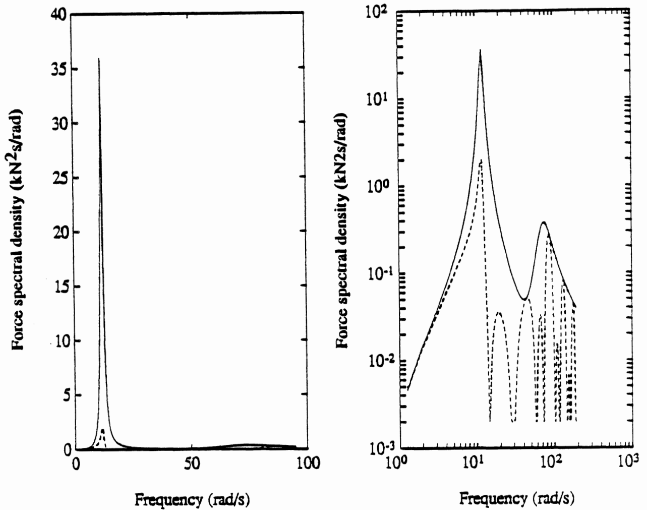
Fig. 4.6 Tyre force spectral density S_{pp}(\omega) and the WIM array error spectral density S_{ee}(\omega) for vehicle model 1 travelling at 100 km/h over a WIM array with n=3 and \Delta = 4 m.
