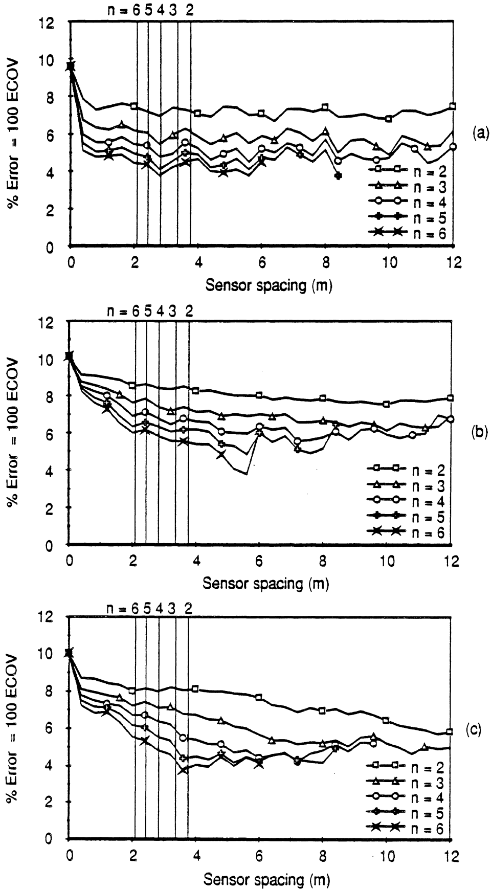
Fig. 5.40 WIM array error vs sensor spacing Vehicle S5, Speed = 18.9 m/s (68 km/h) (a) Axle 1 (b) Axle 3 (c) Axle 5
