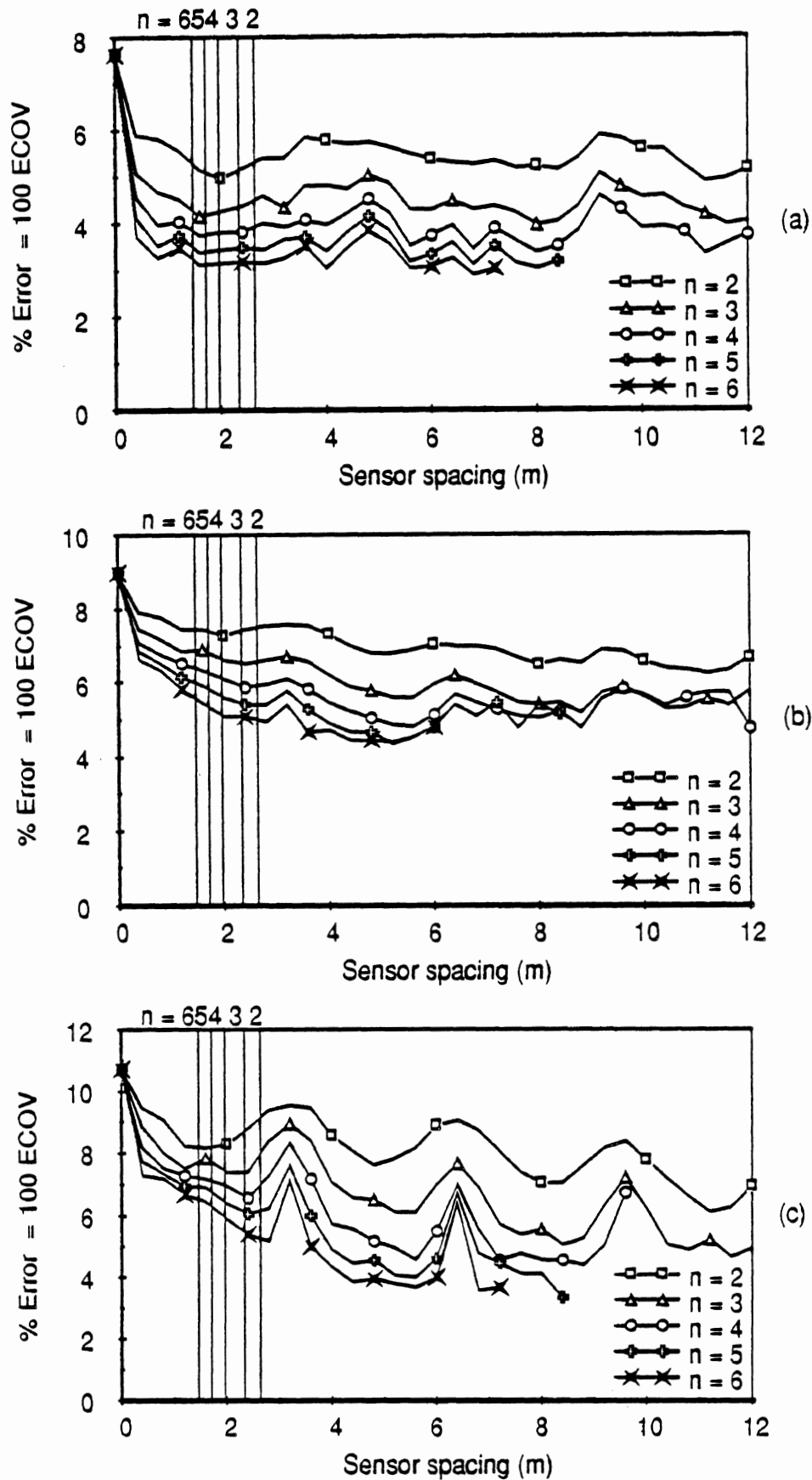
Fig. 5.45 WIM array error vs sensor spacing Vehicle S6, Speed = 13.2 m/s (47 km/h) (a) Axle 1 (b) Axle 3 (c) Axle 5
