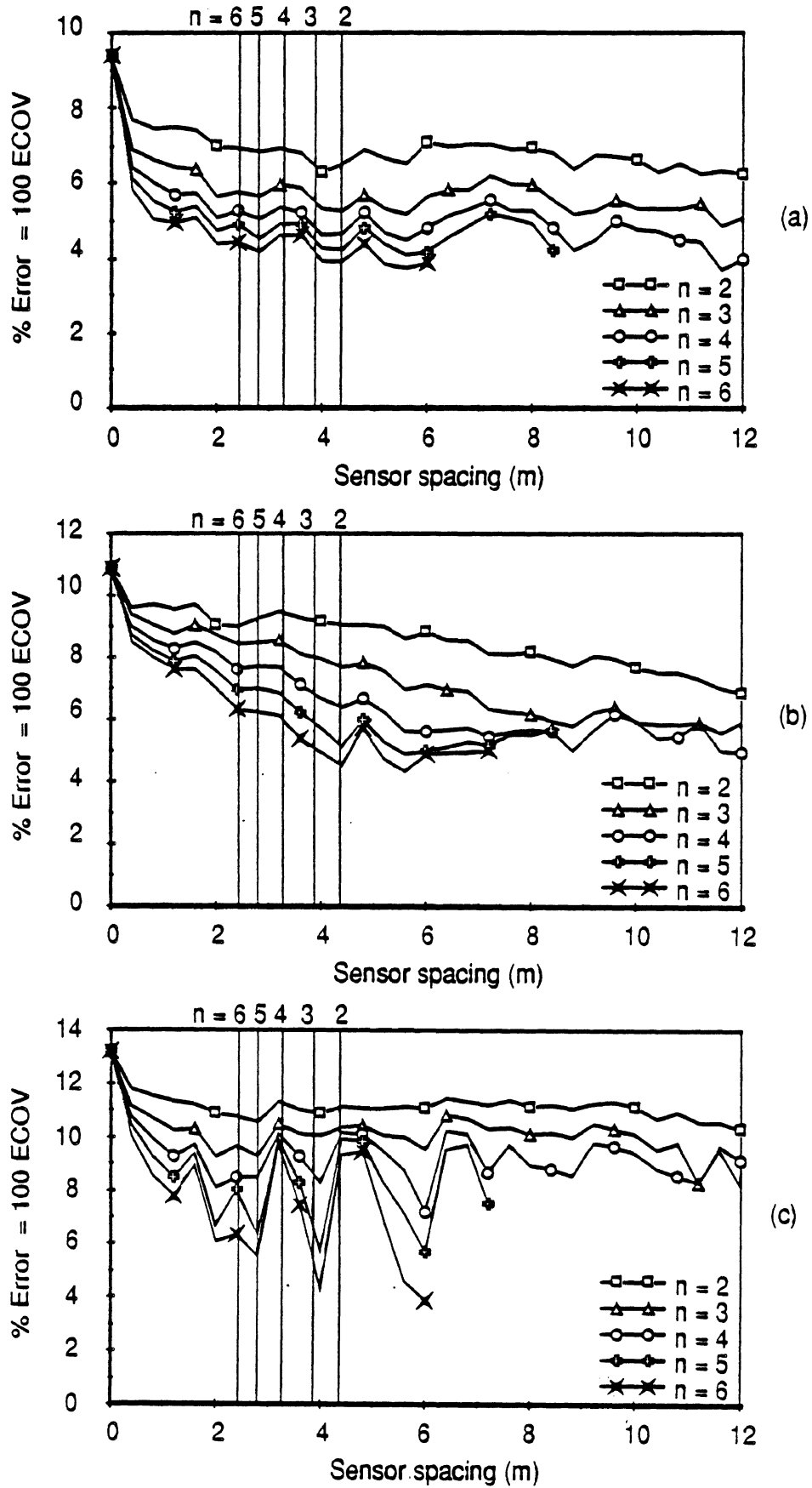
Fig. 5.17 WIM array error vs sensor spacing Vehicle S1, Speed = 21.8 m/s (79 km/h) (a) Axle 1 (b) Axle 3 (c) Axle 5
