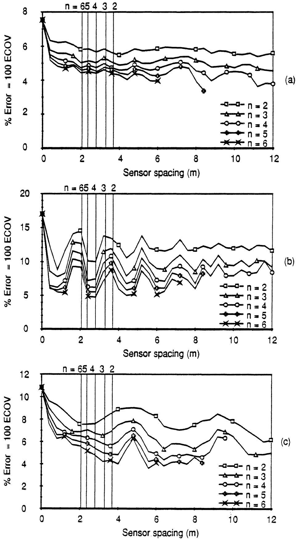
Fig. 5.34 WIM array error vs sensor spacing Vehicle S4, Speed = 18.6 m/s (67 km/h) (a) Axle 1 (b) Axle 3 (c) Axle 5
