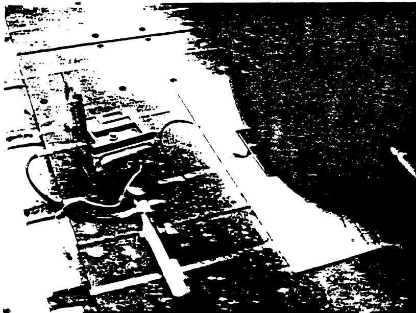
Figure 2. The calibrating equipment placed on the wheel force measuring mat
