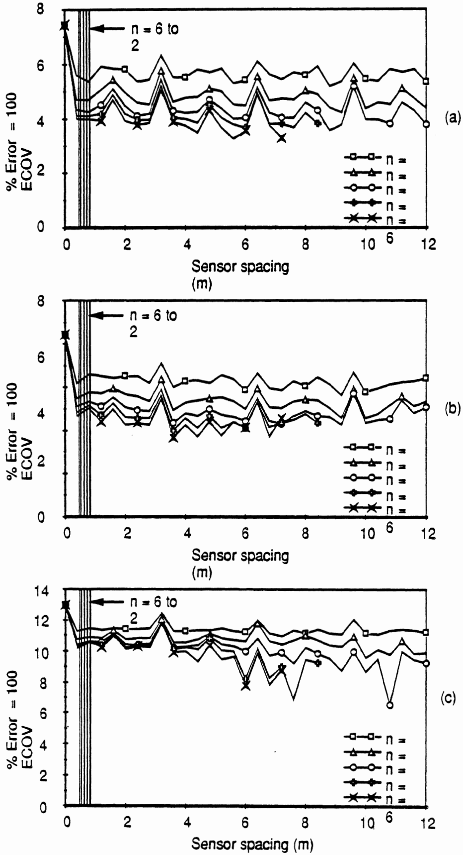
Fig. 5.13 WIM array error vs sensor spacing Vehicle S1, Speed = 4.1 m/s (15 km/h) (a) Axle 1 (b) Axle 3 (c) Axle 5
