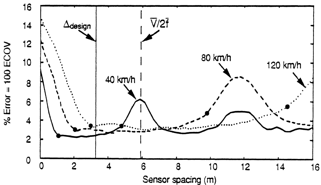
Fig. 5.10 Theoretical graph of \rho vs \Delta , for n = 6 and speeds of 40, 80 and 120 km/h. The design spacing was calculated using an average speed of 80 km/h and an average frequency of 1.9 Hz. The 'solid' circles on each curve correspond to \delta = 1/6 and \delta = 5/6 .
