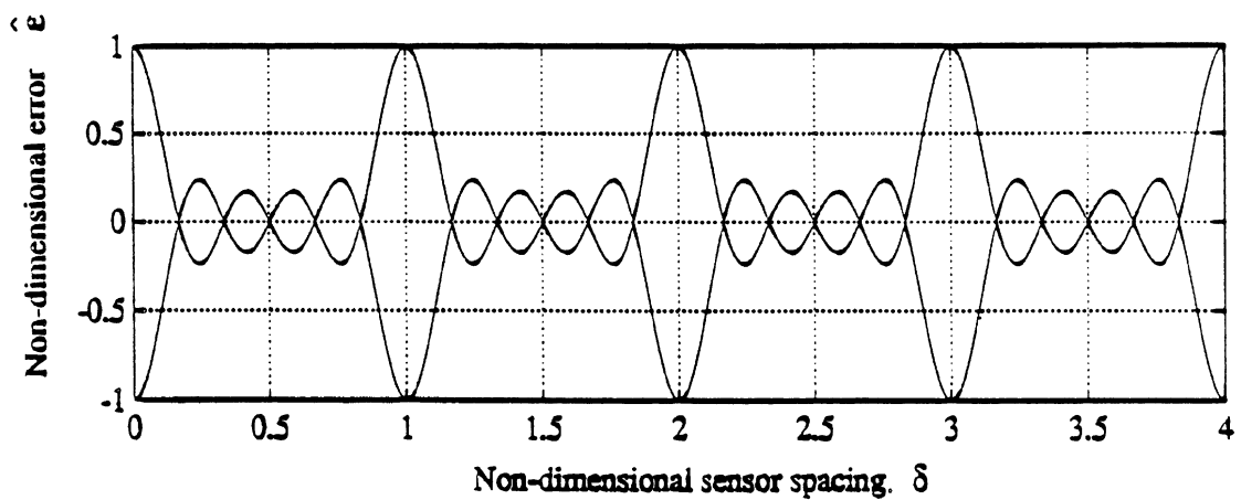
Fig. 4.4 Plot of the envelope error \hat{\epsilon} from equation 4.7 with n=6 , showing the repetition of the 'unit cell' pattern ( 0 \leq \delta < 1 ) due to aliasing.
