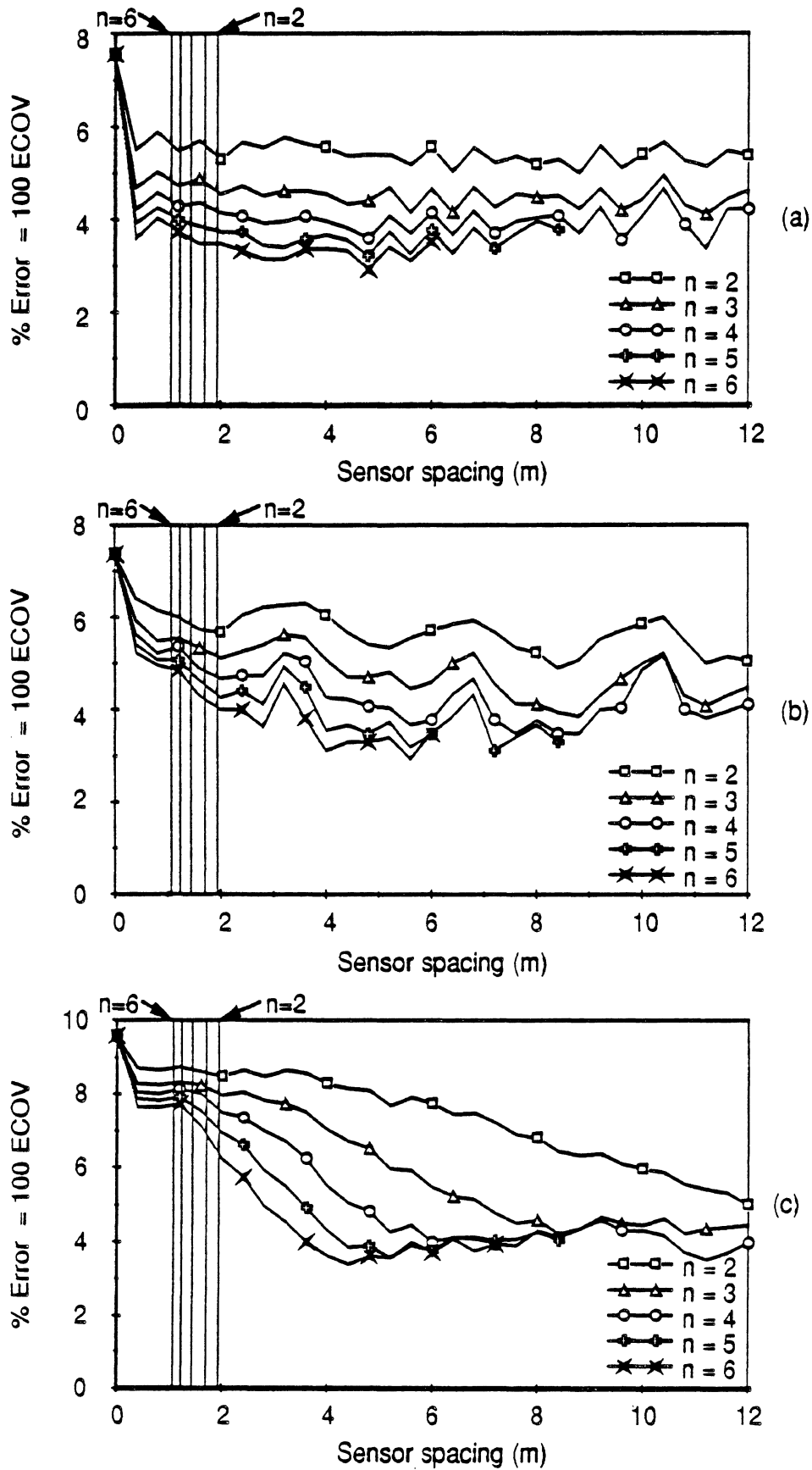
Fig. 5.38 WIM array error vs sensor spacing Vehicle S5, Speed = 9.6 m/s (35 km/h) (a) Axle 1 (b) Axle 3 (c) Axle 5
