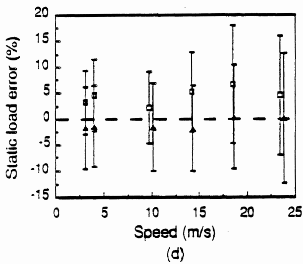
Fig. 3.5 Static load error vs speed, Vehicle S4 (a) Axle 1 (b) Axle 2 (c) Axle 3 (d) Axle 4 (e) Axle 5 Error bars indicate \pm 1 standard deviation
