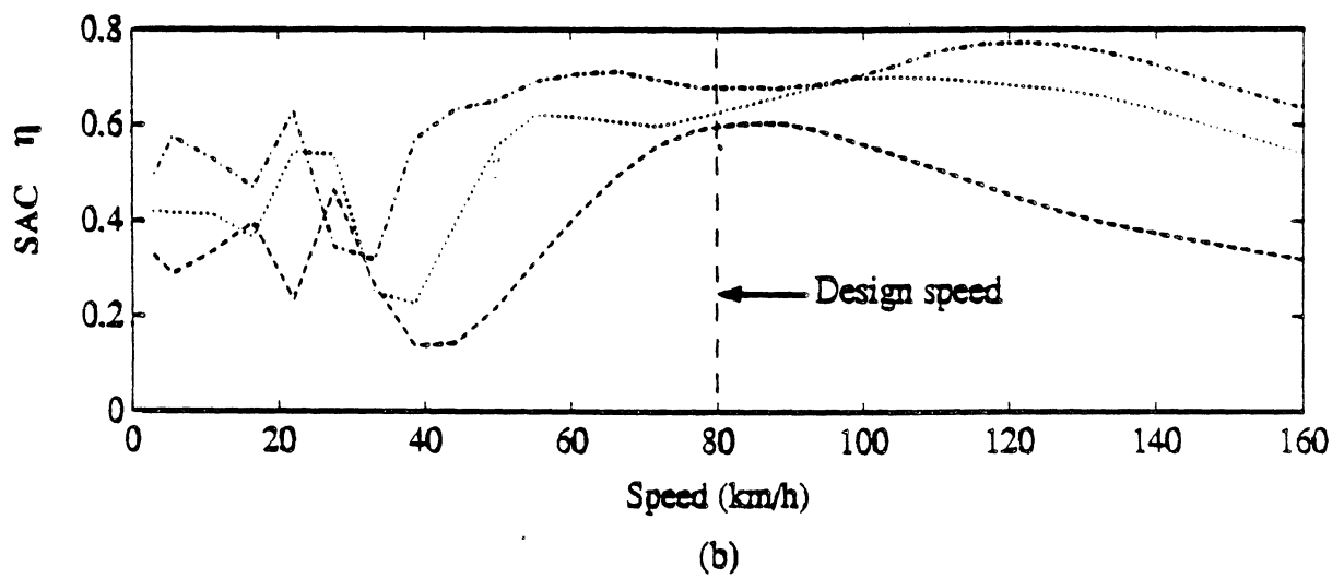
Fig. 4.9 Influence of speed on the performance of 2-, 3- and 4-sensor WIM systems, designed for an average traffic speed of 80 km/h, traversed by vehicle model 1. (a) Error Coefficient of Variation \rho . (b) Static Accuracy Coefficient \eta . — n=1 (DLC), — n=2 , ..... n=3 , -.-.- n=4 .
