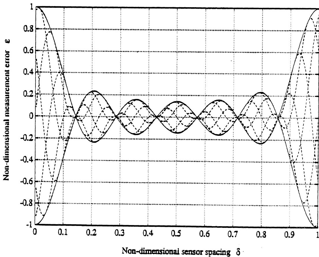
Fig. 4.2 Plot of equation 4.5 for n=7 with 5 different phase angles, \phi = 2\pi/5, 4\pi/5, \dots, 2\pi , (dashed lines) as well as the envelope error \hat{\epsilon} from eq. 4.7, (solid lines).
