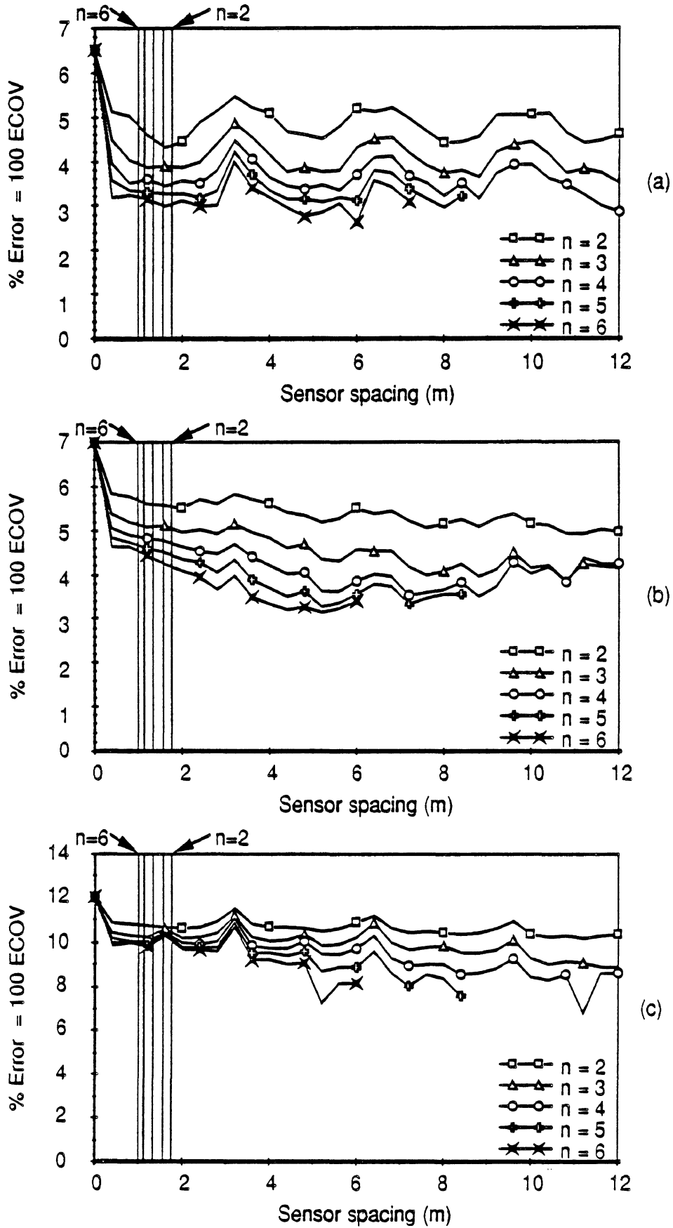
Fig. 5.14 WIM array error vs sensor spacing Vehicle S1, Speed = 8.9 m/s (32 km/h) (a) Axle 1 (b) Axle 3 (c) Axle 5
