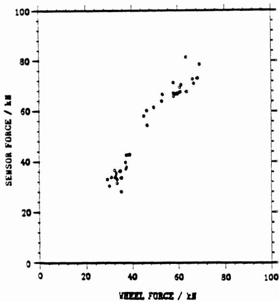
Figure 4. Force measured by sensor 1 against force measured by lorry
