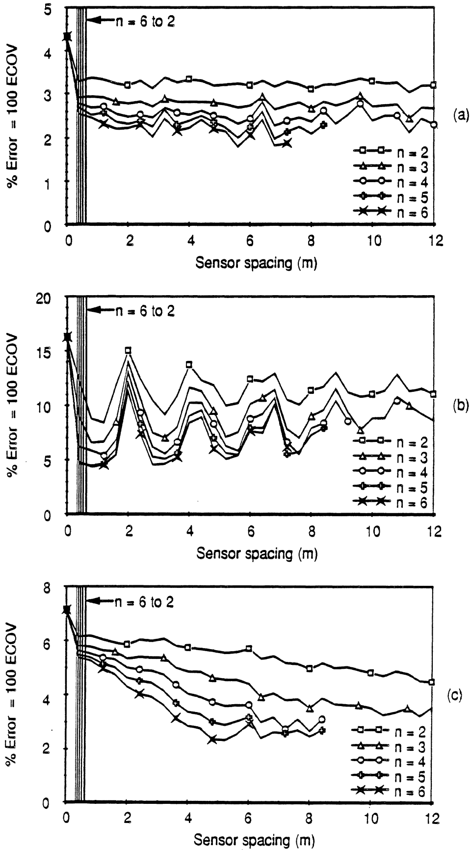
Fig. 5.30 WIM array error vs sensor spacing Vehicle S4, Speed = 3.1 m/s (11 km/h) (a) Axle 1 (b) Axle 3 (c) Axle 5
