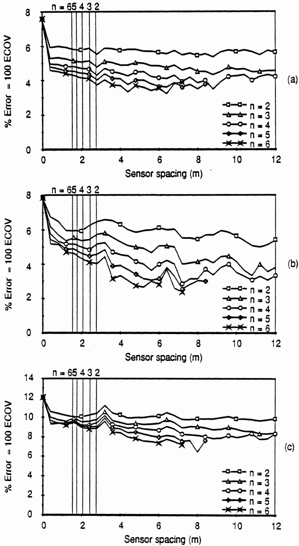
Fig. 5.21 WIM array error vs sensor spacing Vehicle S2, Speed = 13.8 m/s (50 km/h) (a) Axle 1 (b) Axle 3 (c) Axle 5
