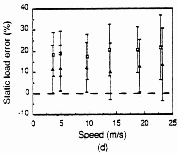
Fig. 3.6 Static load error vs speed, Vehicle S5 (a) Axle 1 (b) Axle 2 (c) Axle 3 (d) Axle 4 (e) Axle 5 Error bars indicate \pm 1 standard deviation
