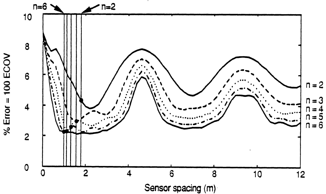
Fig. 5.4 Theoretical WIM array Error Coefficient of Variation \rho vs sensor spacing \Delta '1/4-car' model (natural frequency = 1.9 Hz), speed = 32 km/h. Vertical lines denote design spacings according to eq 4.22.
