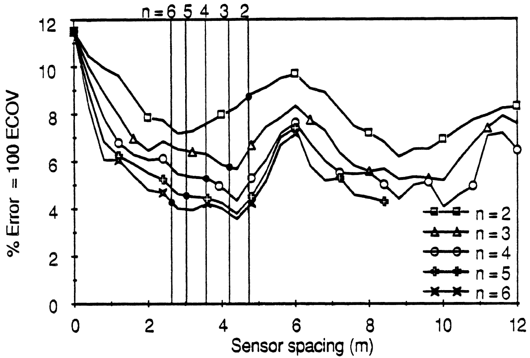
Fig. 5.7 Experimental WIM Error Coefficient of Variation p vs sensor spacing \Delta , vehicle S4, speed 85 km/h, axle 5 (on trailer). Vertical lines denote design spacings according to eq 4.22.
