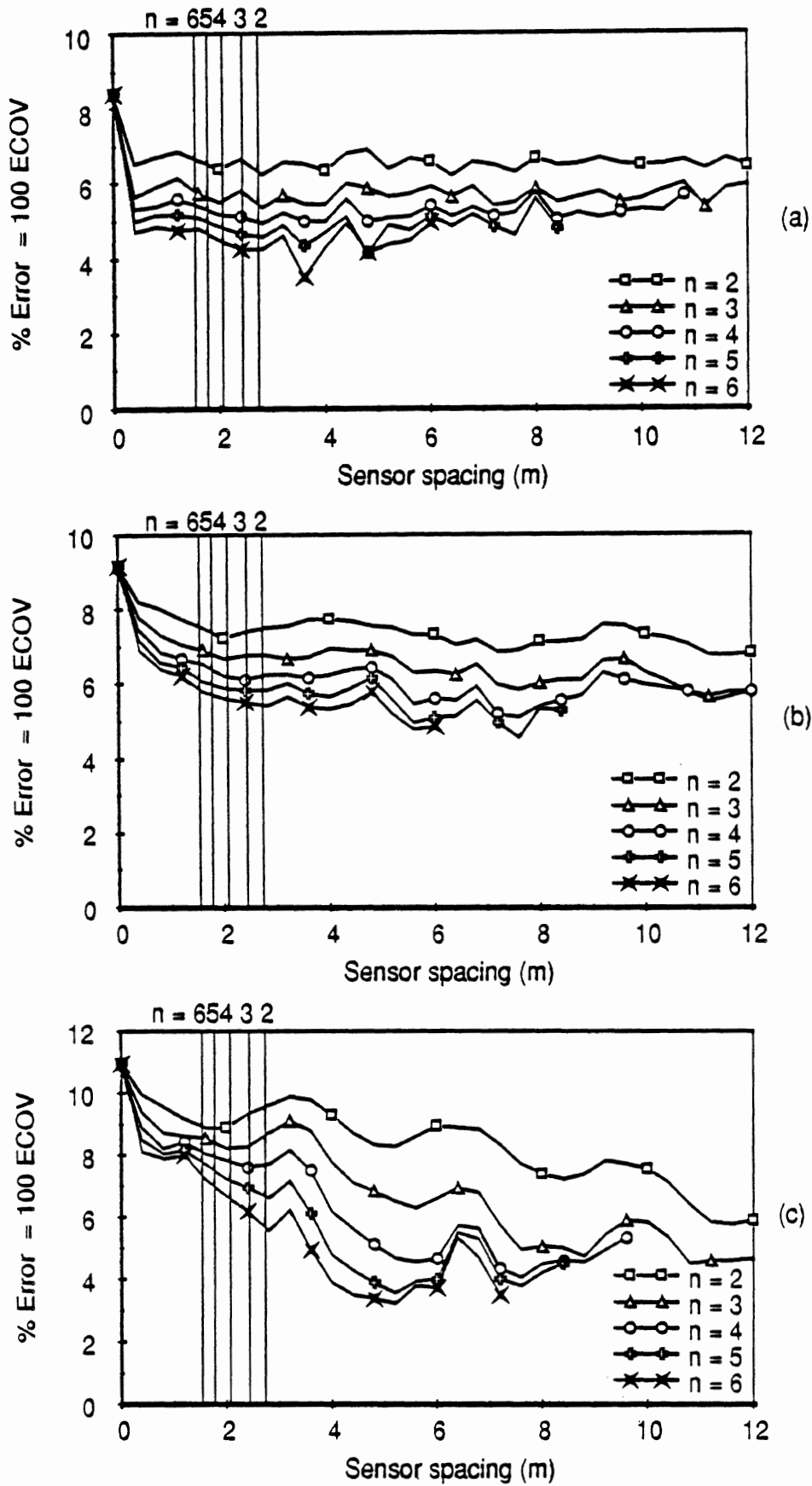
Fig. 5.39 WIM array error vs sensor spacing Vehicle S5, Speed = 13.7 m/s (49 km/h) (a) Axle 1 (b) Axle 3 (c) Axle 5
