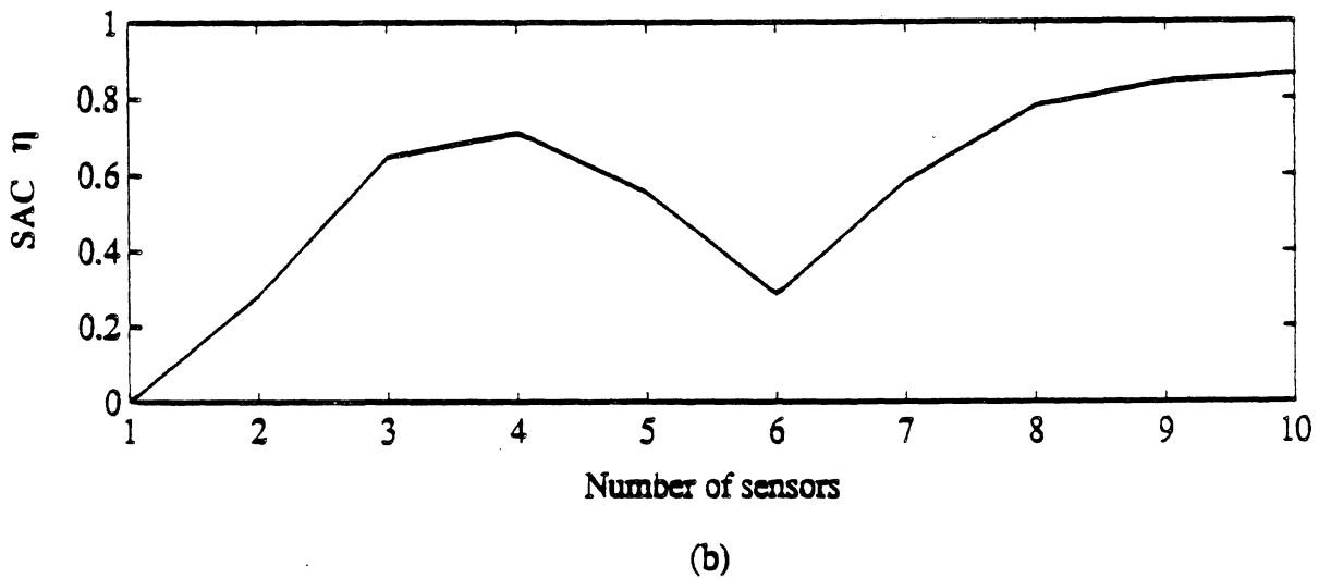
Fig 4.13 Variation of WIM system performance for vehicle model 2 with the number of sensors in the array. The sensors are spaced according to eq. 4.22 with \bar{f}=2.5 Hz and the vehicle is travelling at the array design speed of 80 km/h. (a) Error Coefficient of Variation \rho , (b) Static Accuracy Coefficient \eta .
