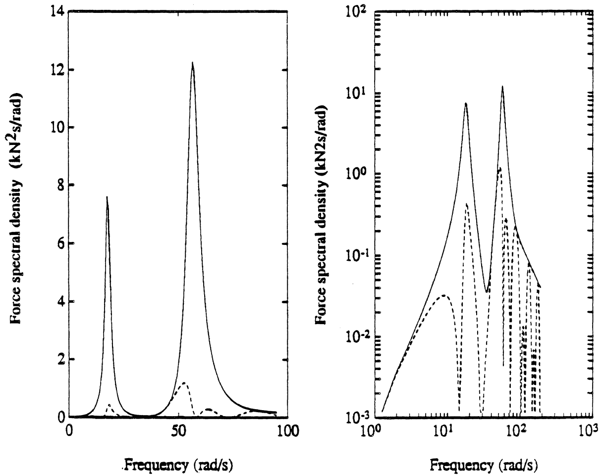
Fig 4.11 Leading tyre force and error spectral densities S_{pp}(\omega) and S_{ee}(\omega) for vehicle model 2 travelling at 100 km/h over a WIM array with n=3 and \Delta = 5 m. — = S_{pp}(\omega) , - - - = S_{ee}(\omega) .
