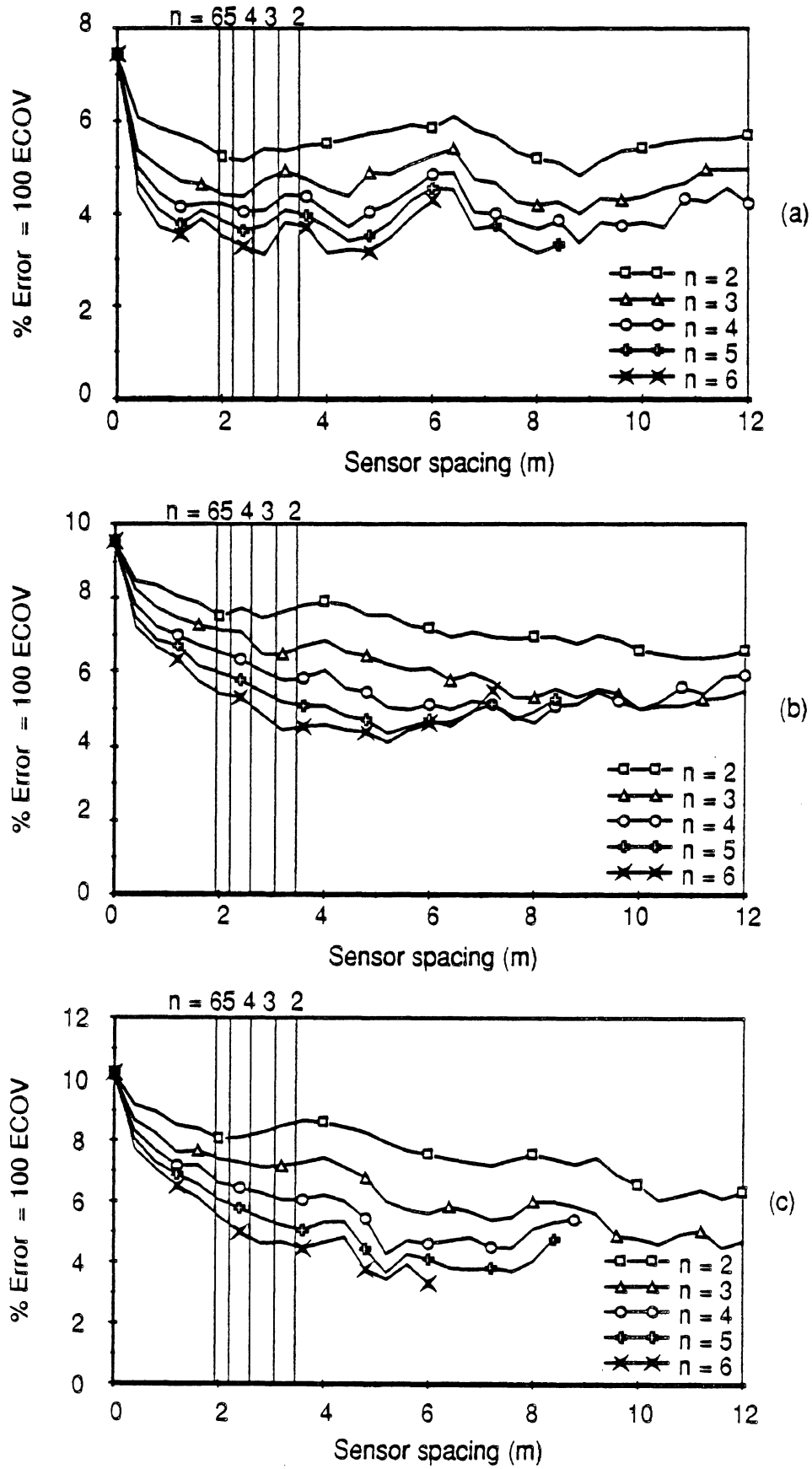
Fig. 5.46 WIM array error vs sensor spacing Vehicle S6, Speed = 17.3 m/s (62 km/h) (a) Axle 1 (b) Axle 3 (c) Axle 5
