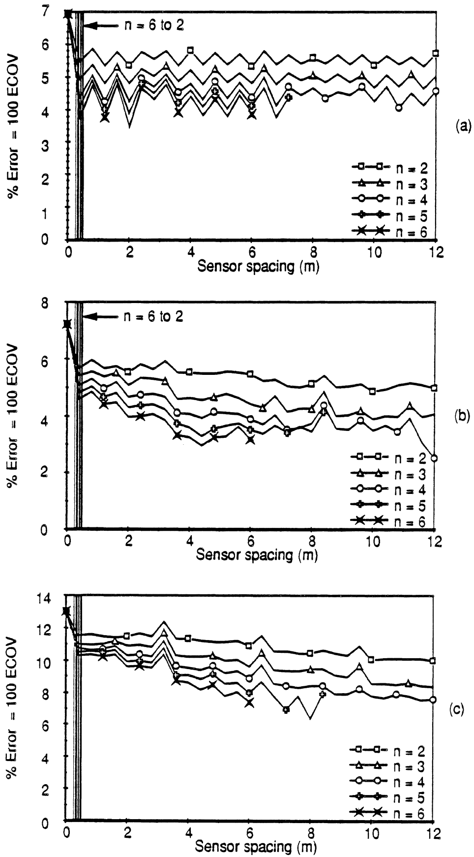
Fig. 5.12 WIM array error vs sensor spacing Vehicle S1, Speed = 2.5 m/s (9 km/h) (a) Axle 1 (b) Axle 3 (c) Axle 5
