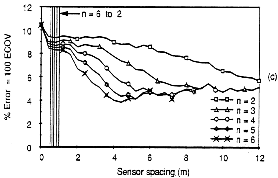
Fig. 5.37 WIM array error vs sensor spacing Vehicle S5, Speed = 4.9 m/s (18 km/h) (a) Axle 1 (b) Axle 3 (c) Axle 5
