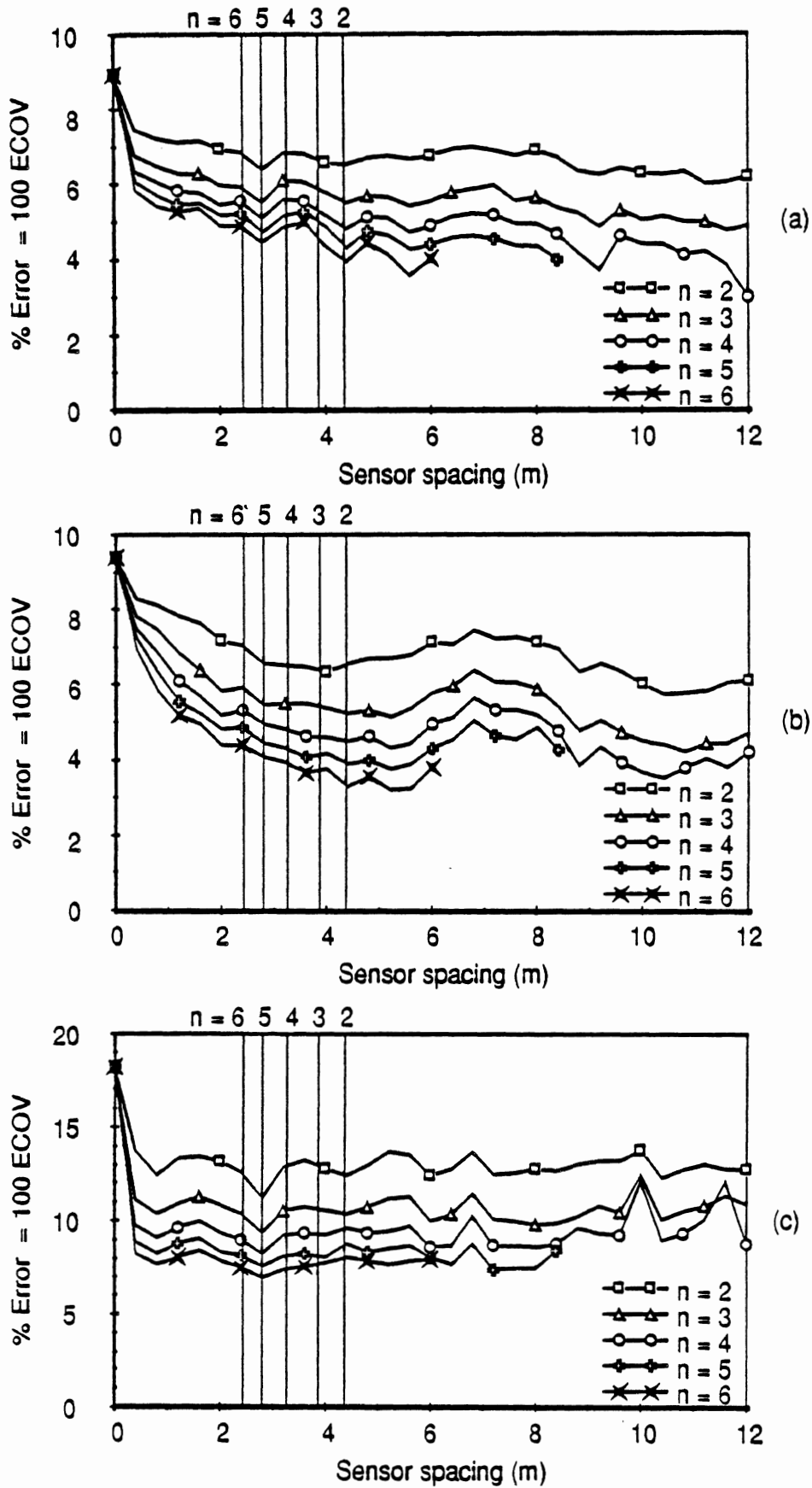
Fig. 5.29 WIM array error vs sensor spacing Vehicle S3, Speed = 21.8 m/s (78 km/h) (a) Axle 1 (b) Axle 3 (c) Axle 5
