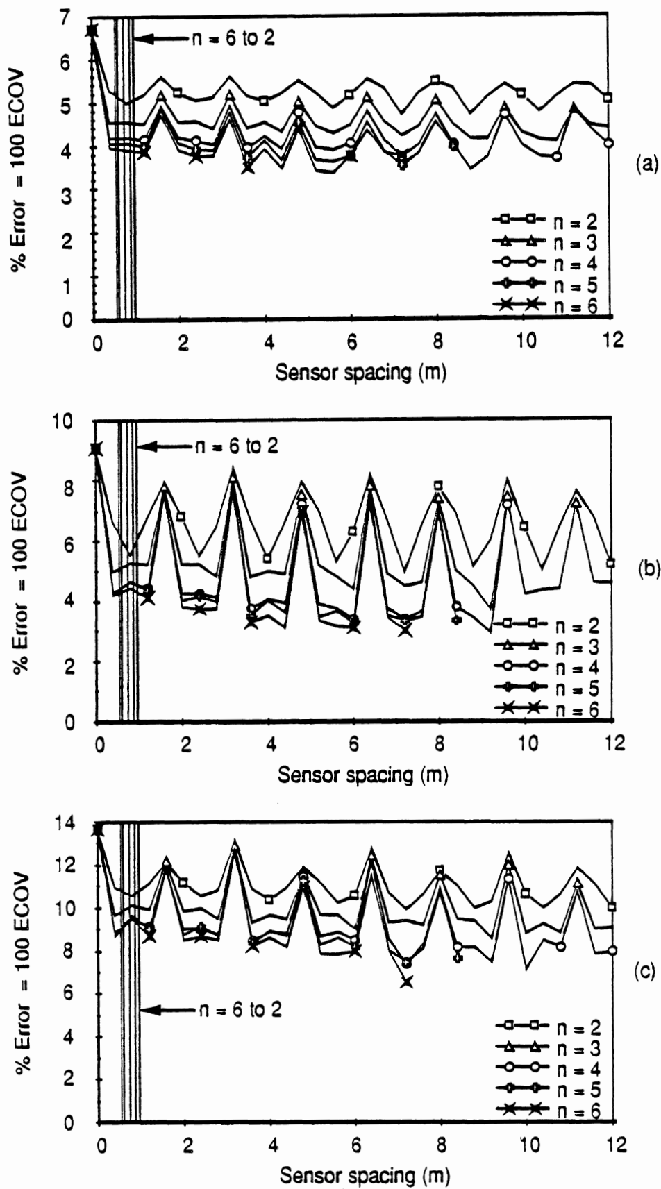
Fig. 5.19 WIM array error vs sensor spacing Vehicle S2, Speed = 4.8 m/s (17 km/h) (a) Axle 1 (b) Axle 3 (c) Axle 5
