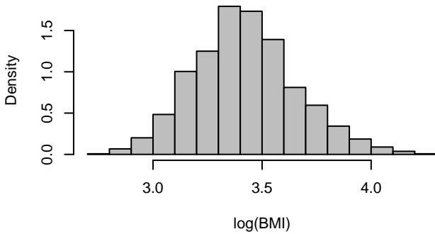
Histogram of Log(BMI)
