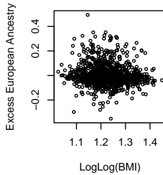
Scatter Plot of Excess European Ancestry at D15S652 and LogLog(BMI)
