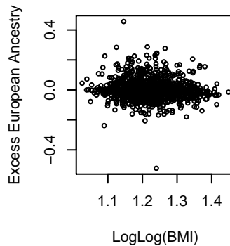
Scatter Plot of Excess European Ancestry at D15S816 and LogLog(BMI)
