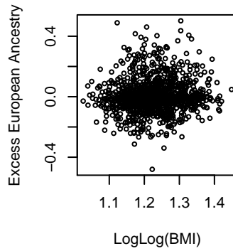
Scatter Plot of Excess European Ancestry at D3S1311 and LogLog(BMI)
