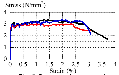
Fig. 5 Stress-strain curves of 3-day age ECC
