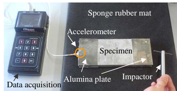
Fig. 2 Resonant frequency test
