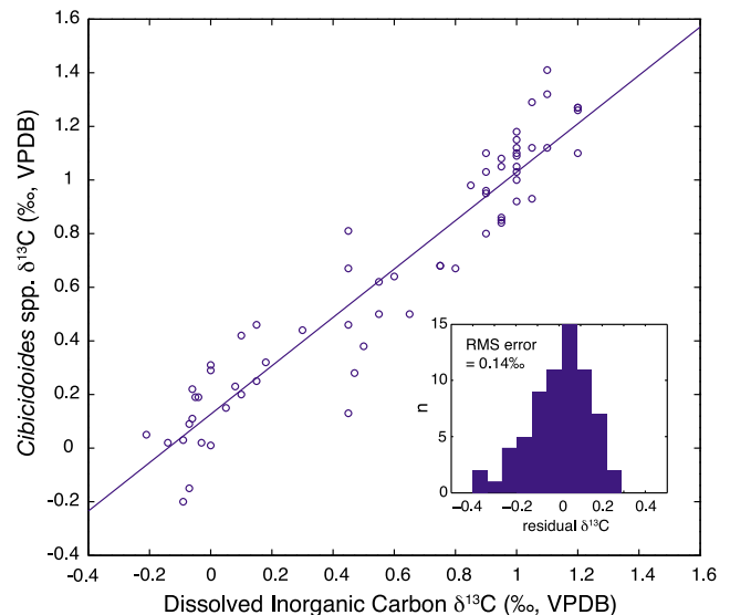
Figure 12. Scatterplot of dissolved inorganic carbon \delta^{13}\text{C} versus Holocene Cibicidoides \delta^{13}\text{C} data from Duplessy et al. [1984]. We estimate an RMS error of 0.14\text{‰} for the regression between the two parameters. Inset shows a histogram of residual values (i.e., foraminiferal \delta^{13}\text{C} values predicted by the regression minus observed foraminiferal \delta^{13}\text{C} ).
