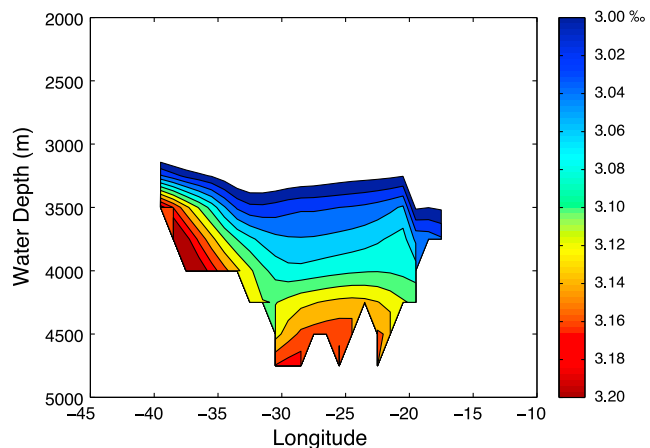
Figure 8. Contoured cross section of \delta^{18}\text{O} at 27.5^\circ\text{S} in the southwest Atlantic. The \delta^{18}\text{O} values are contoured in 0.02\text{‰} increments from 3.00 to 3.20‰. We calculated \Delta\delta^{18}\text{O} by subtracting the \delta^{18}\text{O} values nearest the seafloor from 3.08‰. \Delta\delta^{18}\text{O} is larger if the calculation is limited to the western boundary, where the majority of tracer fluxes into our control volume (see text for details).
