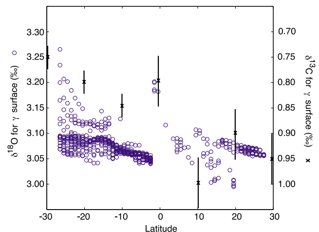
Figure 16. Plot of \delta^{18}\text{O} (circles) and \delta^{13}\text{C} (crosses) versus latitude along the neutral density surface \gamma = 28.15 . To estimate the \delta^{13}\text{C} values, we determined the approximate depth of \gamma = 28.15 in each latitude bin of Figure 11 and used the \delta^{13}\text{C} at that water depth. We estimate an along isopycnal gradient of 5 \times 10^{-8} \text{‰ m}^{-1} for \delta^{13}\text{C} , approximately twice the horizontal gradient for \delta^{18}\text{O} .
