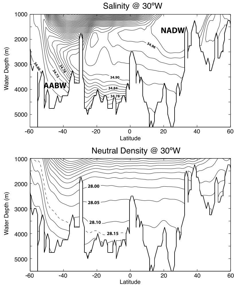
Figure 4. (top) Salinity section along 30^\circ\text{W} in the Atlantic Ocean. The contour interval is 0.02 salinity units. The largest vertical gradient in salinity in the deep Atlantic between 30^\circ\text{S} and the equator exists from 3800 to 4300 m water depth, the approximate location of the upper boundary for AABW. (bottom) Neutral density section along 30^\circ\text{W} in the Atlantic Ocean. The maximum vertical salinity gradient corresponds to a neutral density surface \gamma = 28.15 \text{ kg/m}^3 (dashed line), which also marks the maximum overturning stream function for the South Atlantic [Lumpkin and Speer, 2007]. Salinity and neutral density data are from the WOCE Global Hydrographic Climatology [Gouretski and Koltermann, 2004].
