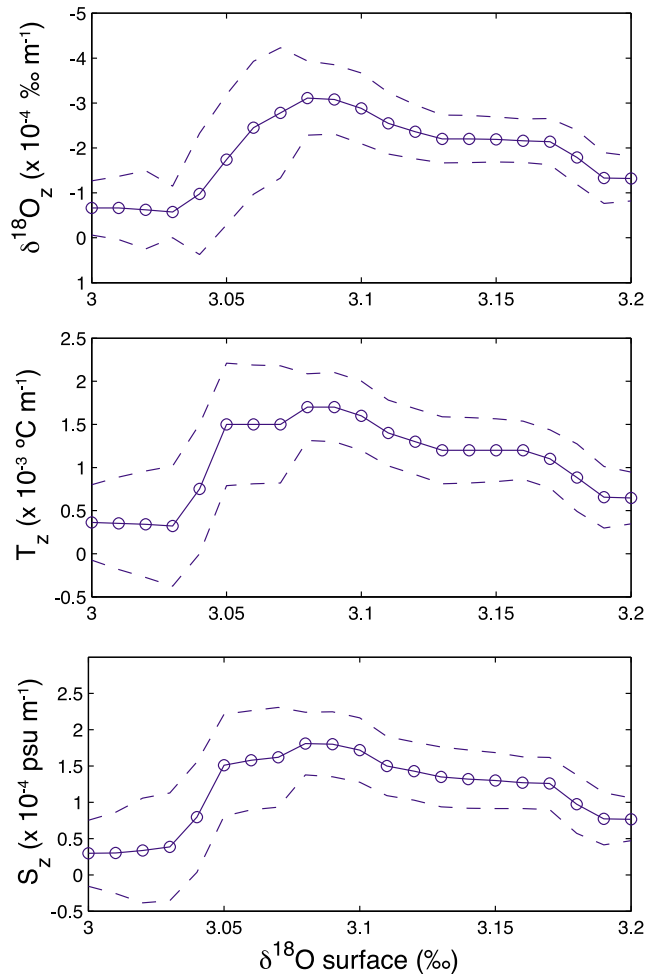
Figure 6. (top) The vertical gradient in \delta^{18}\text{O} , (middle) potential temperature, and (bottom) salinity across \delta^{18}\text{O} isosurfaces ranging from 3.00‰ to 3.20‰. One-sigma standard deviations are given as dashed lines. Temperature and salinity data are from the WOCE Global Hydrographic Climatology [Gouretski and Koltermann, 2004]. The maximum \delta^{18}\text{O}_z occurs between \delta^{18}\text{O} values of 3.06‰ and 3.11‰.
