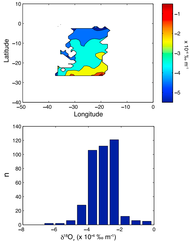
Figure 7. (top) Contour map of the vertical \delta^{18}\text{O} gradient ( \delta^{18}\text{O}_z ) at \delta^{18}\text{O} = 3.08\text{‰} . This \delta^{18}\text{O} surface spans the southwestern Atlantic. (bottom) Histogram of \delta^{18}\text{O}_z values along the \delta^{18}\text{O} = 3.08\text{‰} surface in the southwestern Atlantic. The mean \delta^{18}\text{O}_z value for this \delta^{18}\text{O} surface is -3.1 \times 10^{-4} \text{‰ m}^{-1} .
