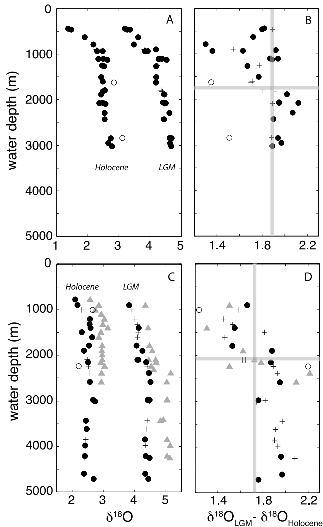
Figure 2. (a) Brazil Margin Cibicidoides spp. \delta^{18}\text{O} (solid circles) [Curry and Oppo, 2005], outliers (open circles), and interpolated data points (crosses). Outliers are defined as those values which exceed the mean \delta^{18}\text{O} from adjacent water depths by more than \pm 0.3\% . Interpolated values are based on linear interpolation between data points at adjacent water depths. (b) Brazil Margin LGM-Holocene \delta^{18}\text{O} . (c) Blake Ridge Cibicidoides spp. \delta^{18}\text{O} (solid circles) [Keigwin, 2004], outliers (open circles), and interpolated data points (crosses). Also included are Uvigerina spp. \delta^{18}\text{O} (gray triangles) [Keigwin, 2004]. (d) Blake Ridge LGM-Holocene \delta^{18}\text{O} . Using a Student t test and assuming a threshold two-sided p value of 0.05, we are able to reject the null hypothesis that the shallow and deep LGM-Holocene \delta^{18}\text{O} data are sampled from the same population ( p \approx 0.005 for Brazil Margin Cibicidoides sp., p \approx 0.0005 for Blake Ridge Cibicidoides sp., and p \approx 0.02 for Blake Ridge Uvigerina sp.). This result is not surprising given that LGM-Holocene \delta^{18}\text{O} data above 2 km fall in the upper left-hand quadrant of each plot, while the deeper data fall in the lower right-hand quadrant.
