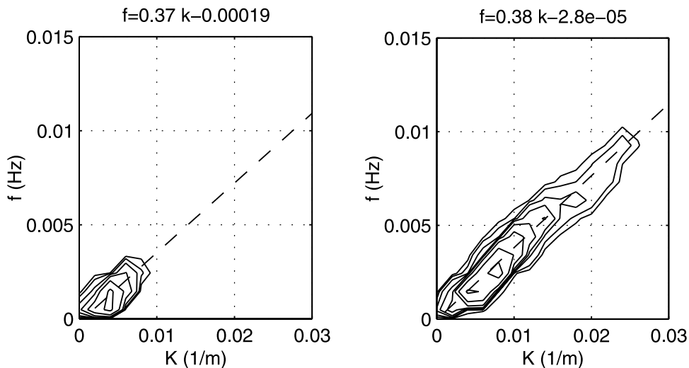
Figure 8. Frequency-longshore wavenumber spectra for c_f = 0.007 for shoreline runup computed while (left) neglecting and (right) including wave-current interaction. Contour levels plotted are (10, 20, 40, 80, 160, 320, 640, 1280). The equation for the best-fit dispersion line (dashed line) is noted above each plot.
