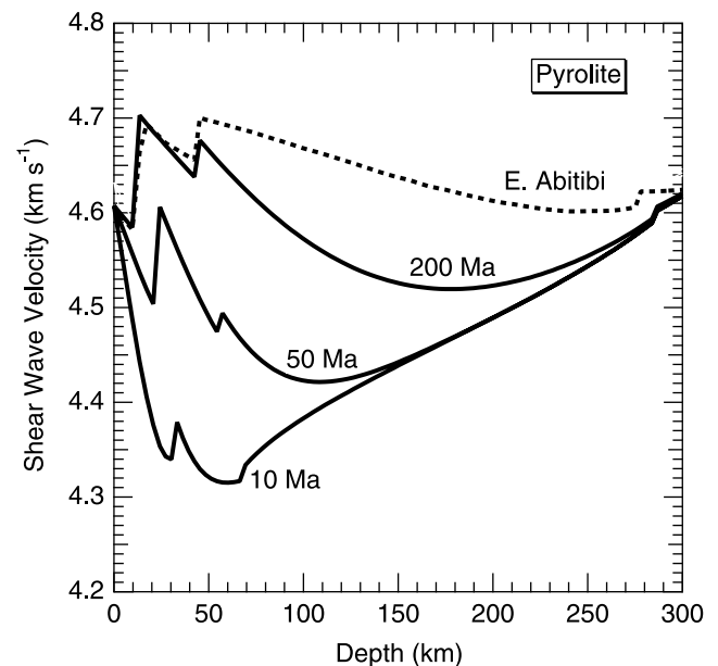
Figure 7. Influence of lithospheric age on the shear wave velocity. Velocity along a continental geotherm (dashed) is shown for comparison.
