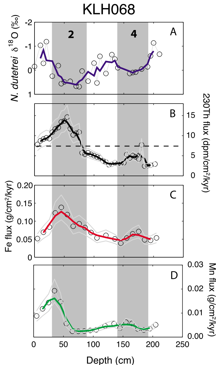
Figure 10. Flux data for core K LH068. (a) Oxygen isotope stratigraphy, (b) ^{230}\text{Th} flux ( \text{dpm}/\text{cm}^2/\text{kyr} ), (c) Fe flux ( \text{g}/\text{cm}^2/\text{kyr} ), and (d) Mn flux ( \text{g}/\text{cm}^2/\text{kyr} ). Colored lines are 3-point running mean values. The expected ^{230}\text{Th} flux for this water depth is approximately 7.5 \text{ dpm}/\text{cm}^2/\text{kyr} (dashed horizontal line). All flux calculations are based on ages inferred from the oxygen isotope stratigraphy. We assume a conservative error of \pm 30\% for the age difference between successive points. This uncertainty dwarfs the errors in dry bulk density, weight percent, and \text{dpm}/\text{g} reported by Frank et al. [1994] and is therefore the primary contributor to the one-sigma flux errors (gray lines). Age model error of a factor or two or larger would be necessary to eliminate the flux maxima at the MIS 2–1 boundary.
