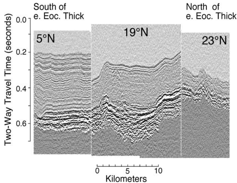
Figure 3. Example seismic sections taken along the 56 Ma transect near the northern and southern extremes of the transect and near the thicker part of the section ( 19^{\circ}\text{N} ). Dark shading indicates acoustic basement. Unshaded intervals indicate the high-amplitude reflection package lying on acoustic basement and taken to represent the lower Eocene calcareous section. Lighter shaded intervals indicate the overlying Cenozoic clays and siliceous-calcareous oozes. Modern latitude of each section is shown at the top of each section. Vertical scale is in milliseconds two-way travel time. Sections have been shifted vertically to achieve a seismic character match of two prominent high-amplitude, continuous reflections.
