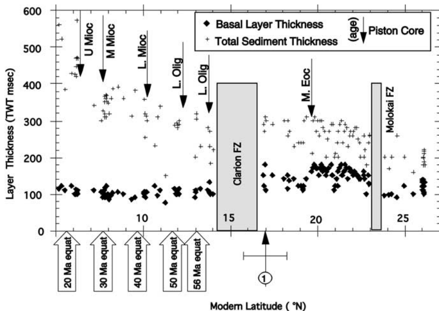
Figure 2. Total sediment thickness (plus signs) and thickness of the basal package of high-amplitude seismic reflections (diamonds) lying over 56 Ma oceanic crust plotted versus modern latitude. Offsets in the transect at fracture zones (Figure 1) are shown as shaded rectangles. Thicknesses are measured in two-way travel time (TWTT). Locations of the paleo-equator as determined by plate rotations [Engerbretson et al. , 1985; Gripp and Gordon, 1990] are indicated below the latitude axis for various times in Cenozoic. A vertical upward arrow with crossbar indicates the estimated position (with error bar) of the 56 Ma equator after correction for hot spot motion (see text). Vertical downward arrows indicate the age and location of the oldest sediments recovered in piston cores taken along the transect.
