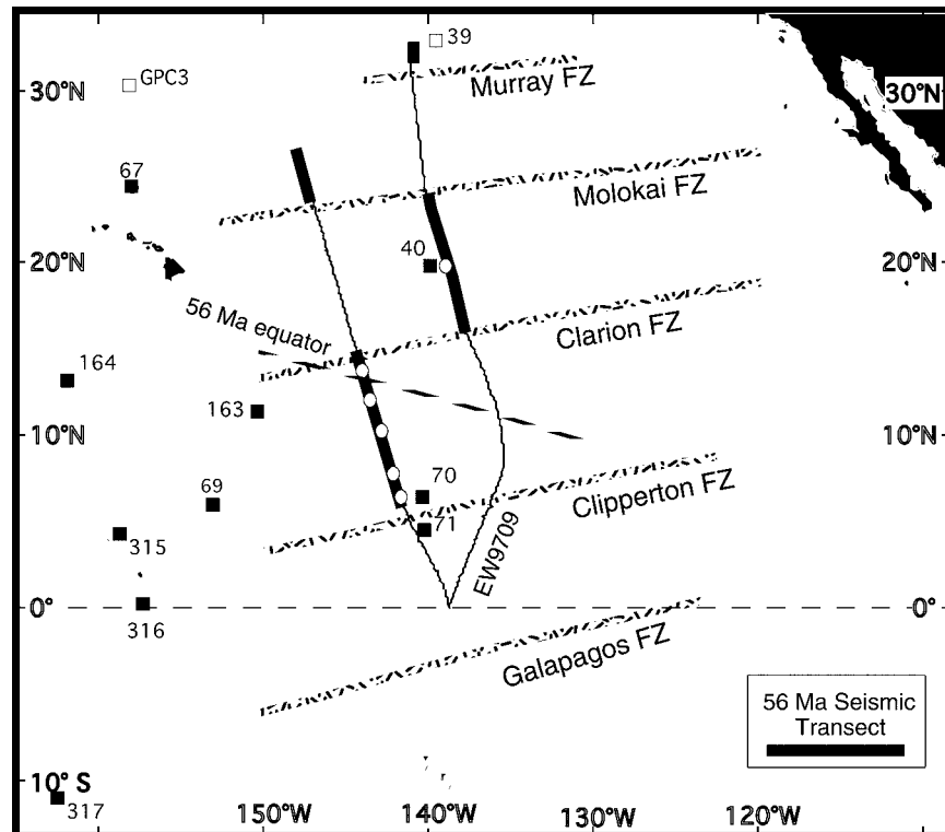
Figure 1. The track of the R/V Maurice Ewing (cruise EW9709). Thick solid lines indicate that part of the survey that is along 56 Ma ocean crust. Oceanic fracture zones (FZ), indicated by broad dotted lines, offset the ridge crest and produce offsets in the age of the crust. A thinner hatched line indicates the position of the 56 Ma paleoequator using the fixed hot spot rotation scheme used in this paper [Engerbreitson et al. , 1985; Gripp and Gordon, 1990]. Open circles indicate locations of the cores shown in Figure 2. Solid squares and associated numbers indicate DSDP sites containing middle to lower Eocene siliceous oozes and cherts. Open squares indicate DSDP sites and Giant Piston Core 3 containing no middle to lower Eocene siliceous oozes and cherts.
