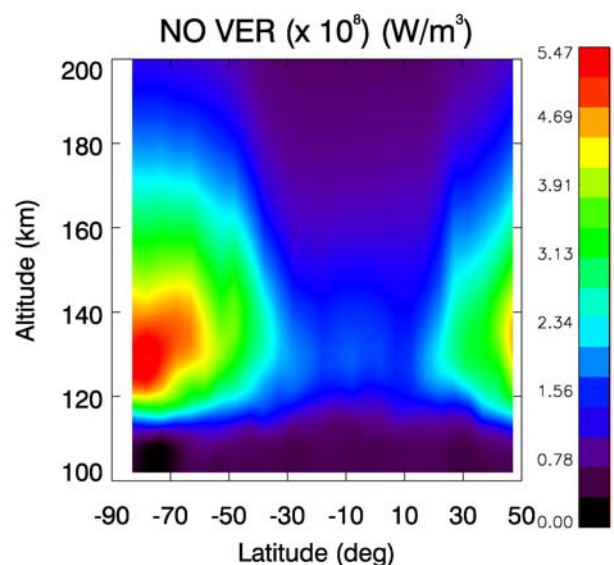
Figure 3. The zonal mean volume emission rate (VER, \text{W/m}^3 ) at 5.3 \mu\text{m} from NO on April 18 during the solar storm. Note the change of scale from Figure 2.
