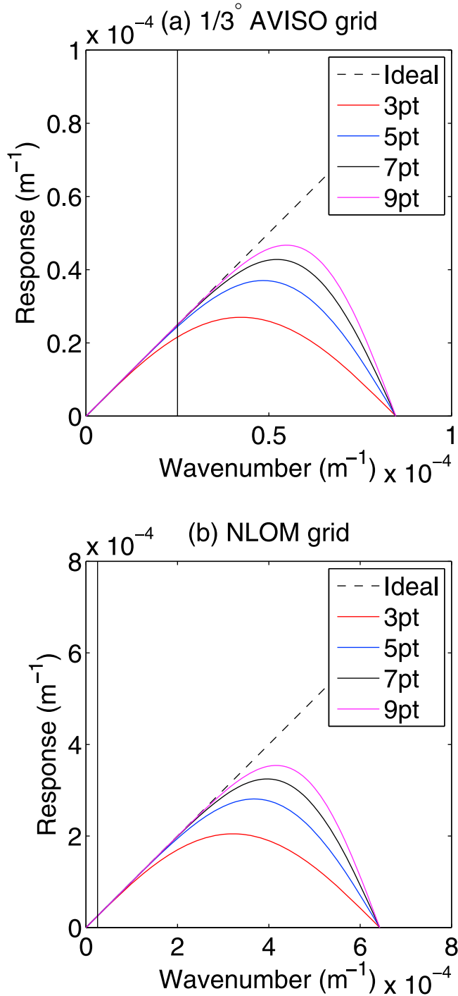
Figure 2. Response of an ideal differentiator and of 3-, 5-, 7-, and 9-point stencils, as a function of wave number, on (a) 1/3^\circ AVISO grid and (b) NLOM grid. The grid spacings used for Figures 2a and 2b are 37 and 4.9 km, respectively, and the response is the absolute value |\Lambda| of the eigenvalue of the von Neumann analysis. See text for more details. Vertical lines are drawn at the wave number (40 \text{ km})^{-1} , corresponding approximately to the 2\text{--}3^\circ wavelength resolution limitation of the AVISO sea surface height fields.
