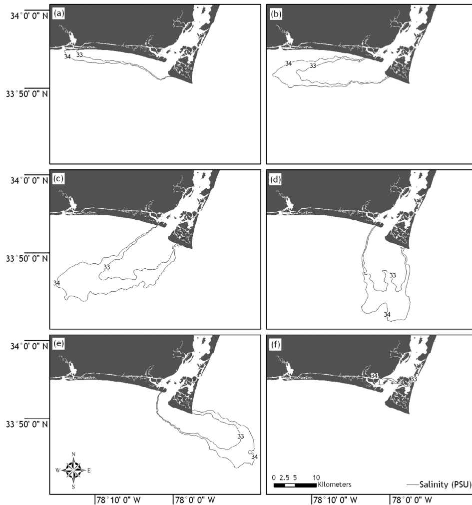
Figure 2. (a) Type I. The sea surface salinity fields forced by southerly wind with speed of 15m/s and river discharge of 1000 m 3 /s. (b) Type II. Surface salinity fields forced by wind speed of 25m/s and river discharge of 1000 m 3 /s under the response to northeasterly winds. (c) Type III. Surface salinity fields forced by wind speed of 5m/s and normal discharge under northerly winds. (d) Type IV. Surface salinity fields forced by wind speed of 5m/s and normal discharge under northwesterly winds. (e) Type V. Surface salinity fields forced by wind speed of 10m/s and river discharge of 304 m 3 /s under west winds. (f) Type VI. Plume structure under southeasterly winds and normal river discharge with a wind speed of 20 m/s. All used the results after 5 day simulation.
