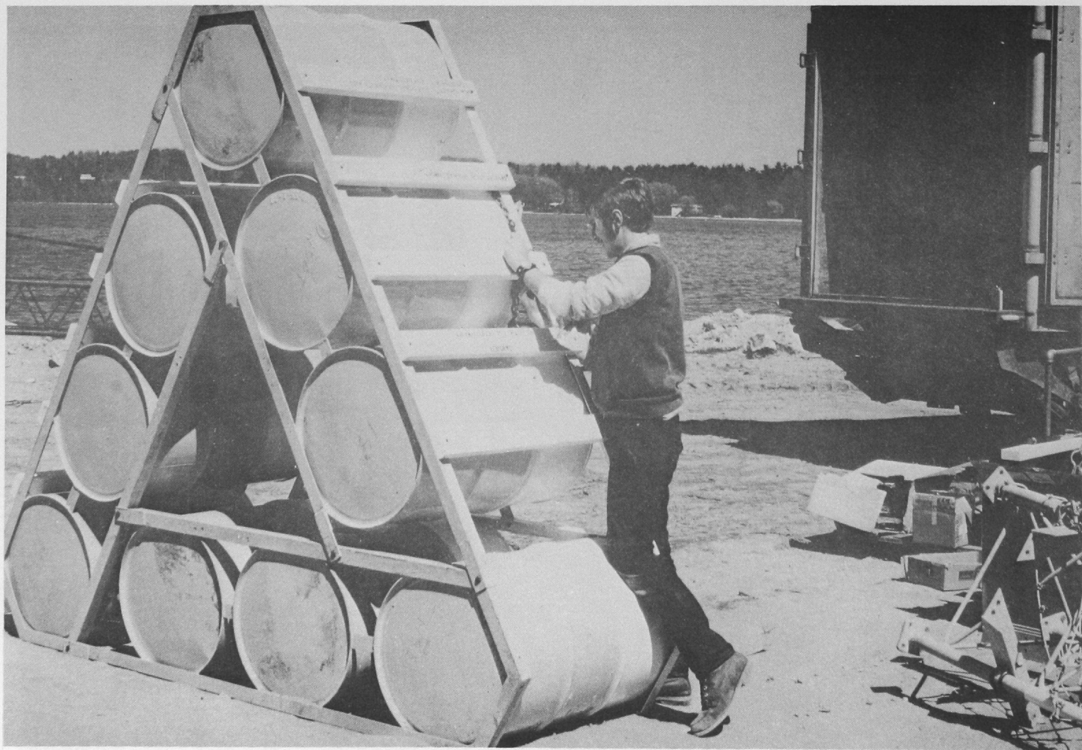
FIGURE 3 Floatation Collar
