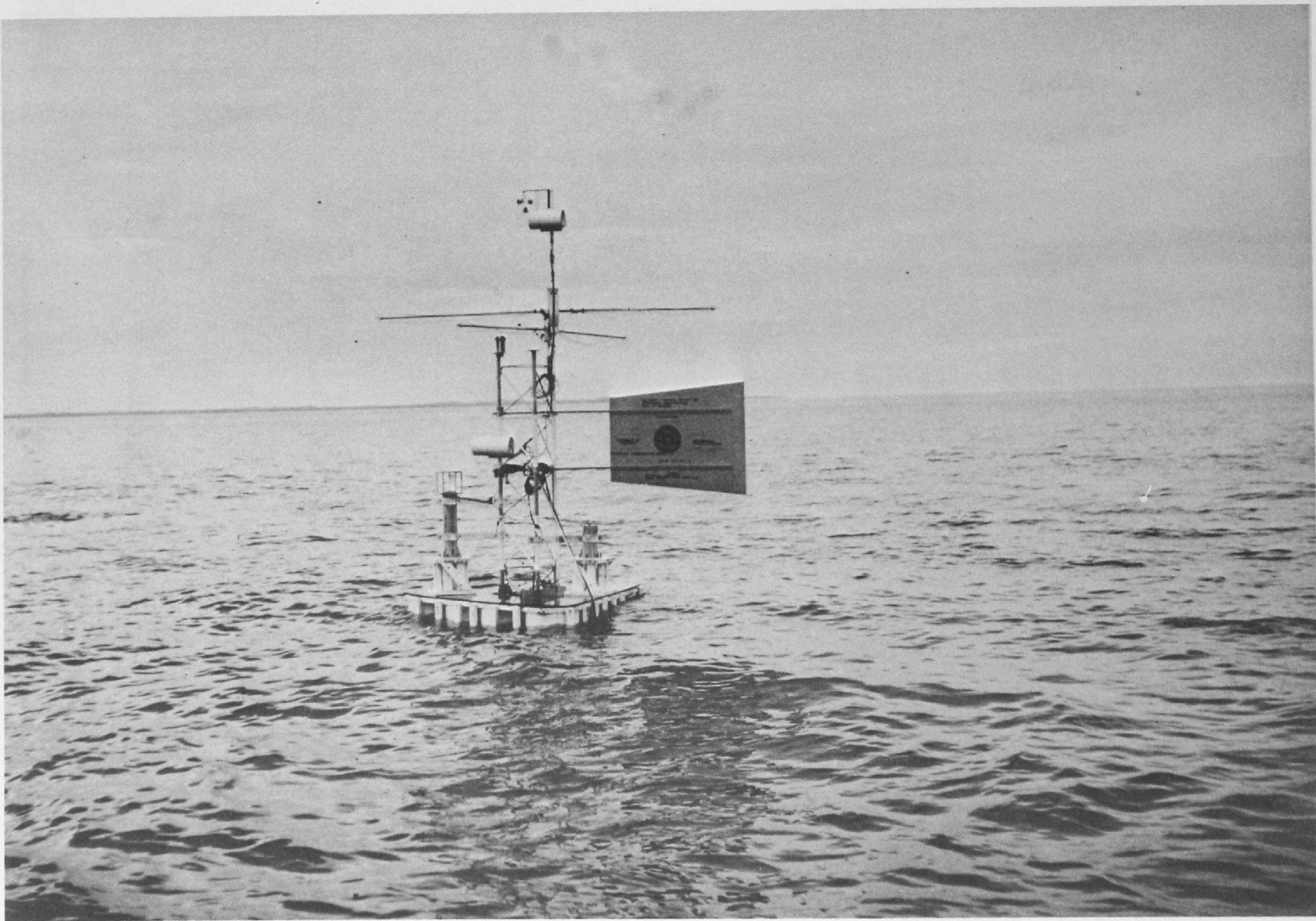
FIGURE 10 SMOP Anchored and Recording Data
