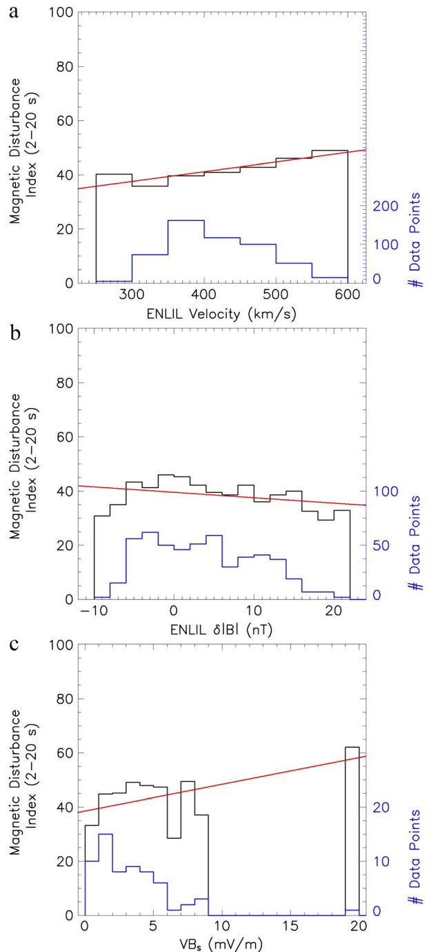
Figure 12. (a) Mean values of magnetic disturbance index (MDI) versus ENLIL-computed solar wind speed. (b) Mean MDI values versus ENLIL \delta B . (c) Mean MDI values versus hybrid VB_s (as shown in Figure 10).
