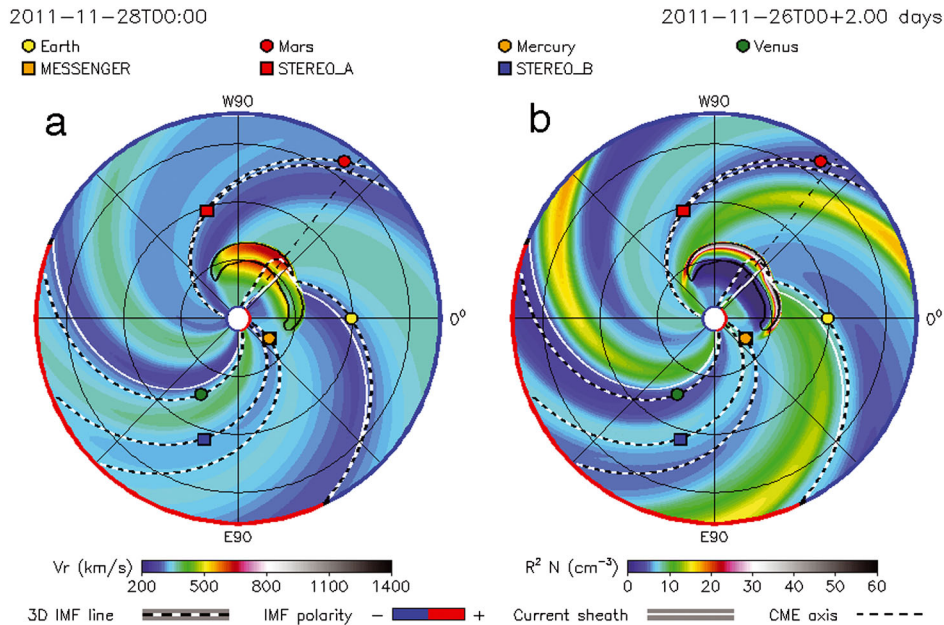
Figure 8. Model similar to that in Figure 3 but utilizing the “cone model” version of WSA-ENLIL with a propagating CME (outlined in black) as seen on 28 November 2011. (a) Solar wind speed profile. (b) Density map for the same period as Figure 8a.
