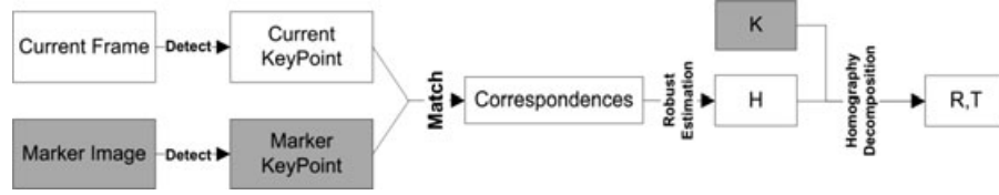
Fig. 3. Homography-from-detection algorithm framework.
