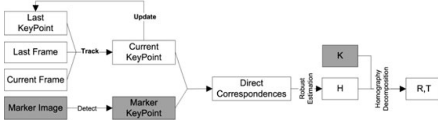
Fig. 4. Homography-from-tracking algorithm framework.
