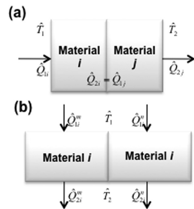
FIG. 1. (a) Heat flow for layers in series. Here, T_1 and T_2 denote the Laplace transformation of ambient temperatures on both sides of the composite; \hat{Q}_{2i(j)} and \hat{Q}_{1i(j)} are the thermal input and outflow of material i(j) . Here, \hat{Q}_{2i} = \hat{Q}_{1j} is based on the continuity of the interface heat flux between adjacent layers. (b) Heat flow for layers in parallel, where \hat{Q}_{1i}^m , \hat{Q}_{1i}^n denote input heat flux carried by two thermal dissipation modes, and \hat{Q}_{1i}^m + \hat{Q}_{1i}^n is the total heat flux into material, i .
