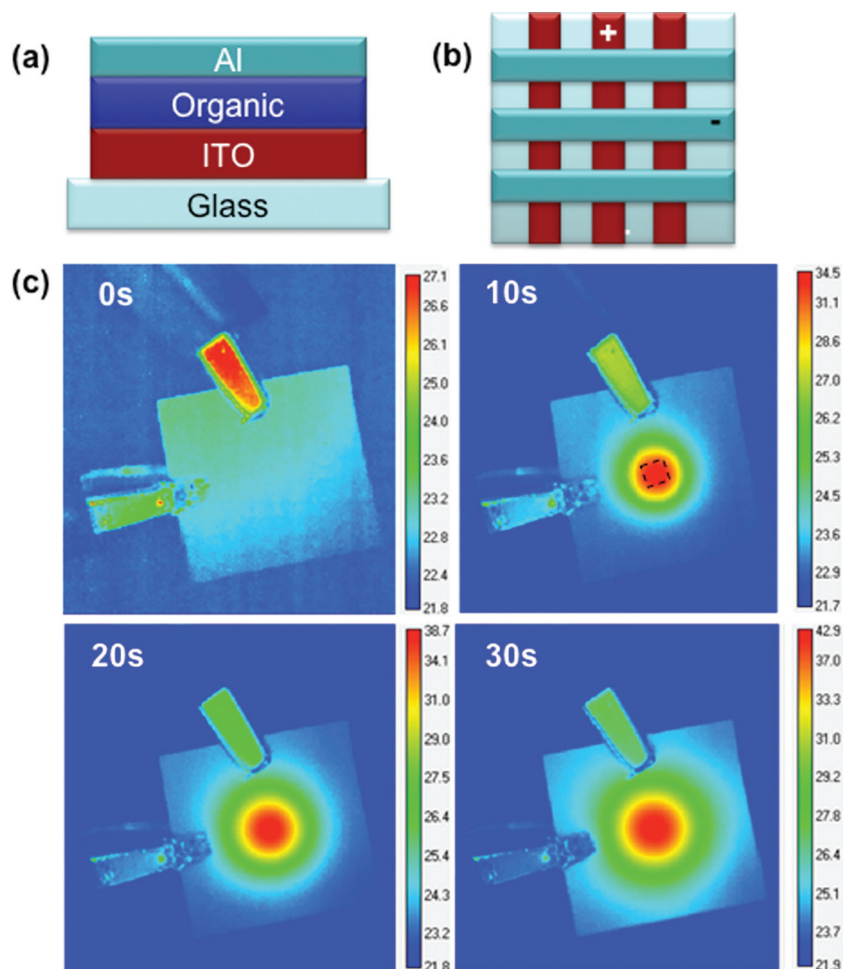
FIG. 3. (Color) (a) Schematic structure of small-area Ir(ppy) 3 devices: glass (1 mm)/ITO (120 nm)/organic layers (105 nm)/Al cathode (100 nm). (b) Patterning of the ITO and Al anode and cathode stripes, each 1 mm wide. (c) Thermal images of the Ir(ppy) 3 device under a fixed voltage of 10 V (corresponding to a current density of 1 A/cm 2 ) after 10, 20, and 30 s operation following the onset of the voltage ramp. The dashed square indicates the device location.
