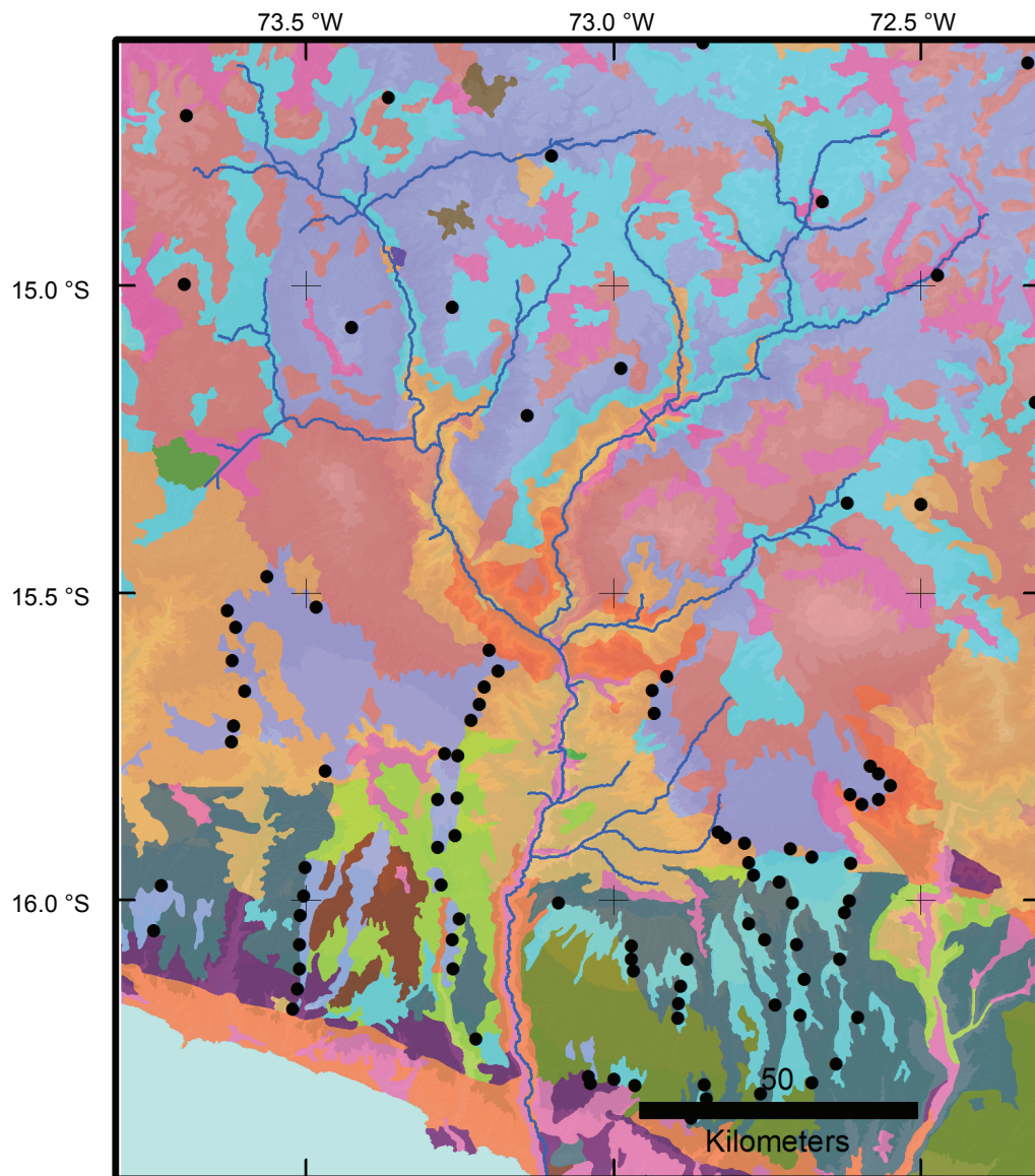
Supplementary Figure 1: Geological map used to identify 16 Ma paleosurface
