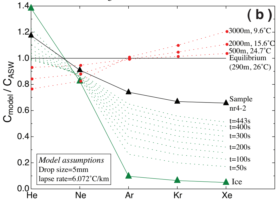
Time-dependent evolution of noble gas patterns in a raindrop assuming variable surface concentration
