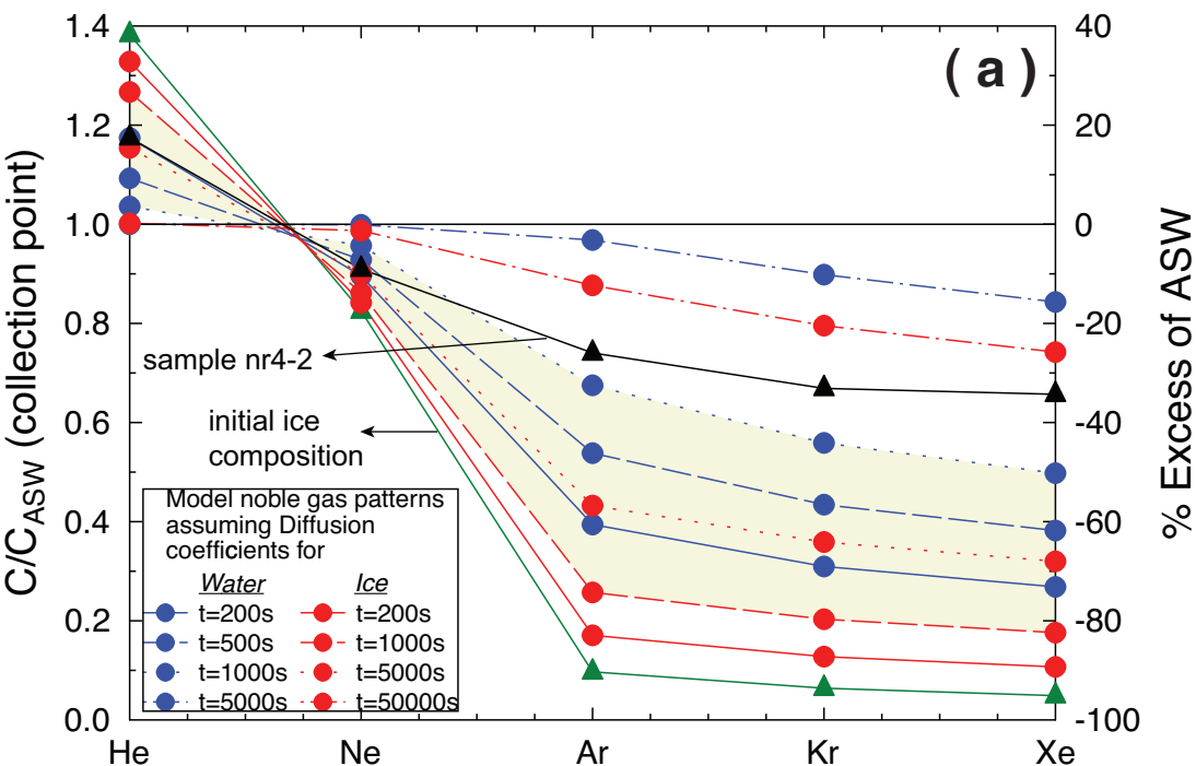
Time-dependent evolution of noble gas patterns in a raindrop assuming constant boundary condition
