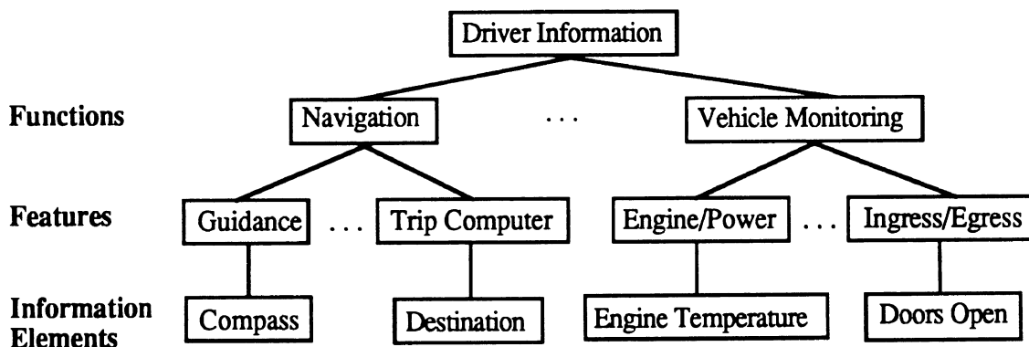
Figure 1. Driver information system terminology and organization.
