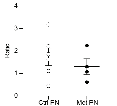
E Dam P11 BF Ratio
