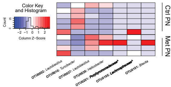
F Dam P11 Heatmap
