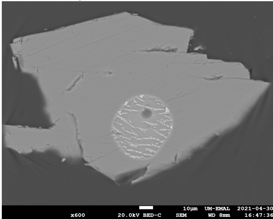
79135 OL3 olivine grain
