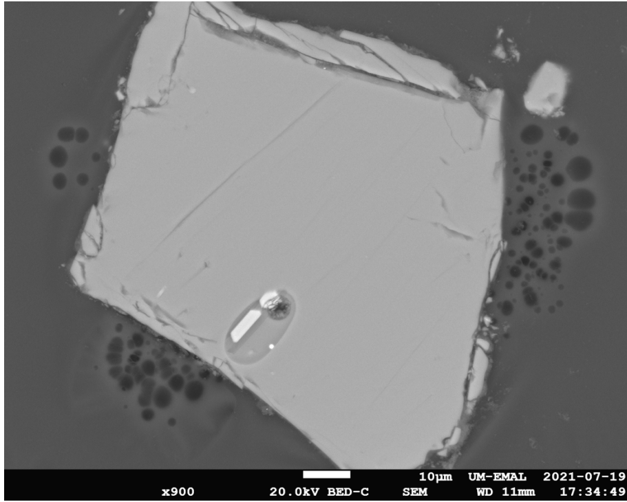
79135 OL6 olivine grain
