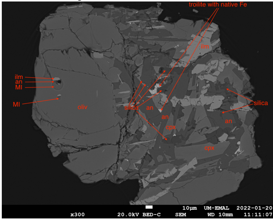
79135 OL7 olivine grain
