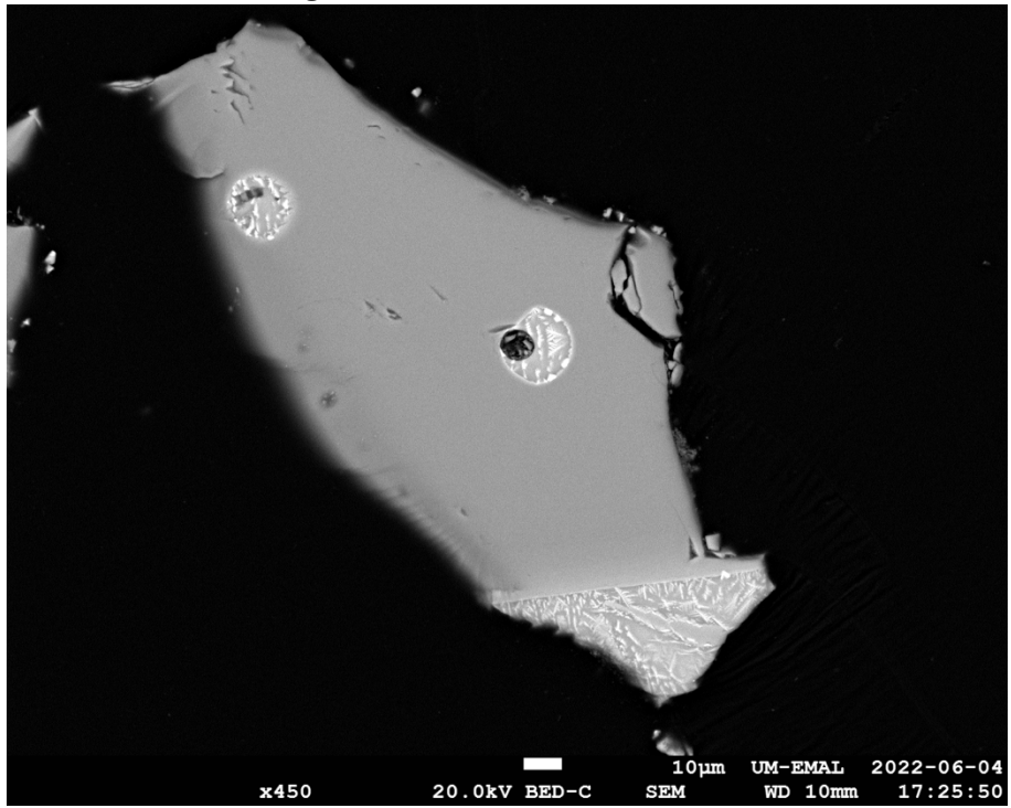
79135 OL11 olivine grain
