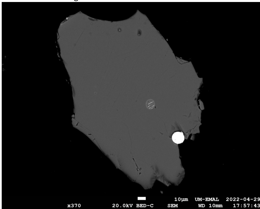
79135 OL9 olivine grain
